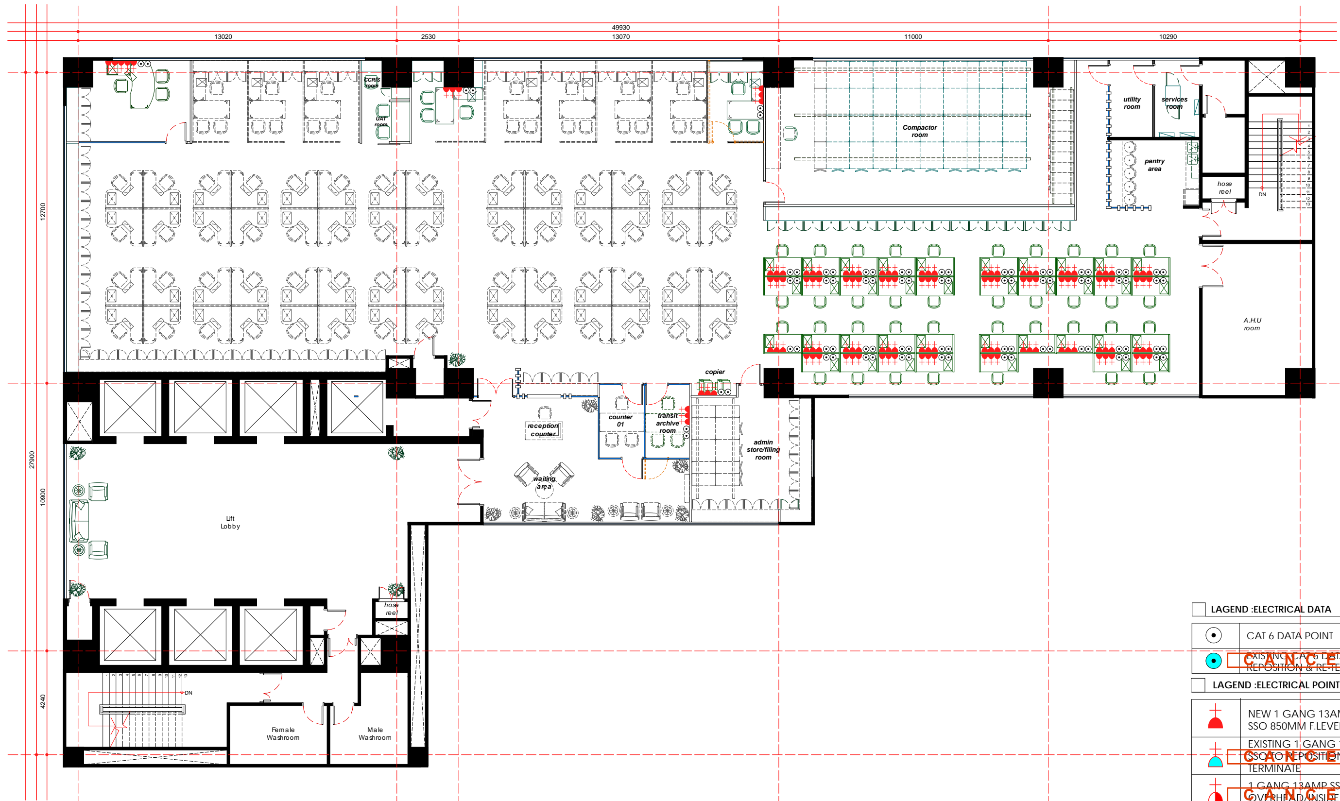
ELECTRICAL POINT LAYOUT PLAN - 05TH FLOOR SCALE 1:150 WISMA BSN
