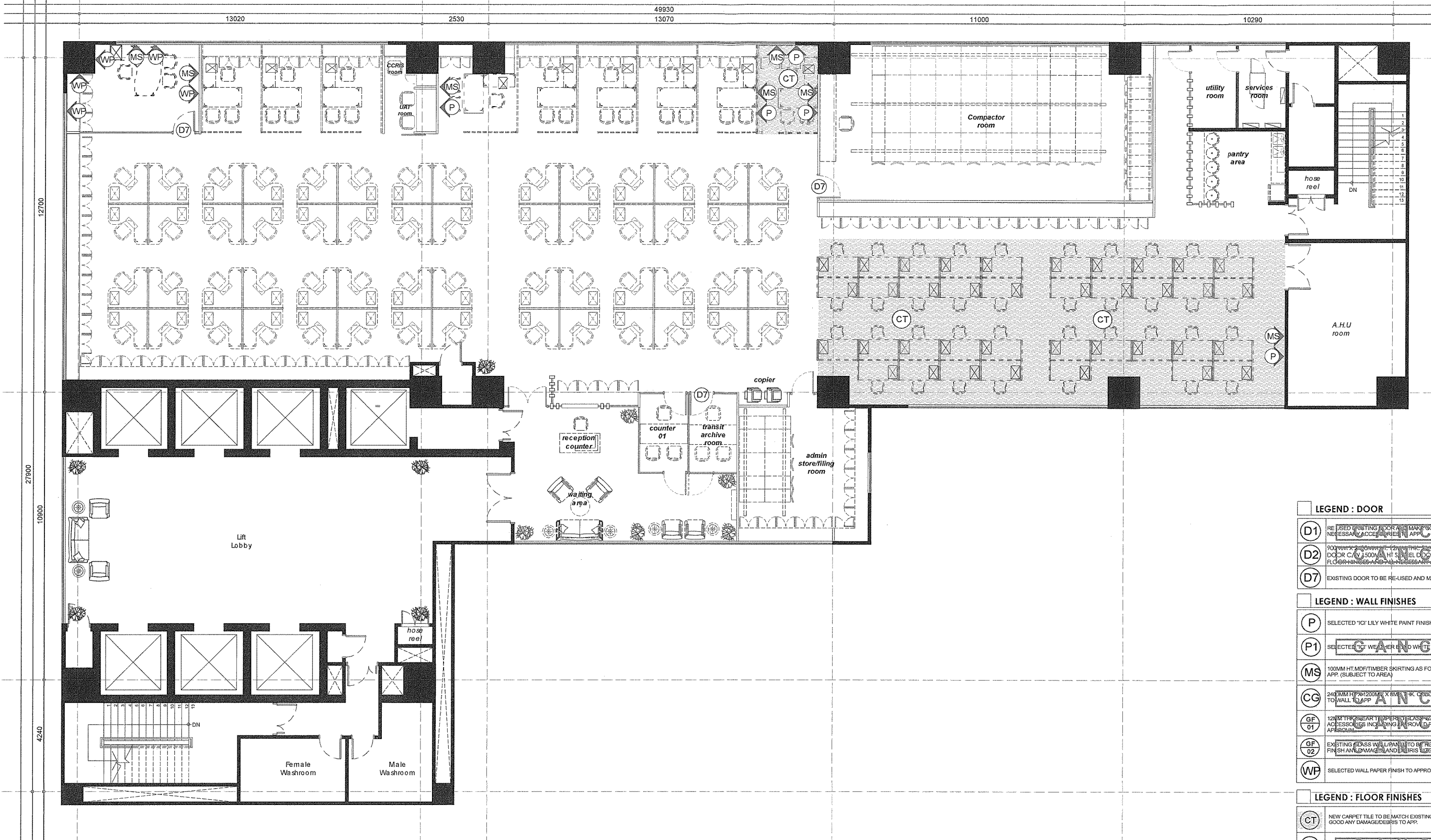
LAYOUT PLAN - 05TH FLOOR SCALE 1:150 WISMA BSN
