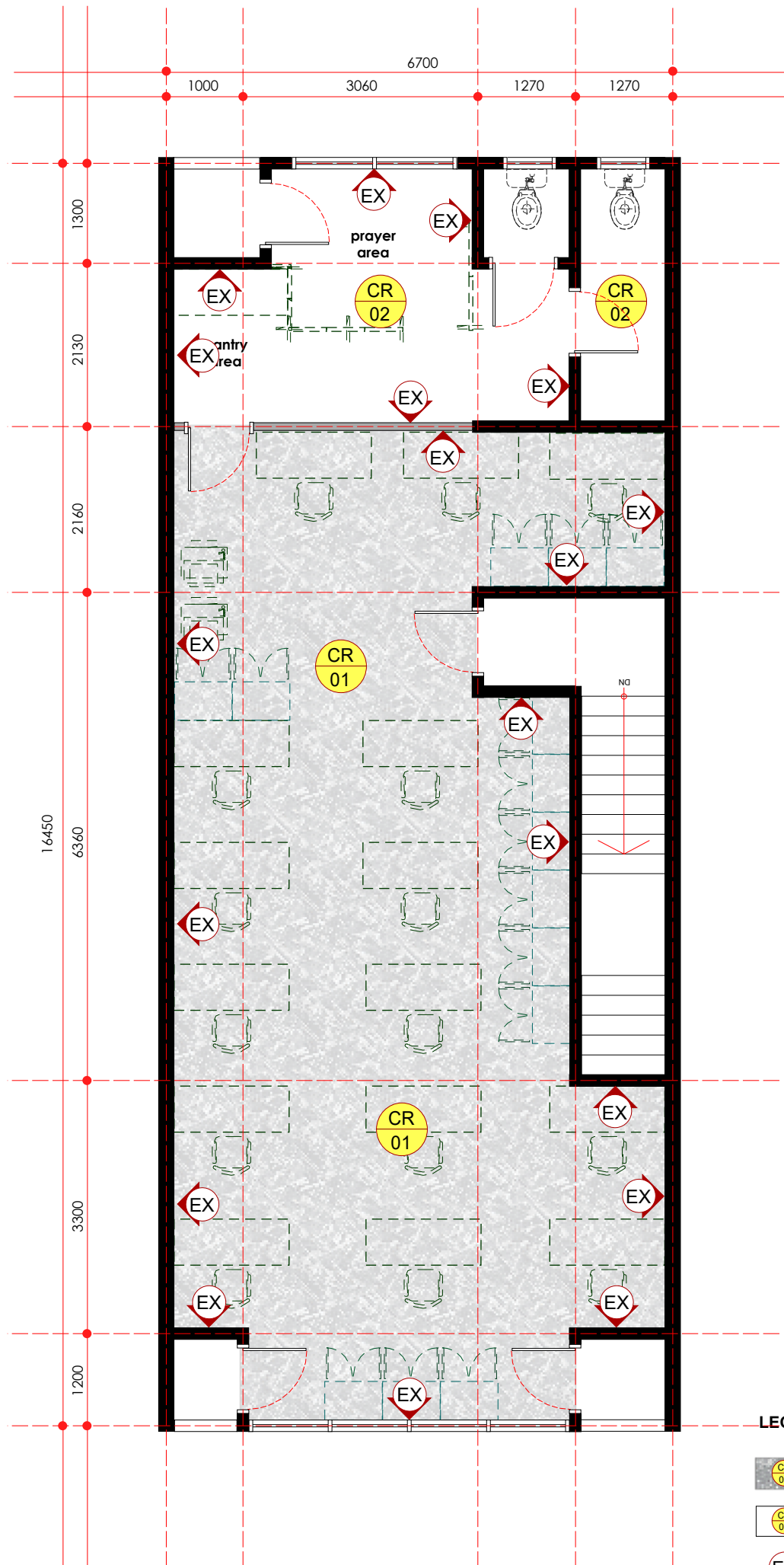
finishing layout plan - first floor scale 1: 75
