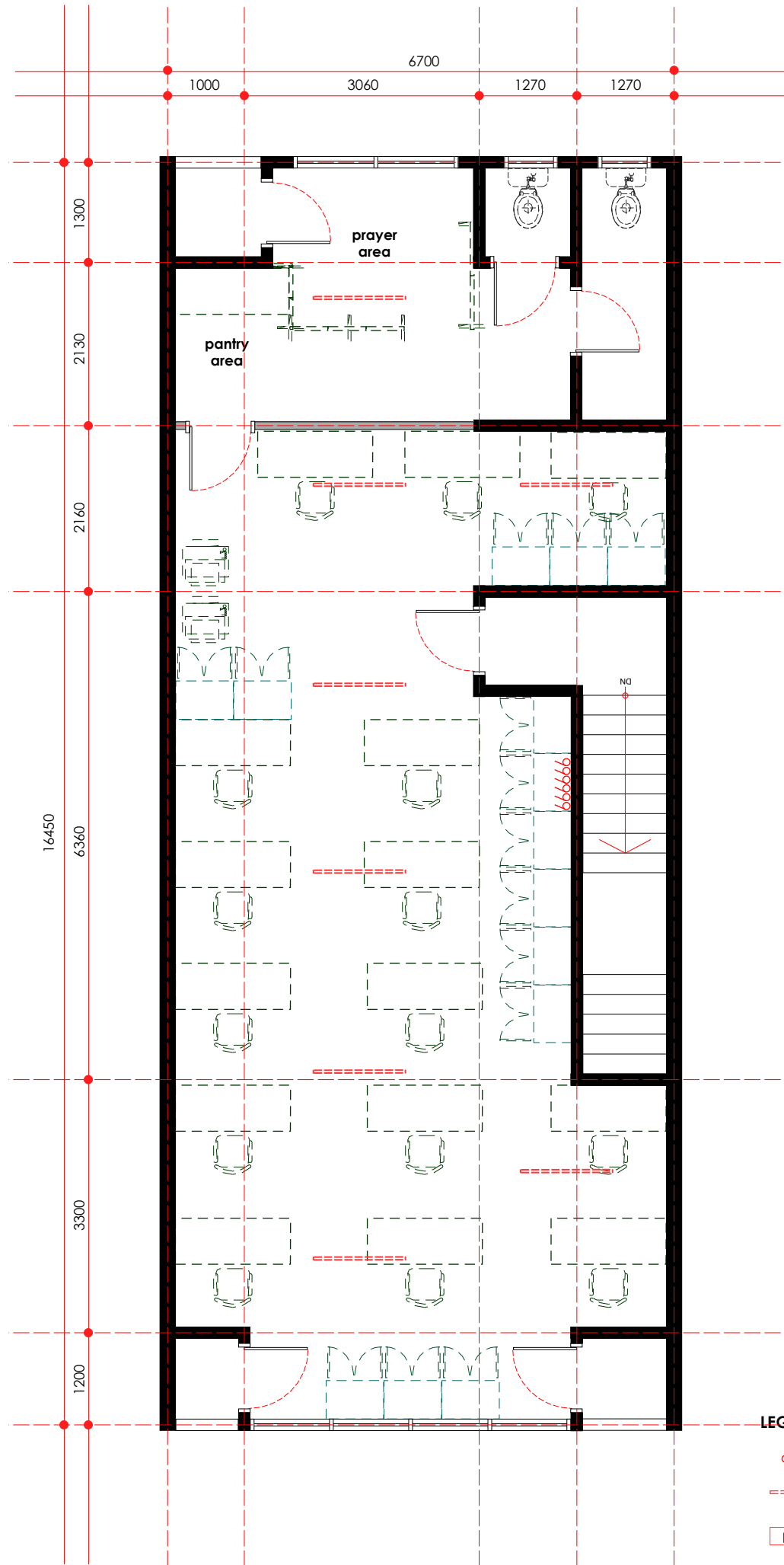
electrical point layout plan - first floor scale 1: 75
