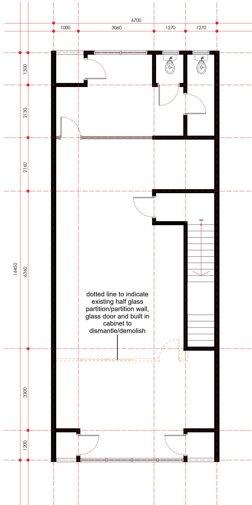
existing layout plan - first floor scale 1: 75
