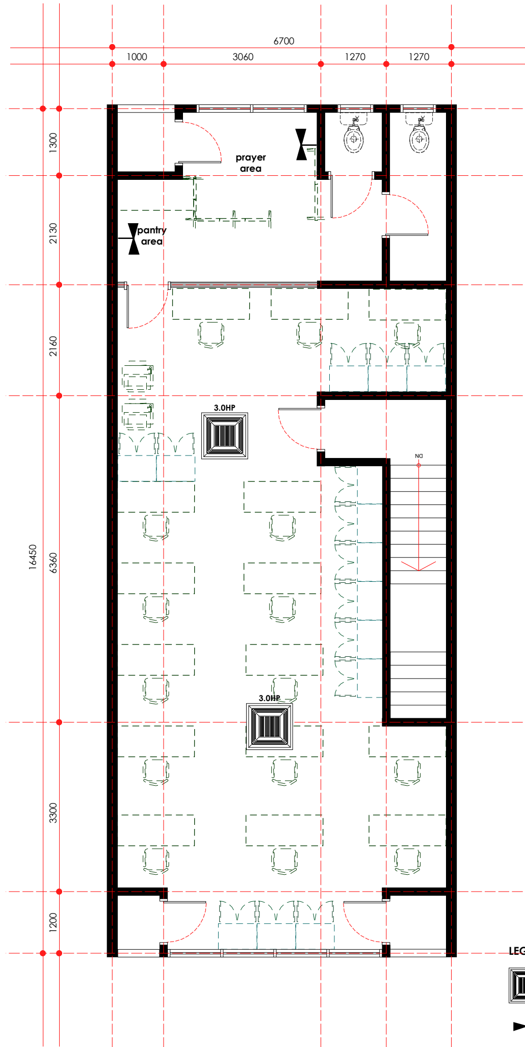
mechanical point layout plan - first floor scale 1: 75
