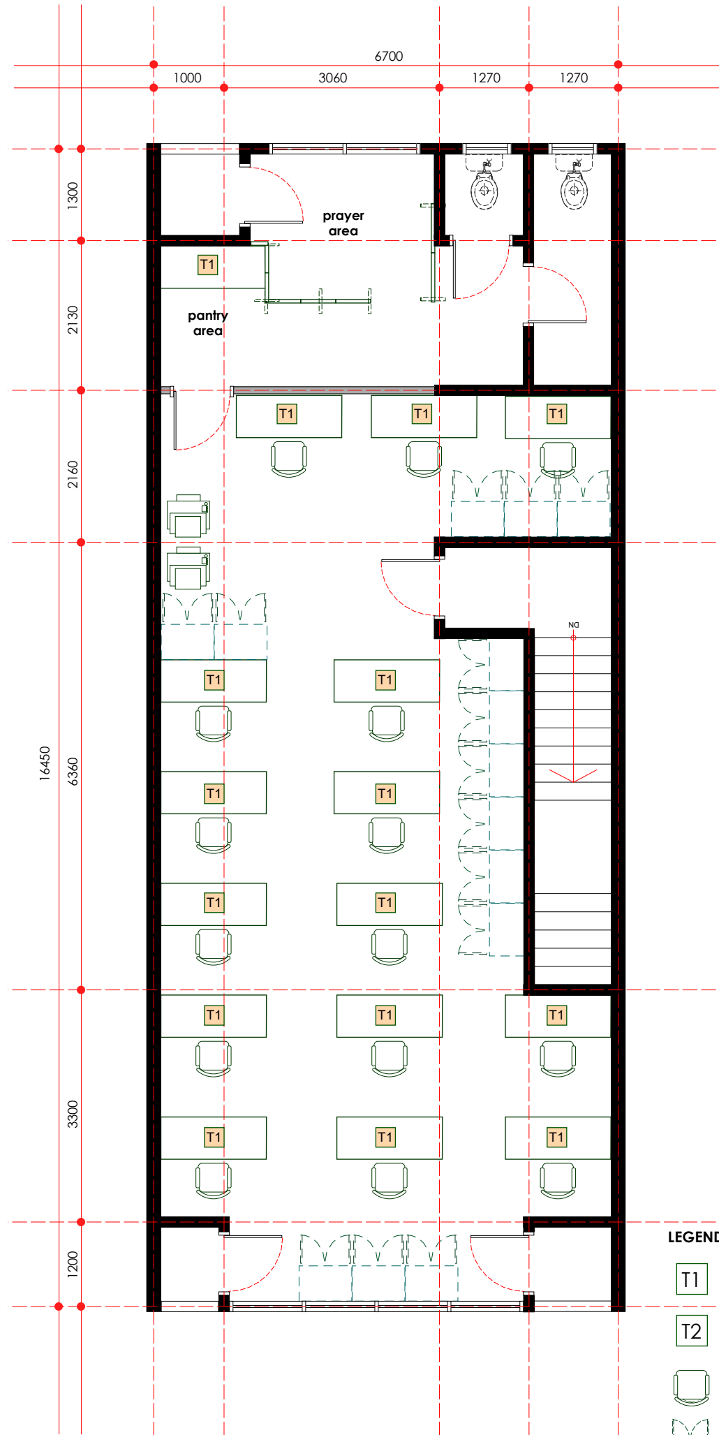
furniture layout plan - first floor scale 1: 75
