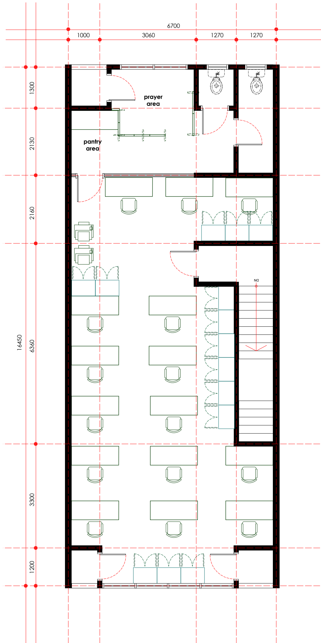
proposed layout plan - first floor scale 1: 75
