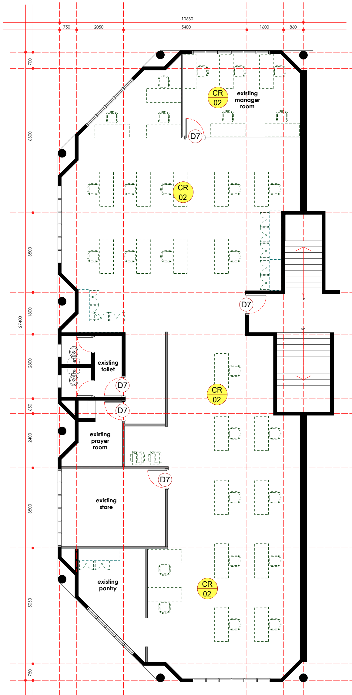
finishing layout plan - first floor scale 1: 75
