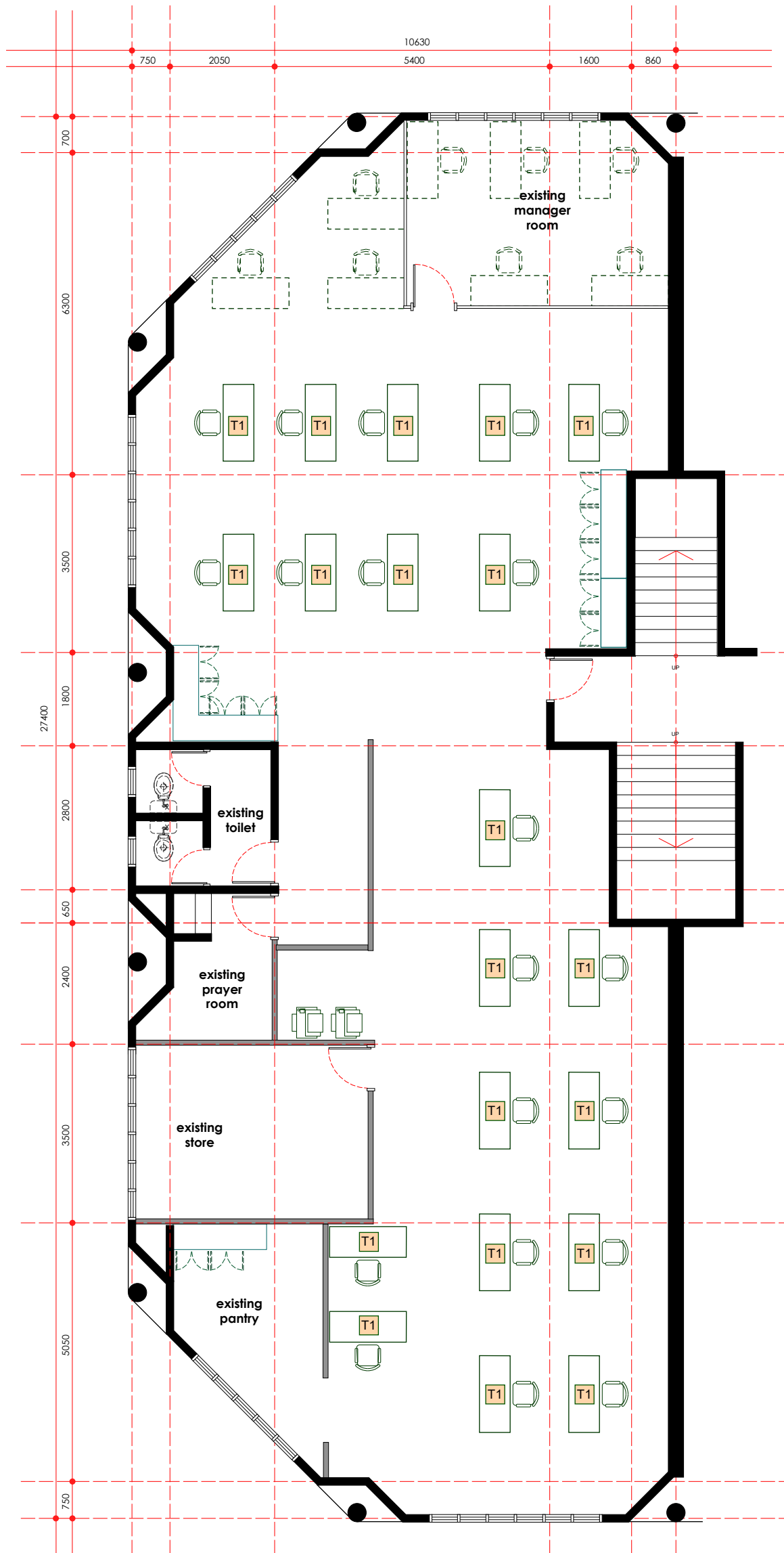
furniture layout plan - first floor scale 1: 100
