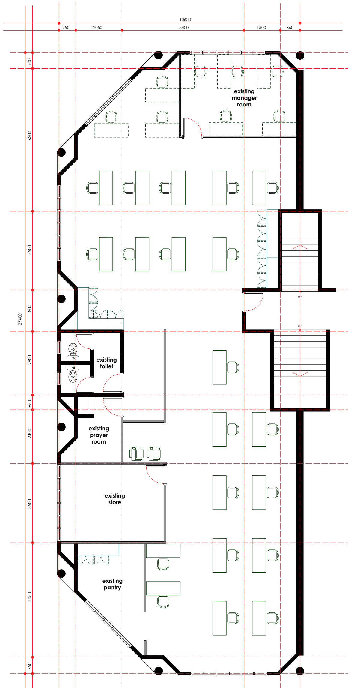
proposed layout plan - first floor scale 1: 75
