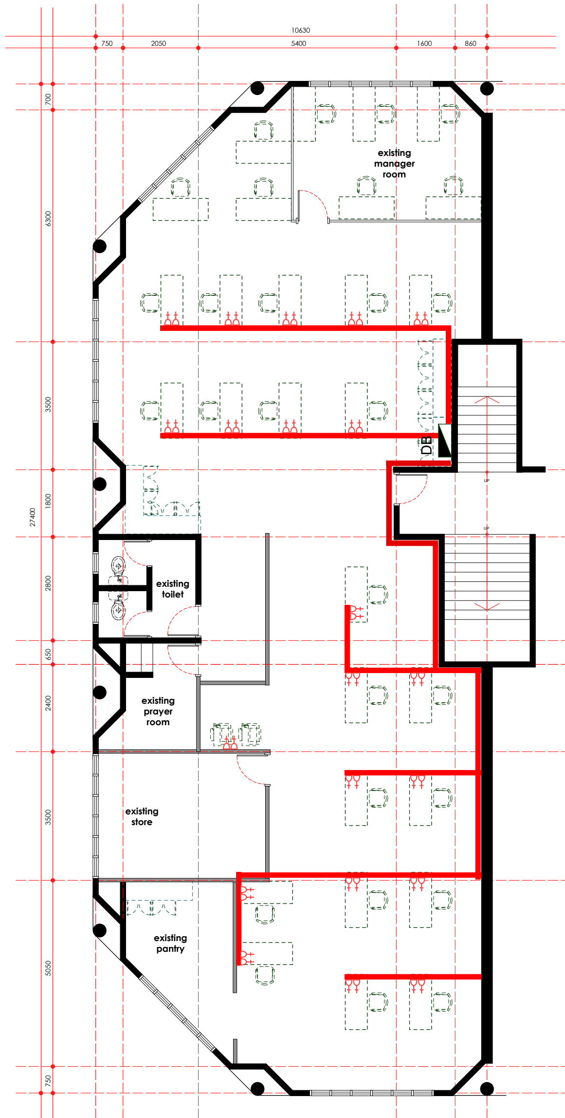
cabling route & SSO point layout plan - first floor scale 1: 100
