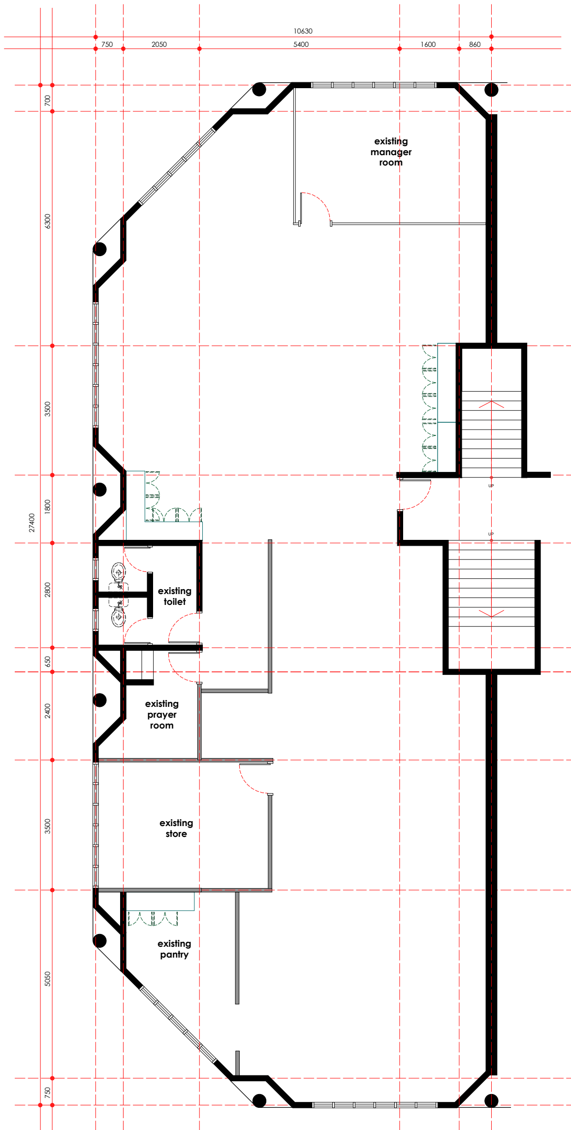
existing layout plan - first floor scale 1: 75
