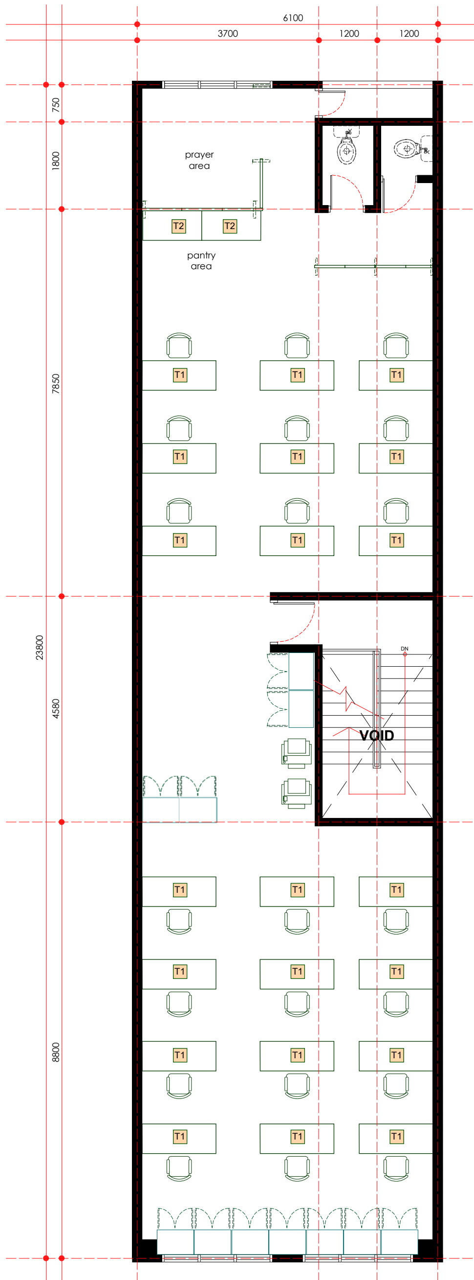
furniture layout plan - second floor scale 1: 75
