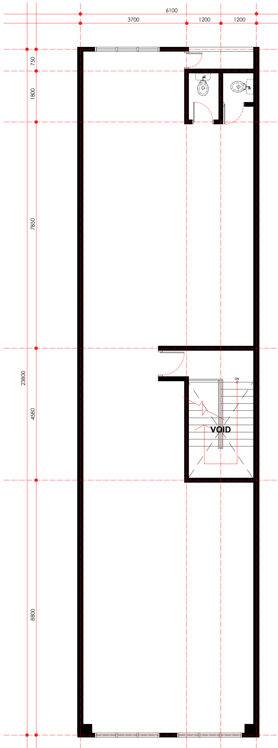
existing layout plan - second floor scale 1: 75
