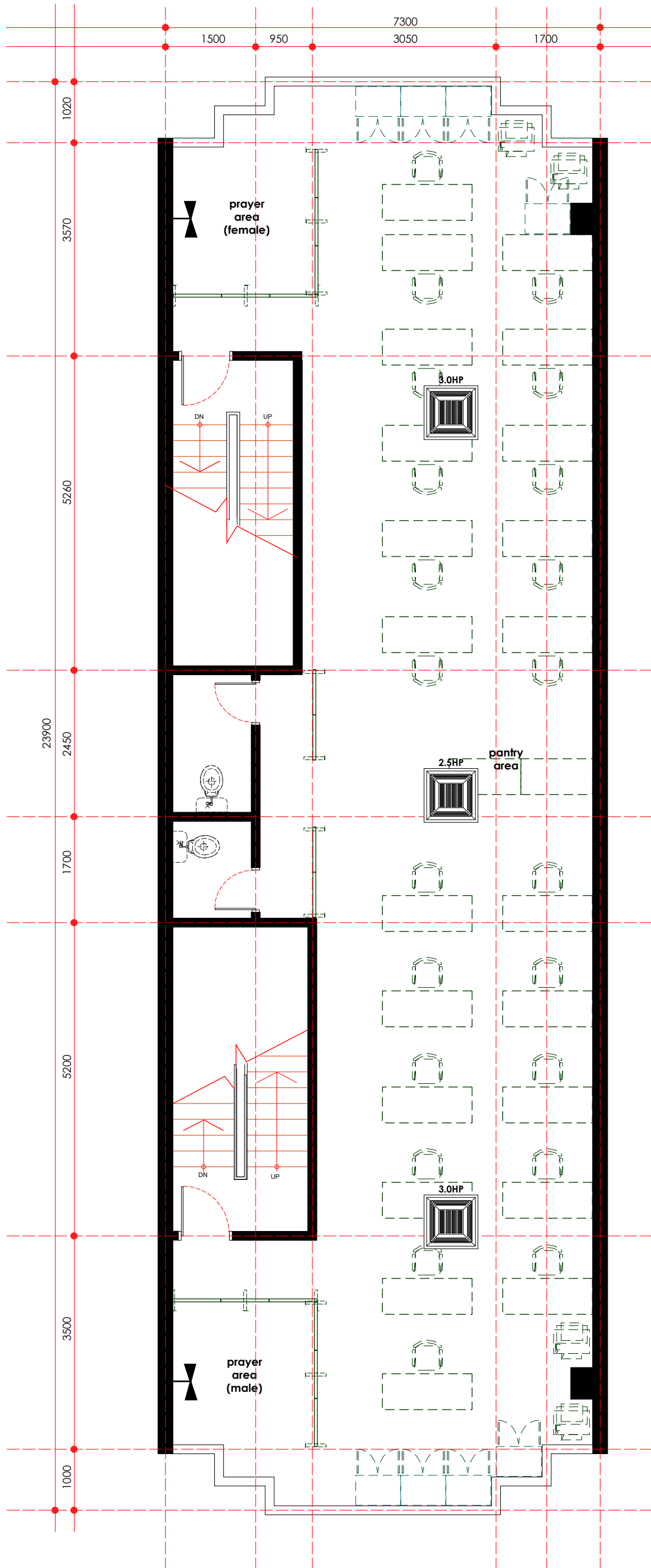
mechanical point layout plan - Second floor scale 1: 75
