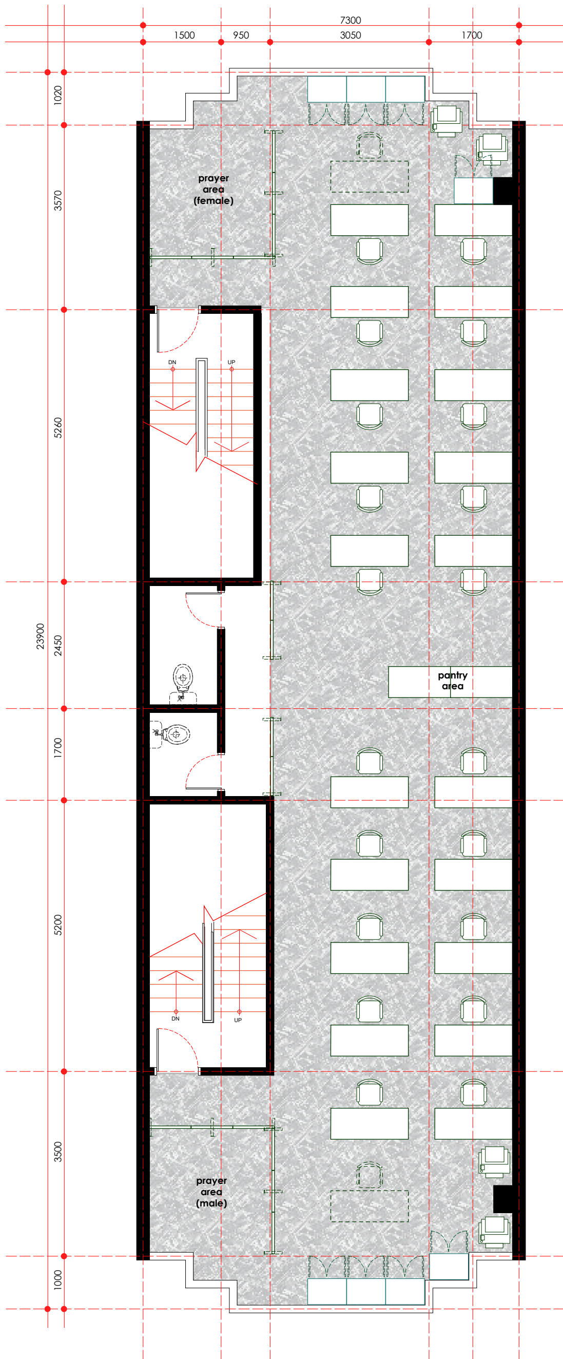
proposed layout plan - Second floor scale 1: 75
