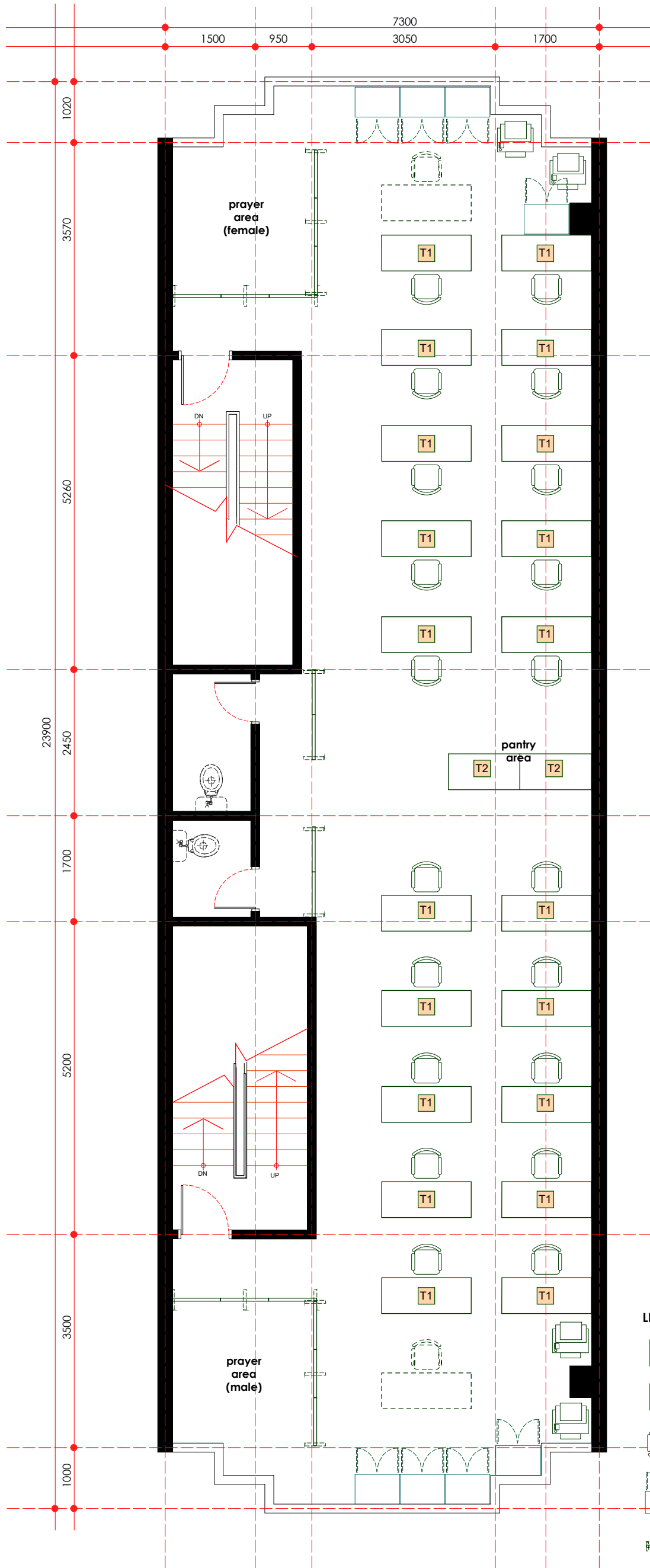
furniture layout plan - Second floor scale 1: 75
