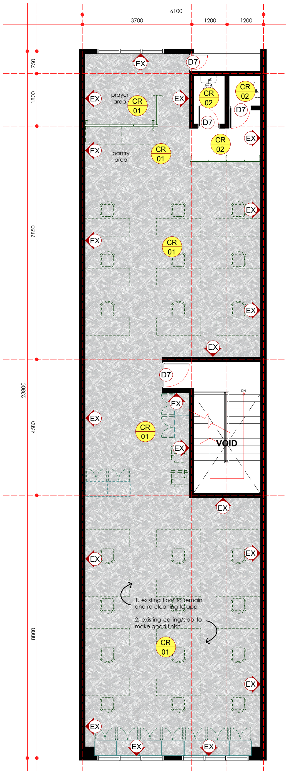
finishing layout plan - second floor scale 1: 75
