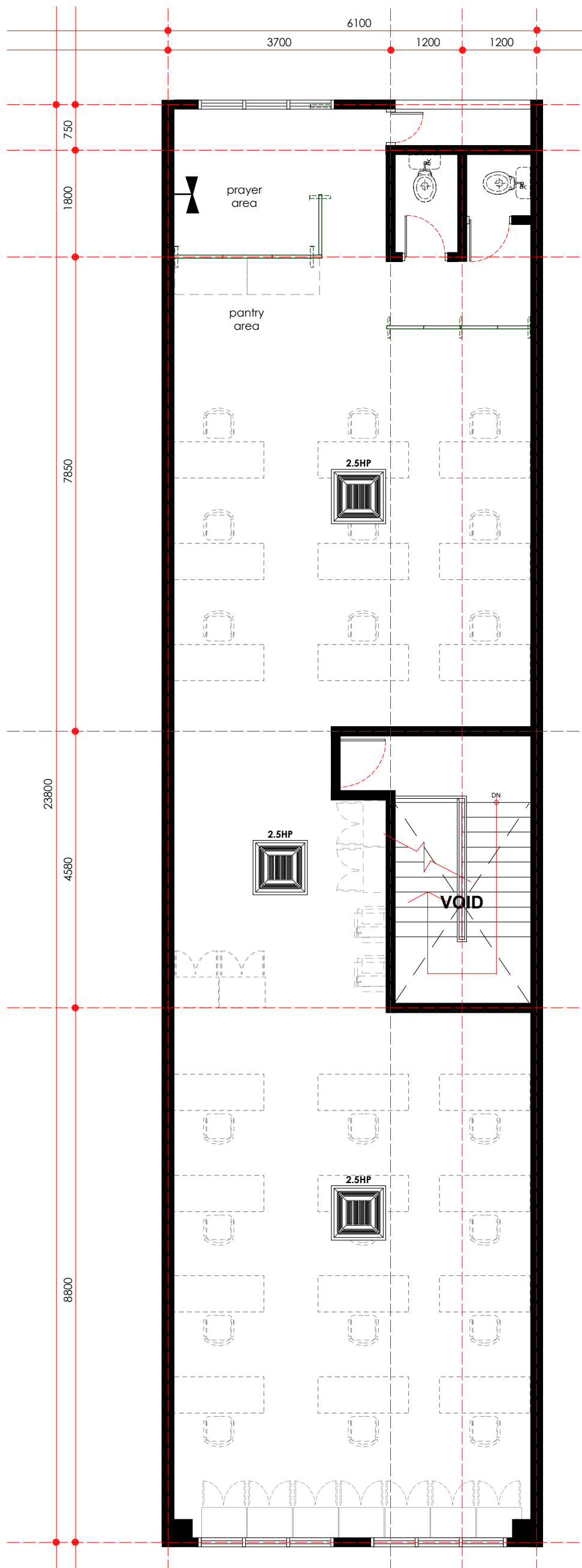
mechanical point layout plan - second floor scale 1: 75
