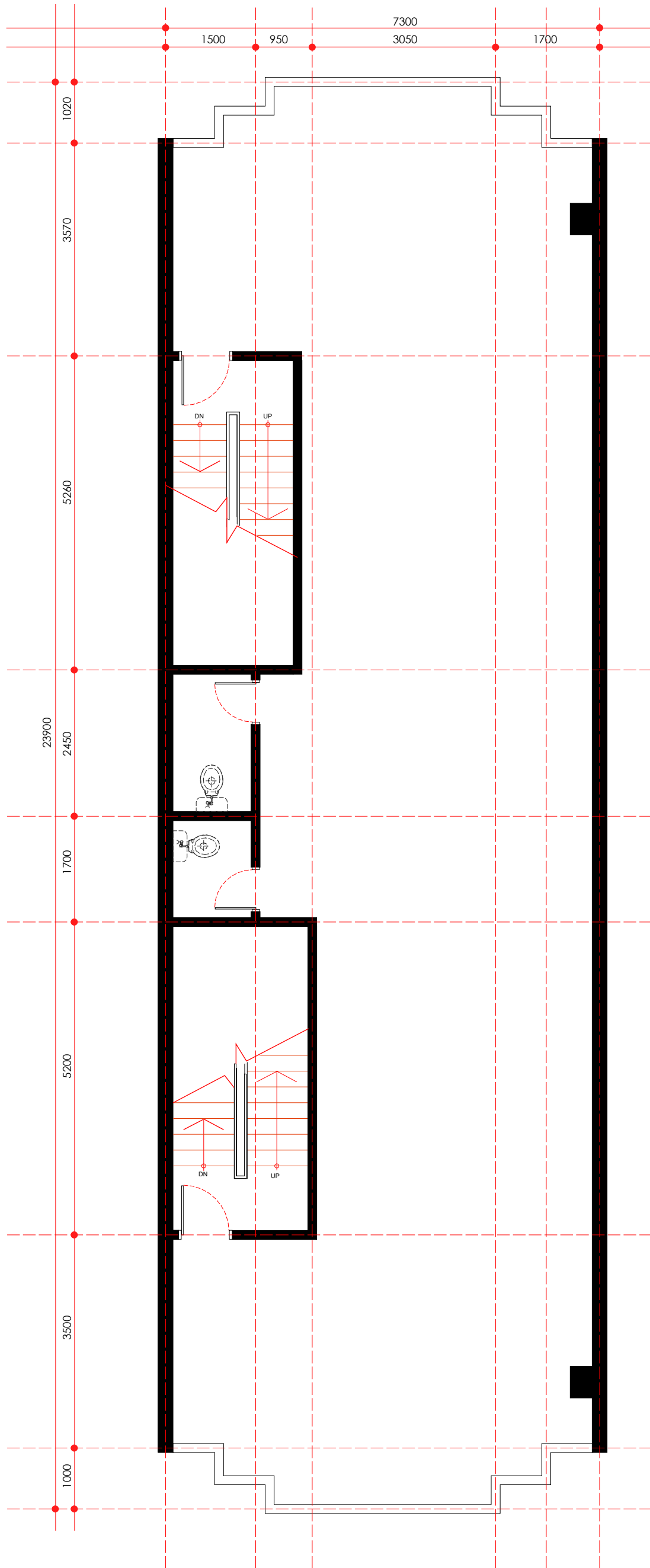
existing layout plan - Second floor scale 1: 75
