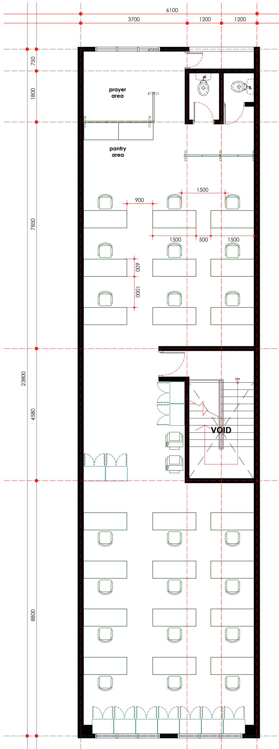
proposed layout plan - second floor scale 1: 75
