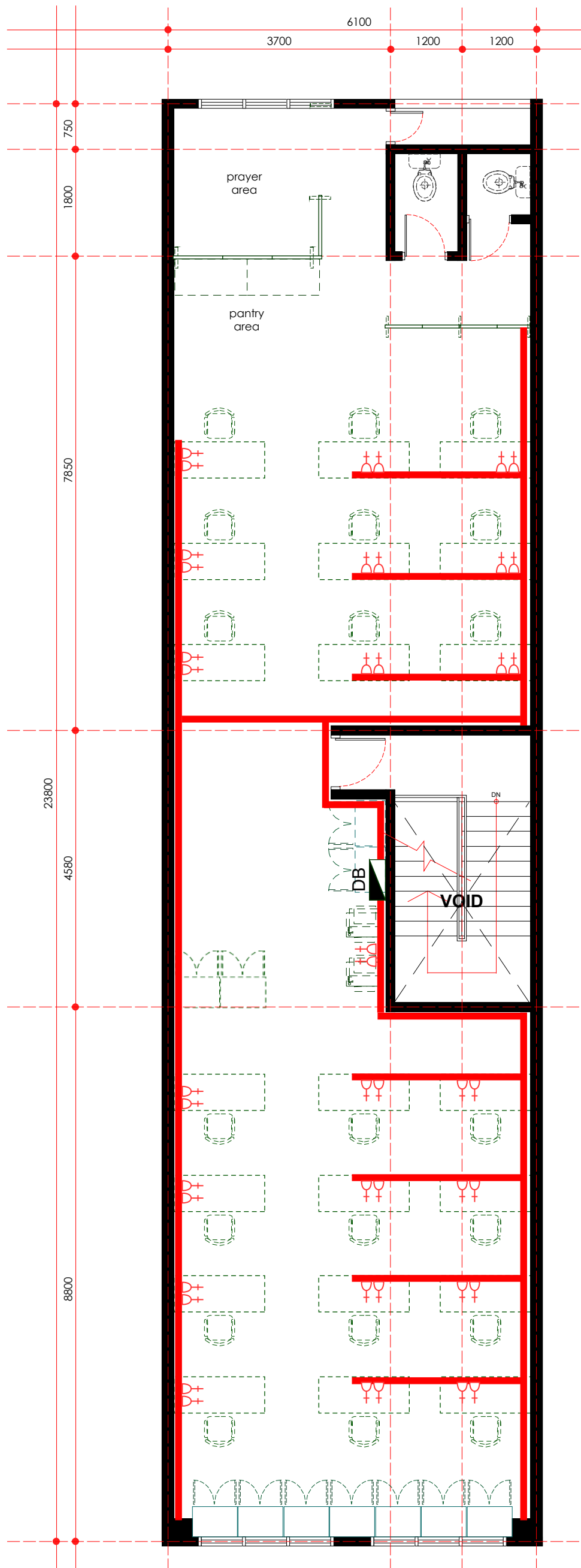
cabling route & point layout plan - second floor scale 1: 75
