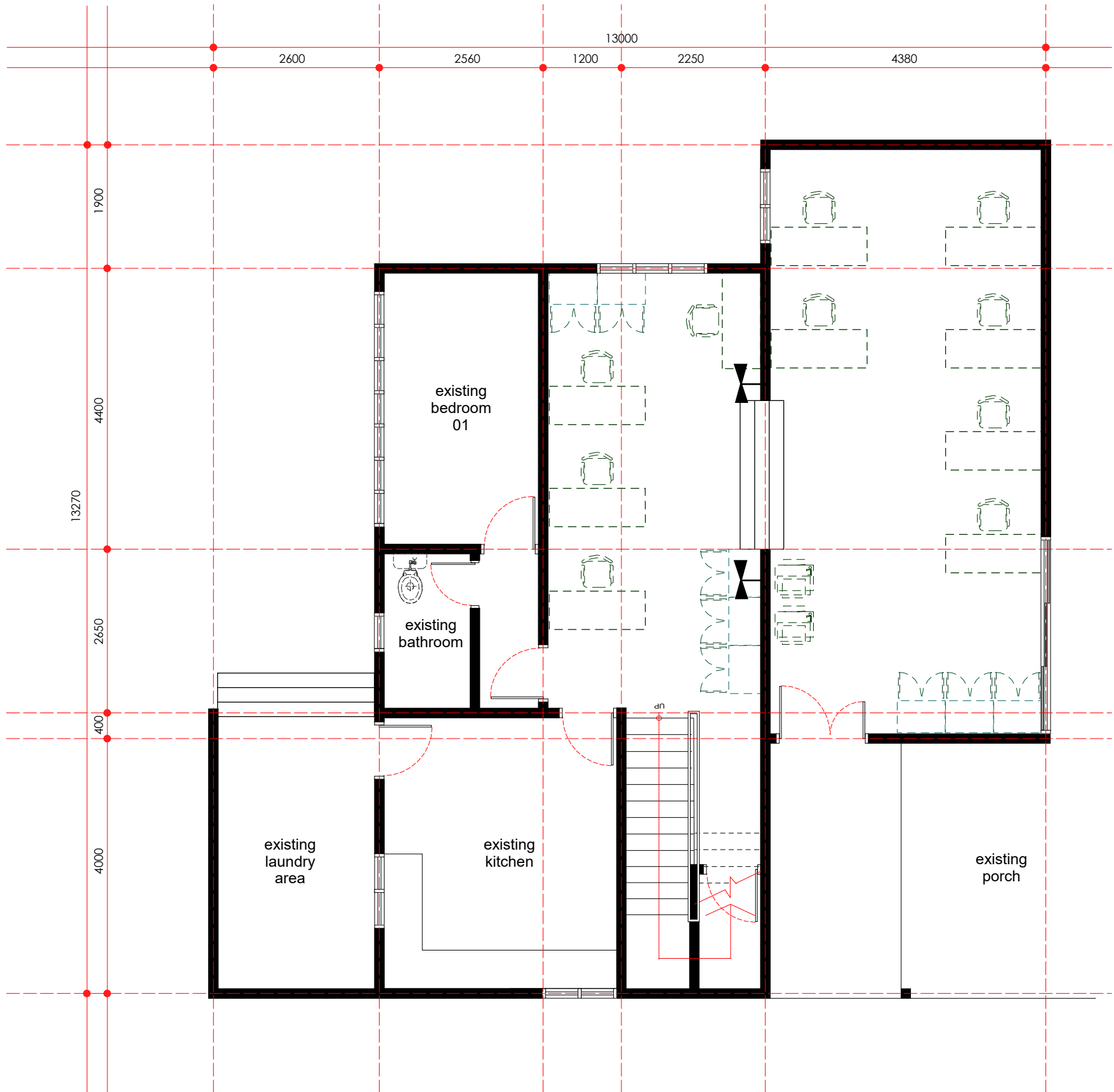
mechanical point layout plan - ground floor scale 1: 75
