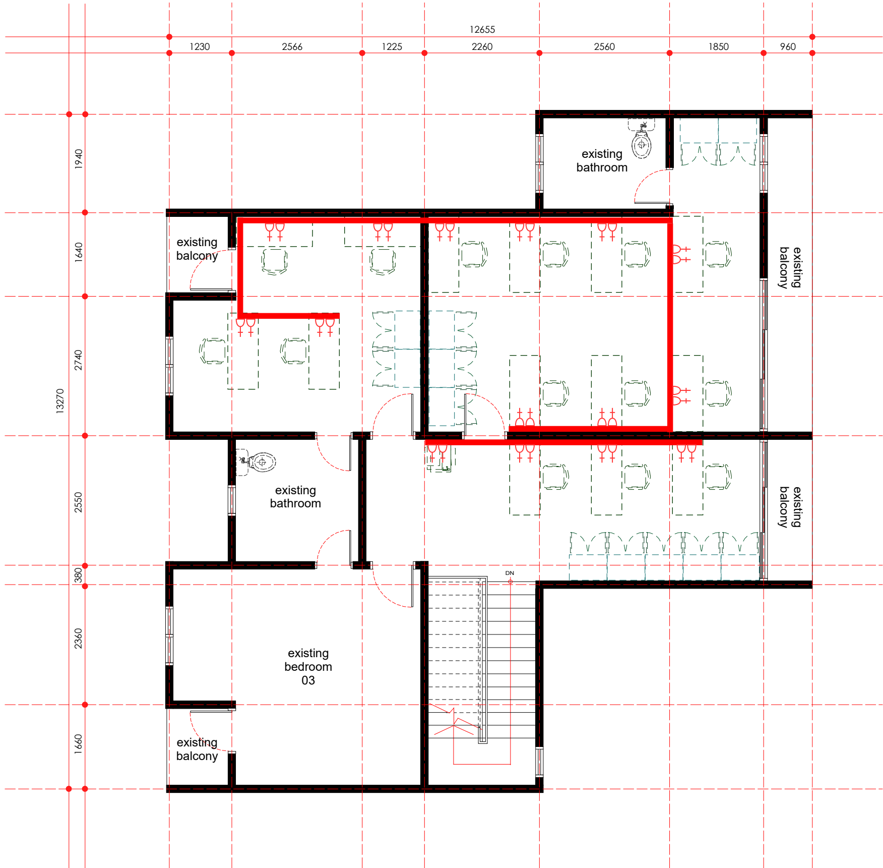
cabling route & SSO point layout plan - first floor scale 1: 75
