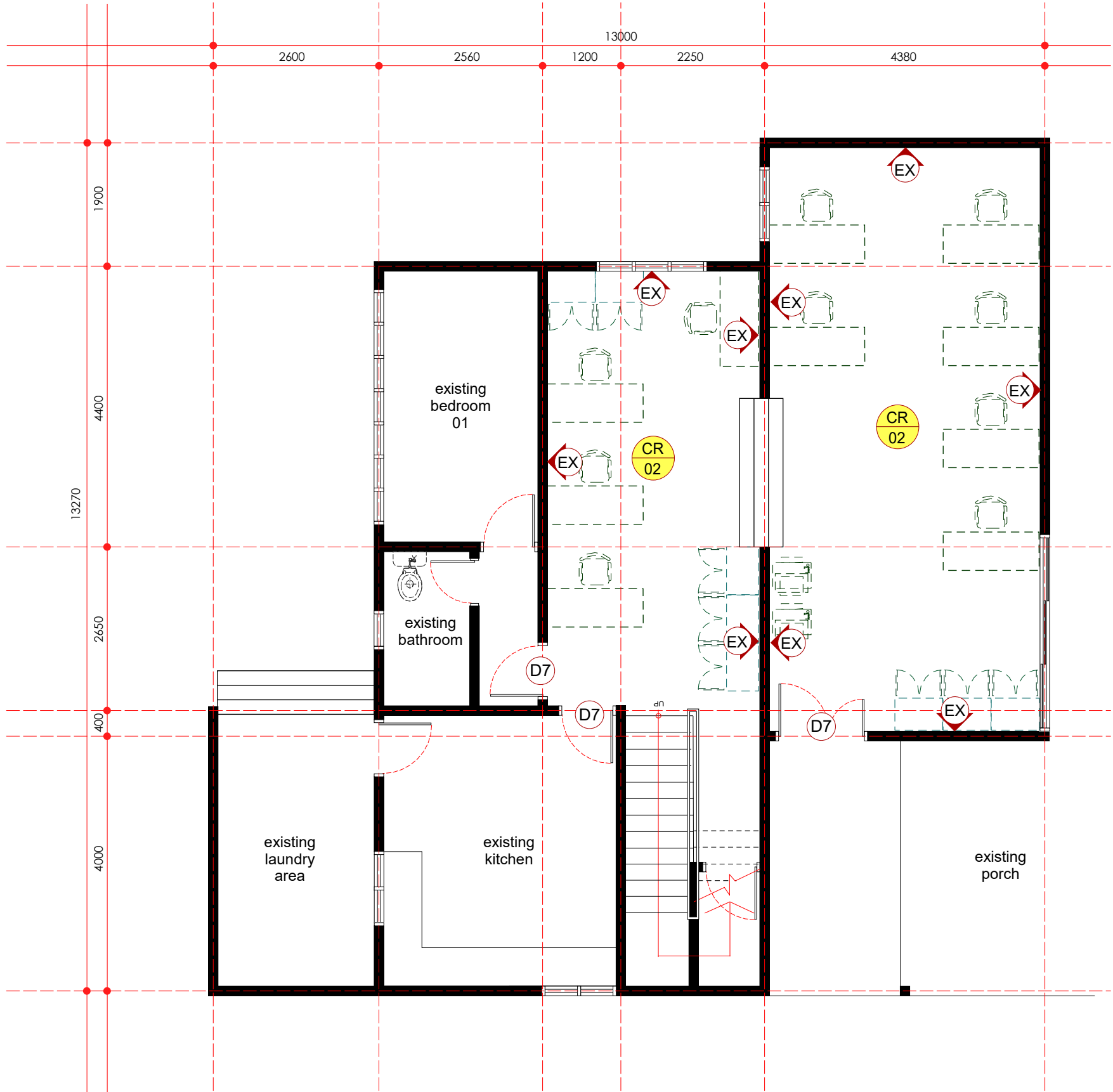
finishing layout plan - ground floor scale 1: 75
