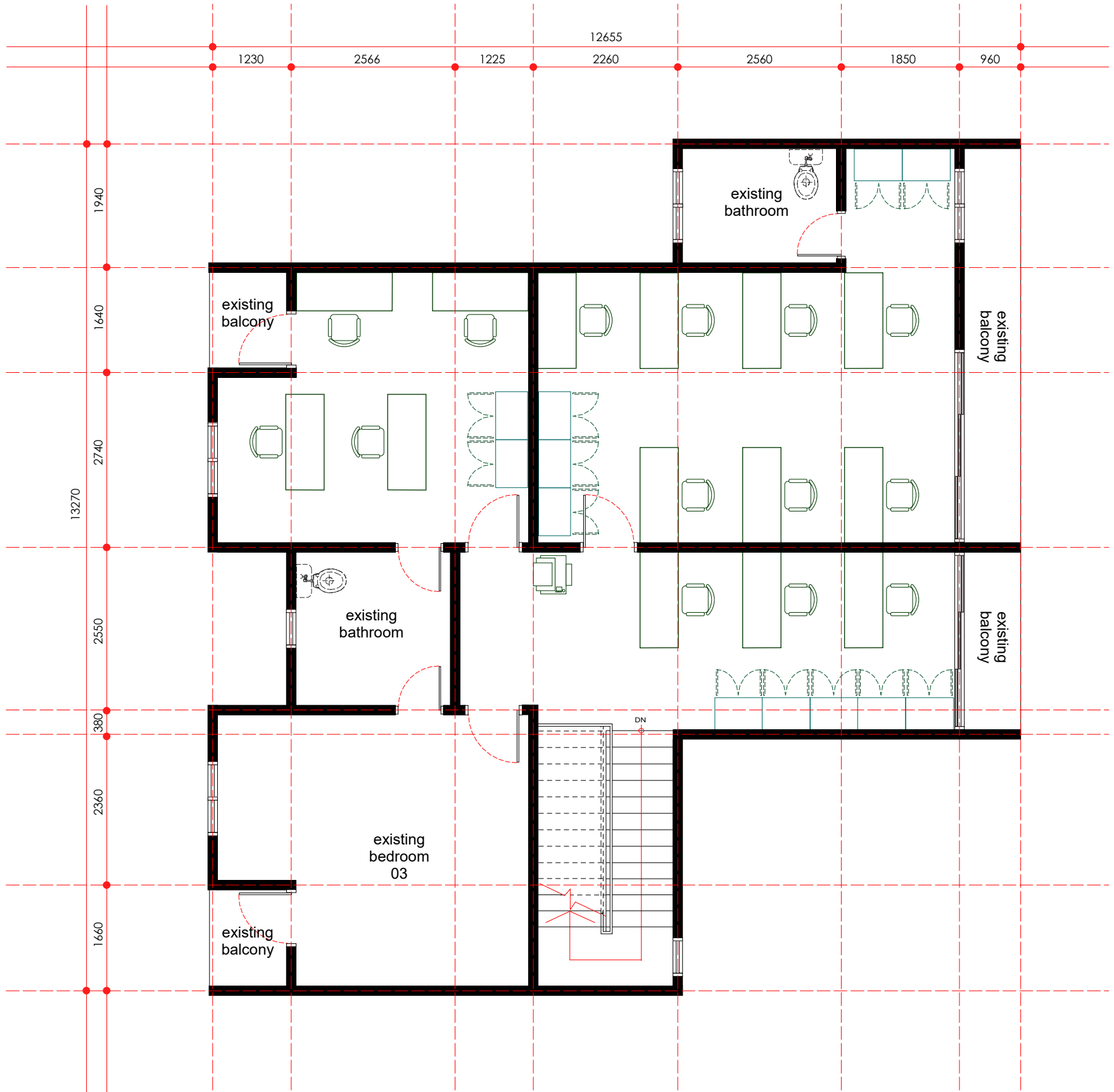
proposed layout plan - first floor scale 1:75
