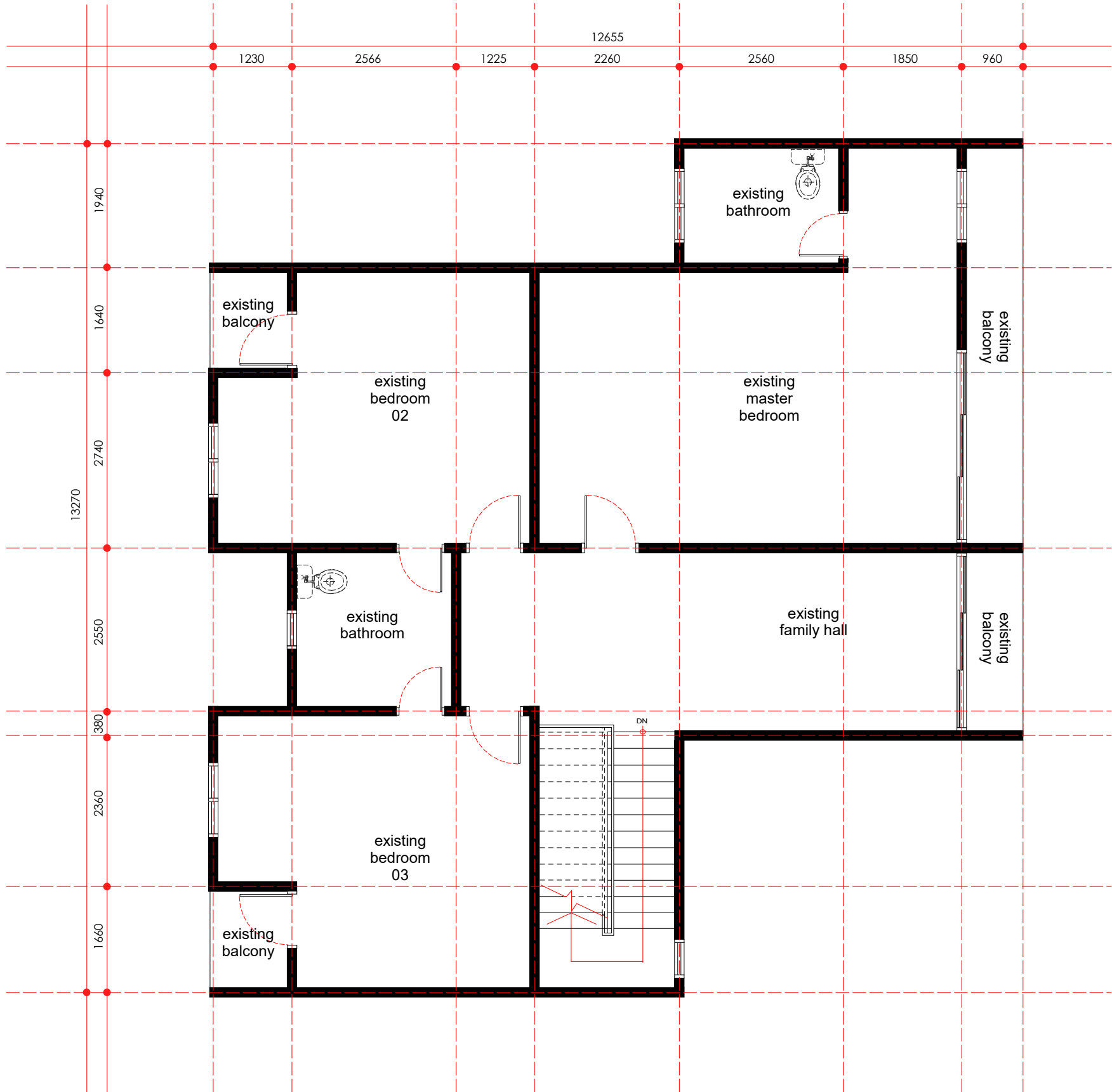
existing layout plan - first floor scale 1: 75
