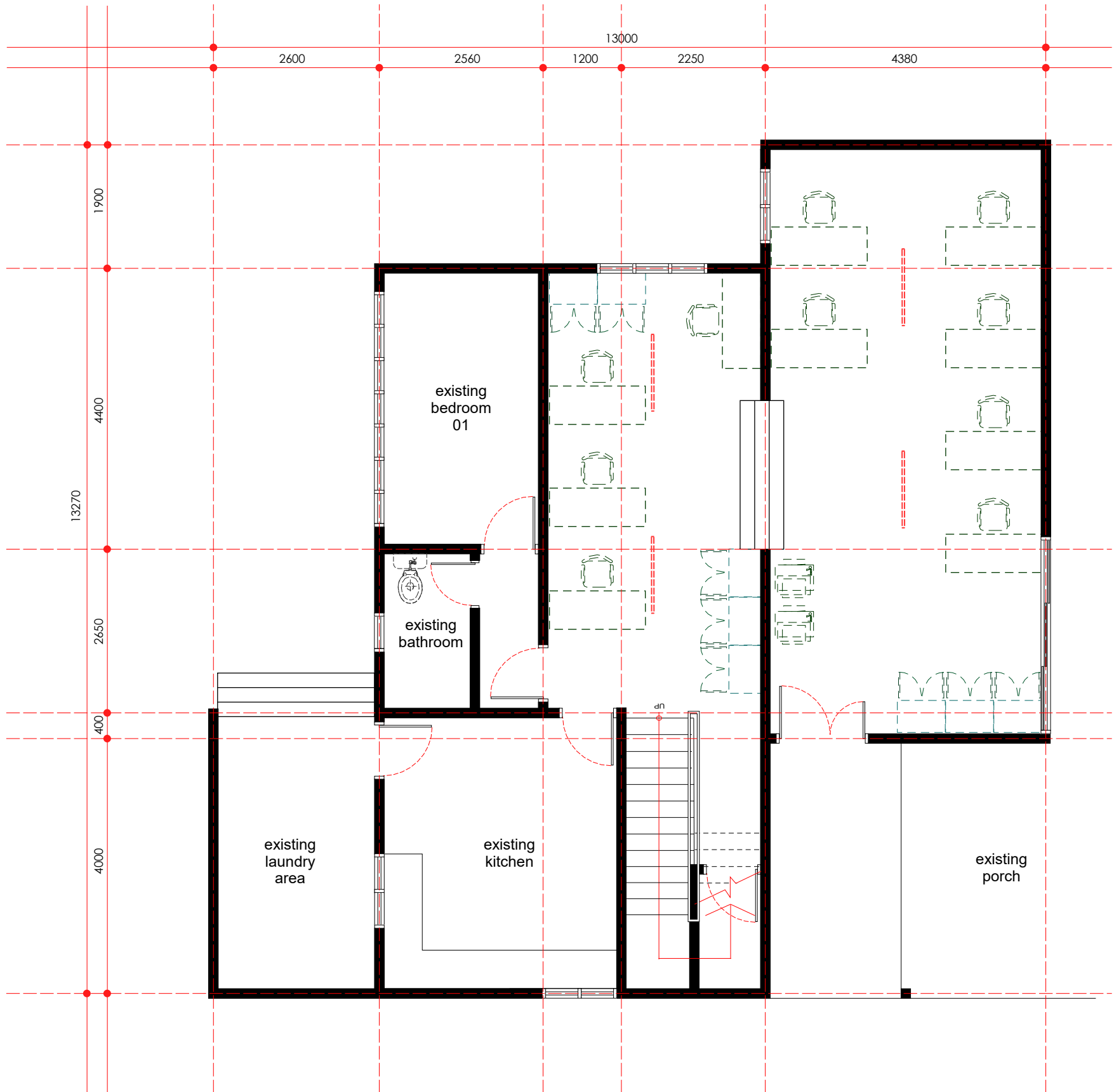
electrical point layout plan - ground floor scale 1: 75
