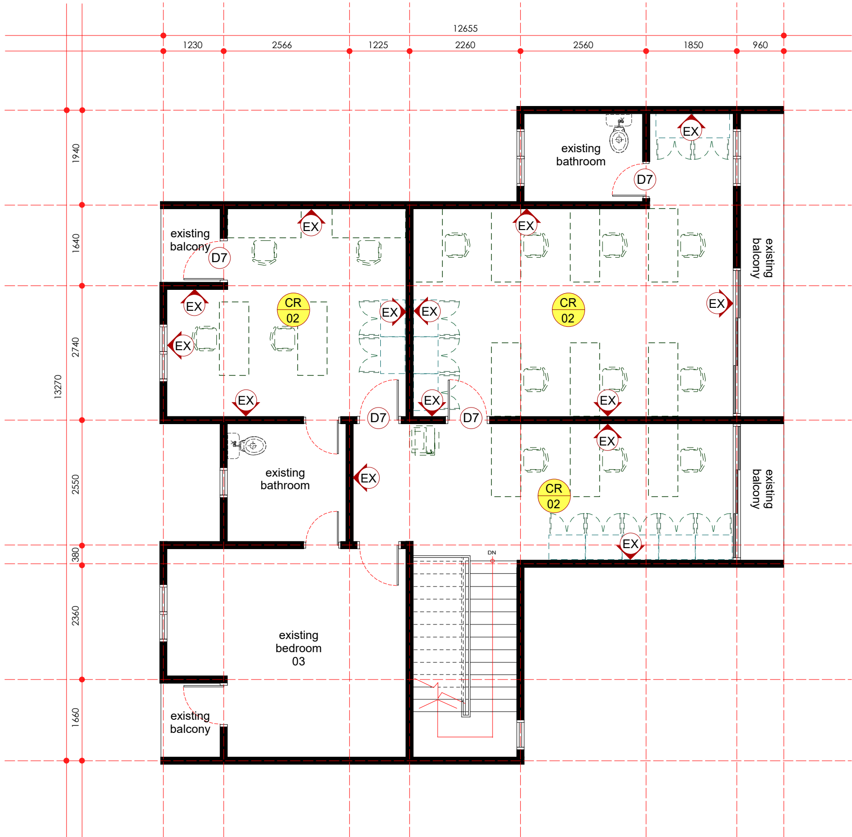
finishing layout plan - first floor scale 1: 75
