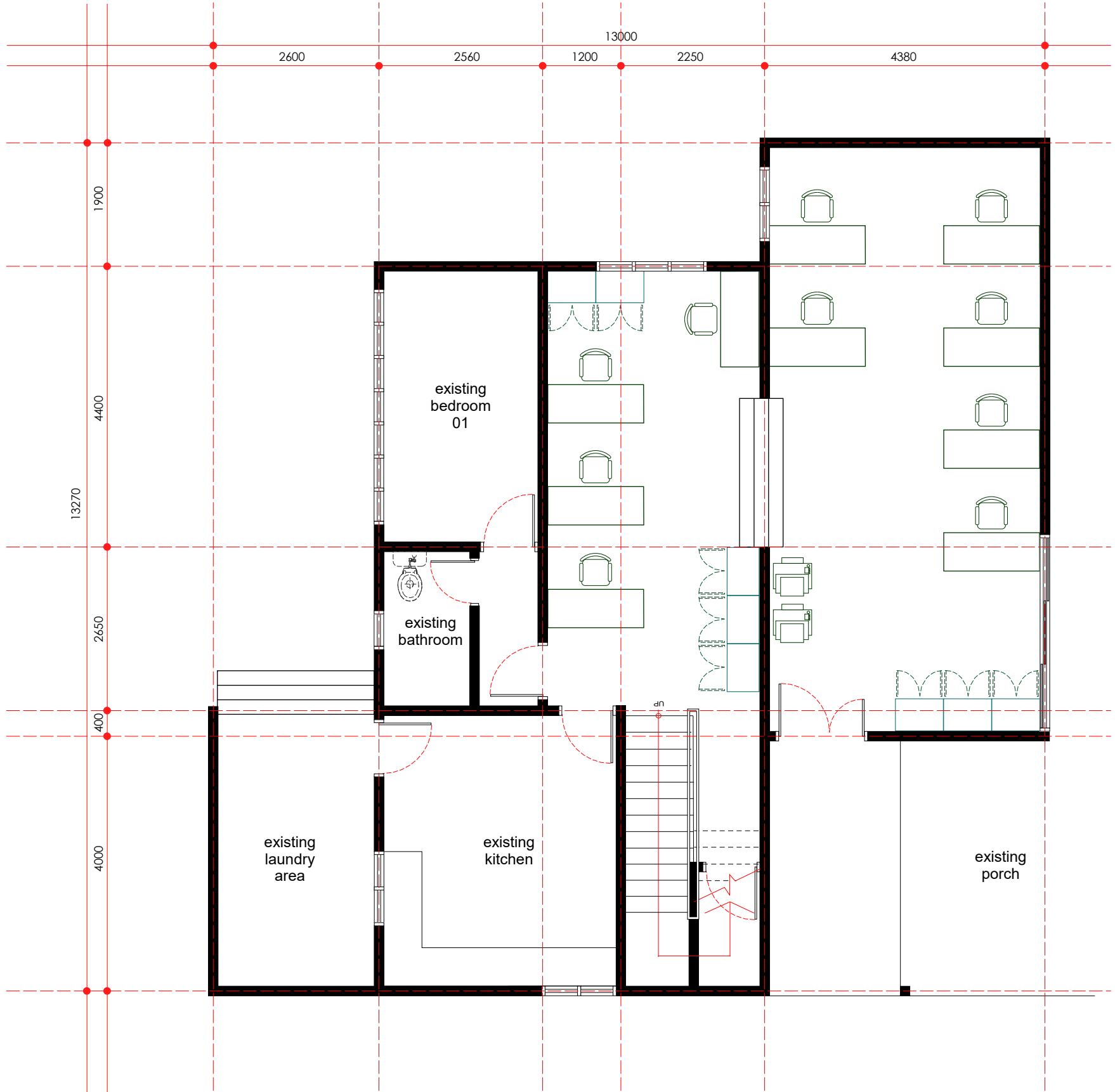
proposed layout plan - ground floor scale 1: 75
