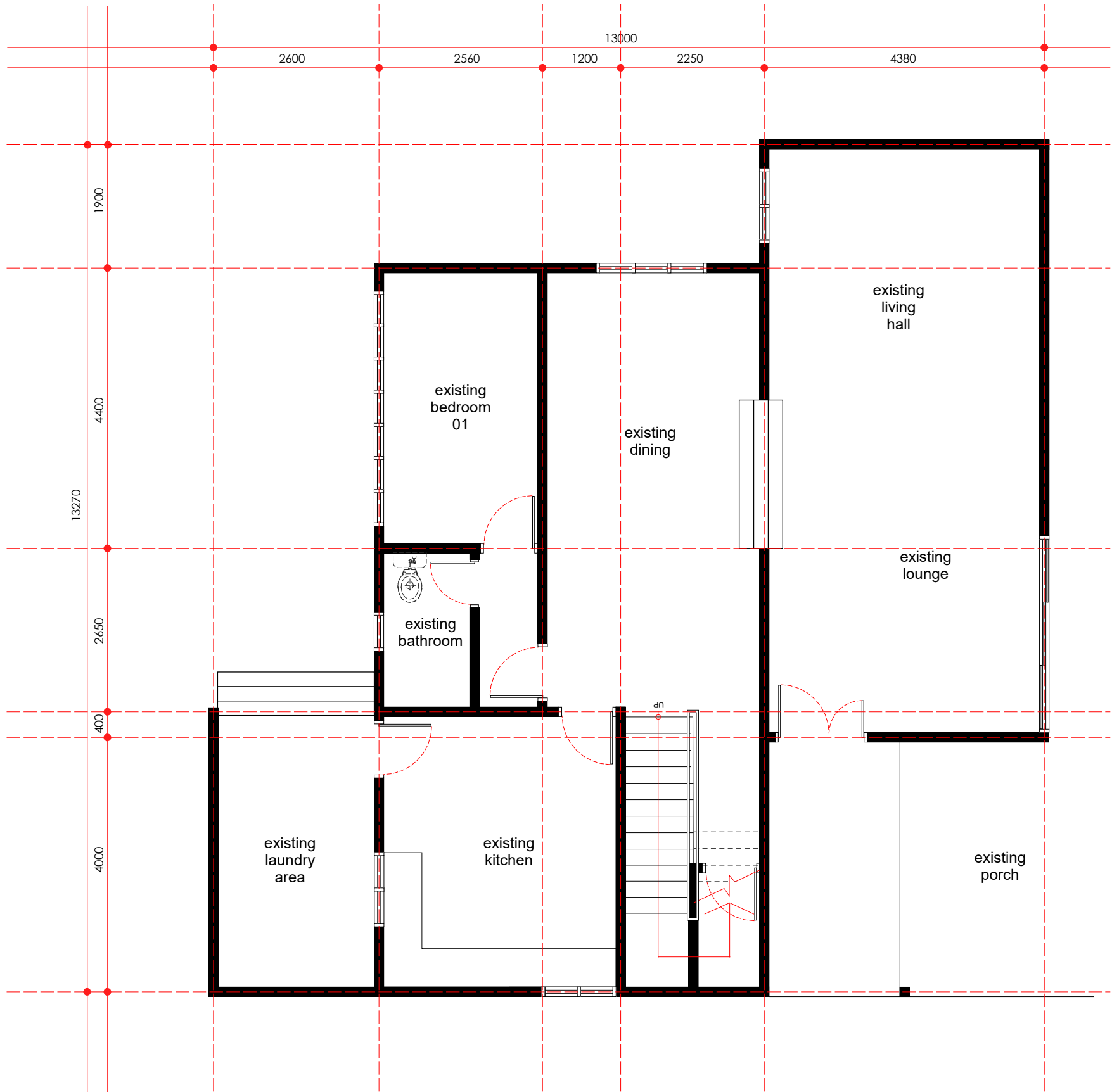
existing layout plan - ground floor scale 1: 75
