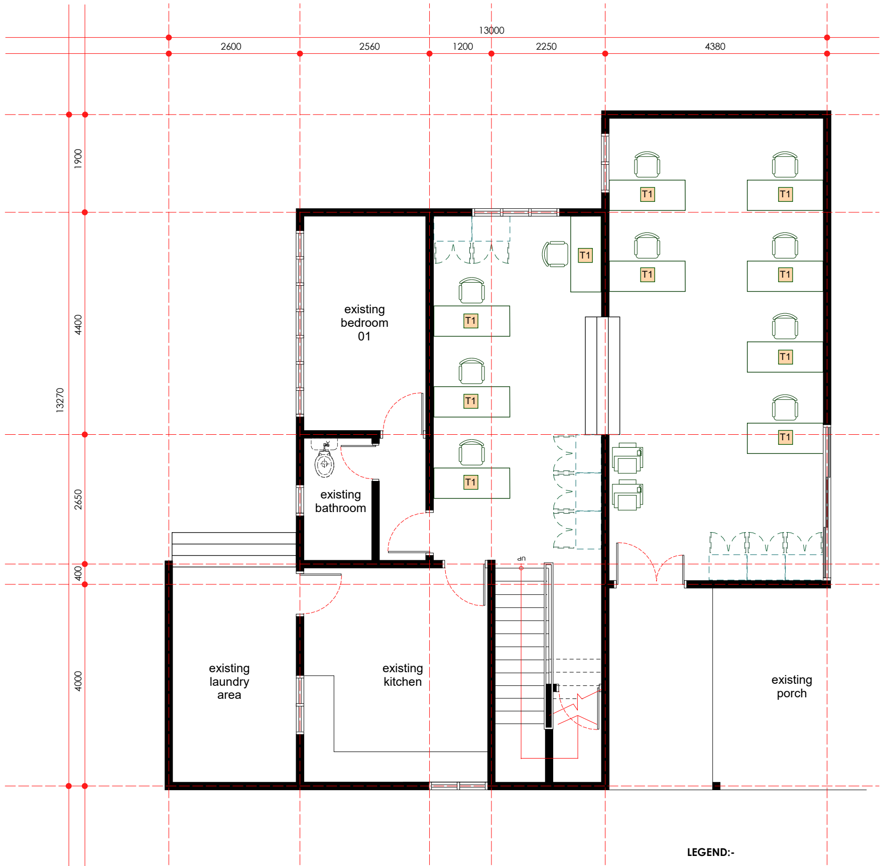
furniture layout plan - ground floor scale 1: 75
