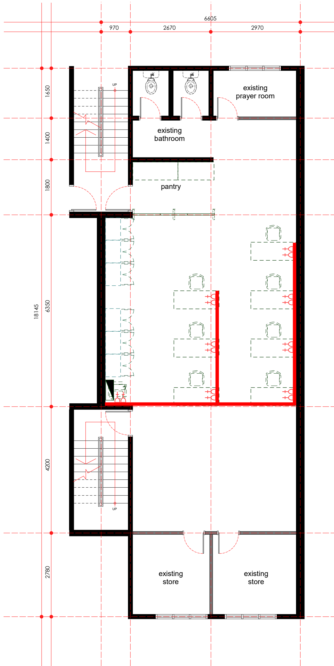
cabling route & SSO point layout plan - first floor scale 1: 75
