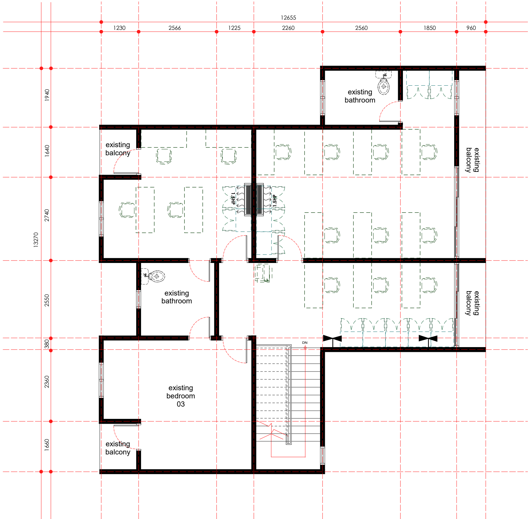
mechanical point layout plan - first floor scale 1: 75
