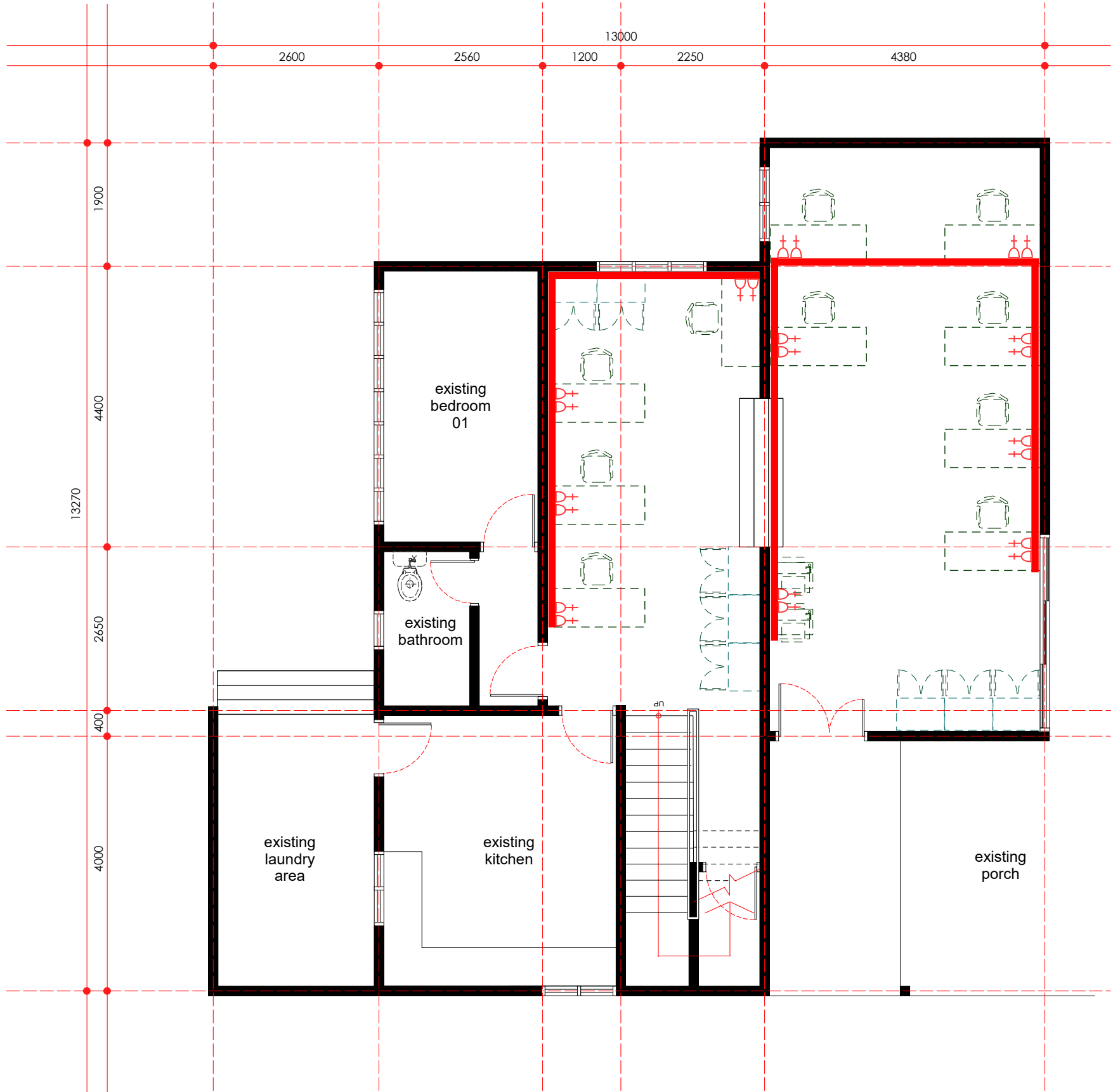
cabling route & SSO point layout plan - ground floor scale 1: 75
