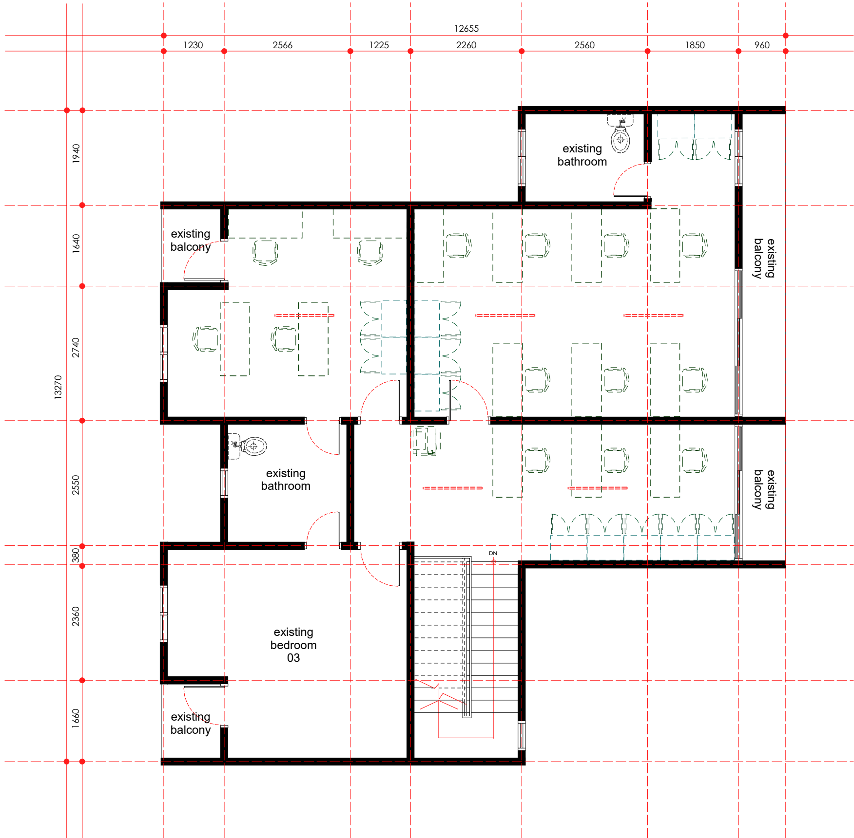
electrical point layout plan - first floor scale 1: 75
