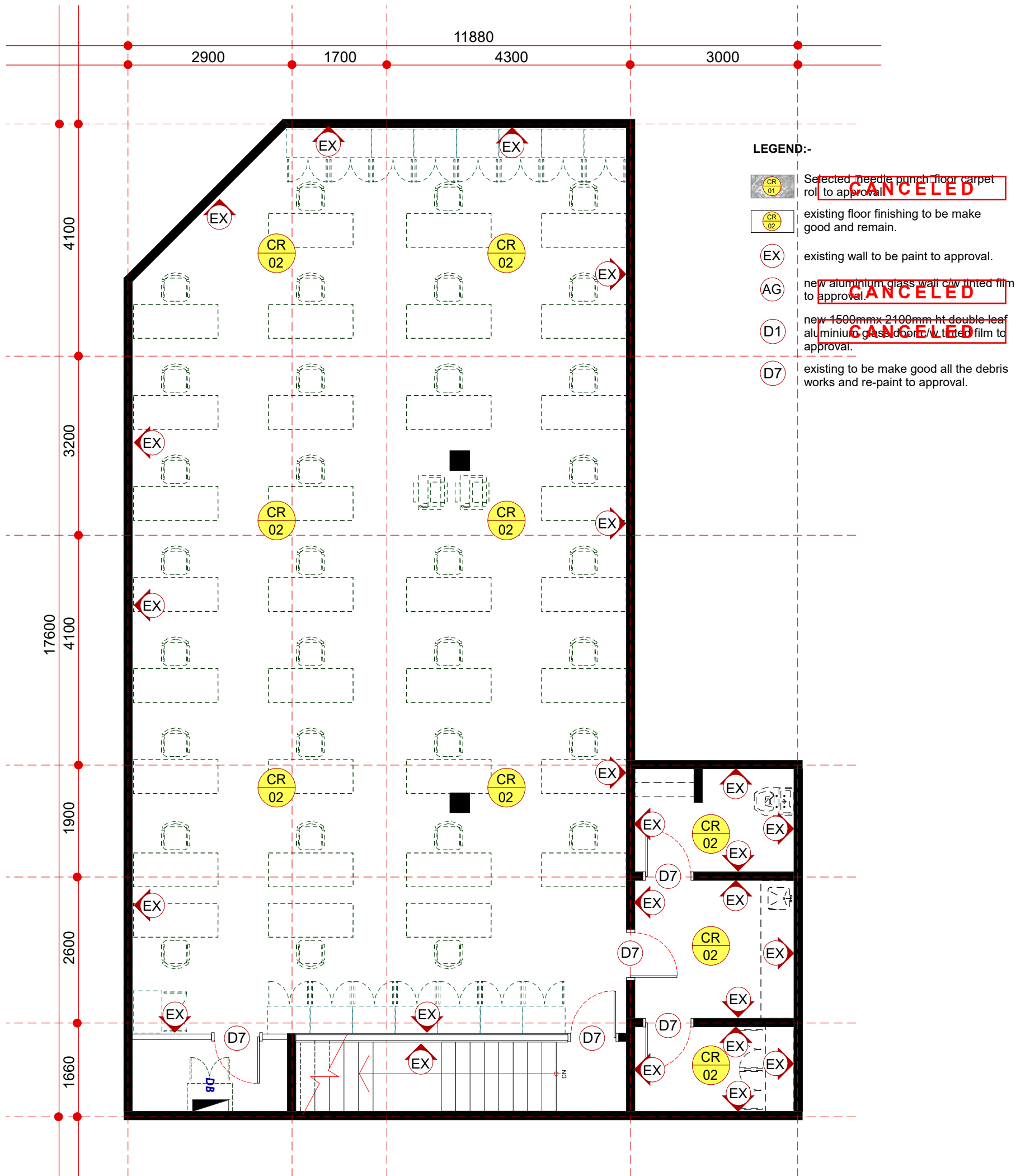
finishing layout plan - first floor scale 1: 75
