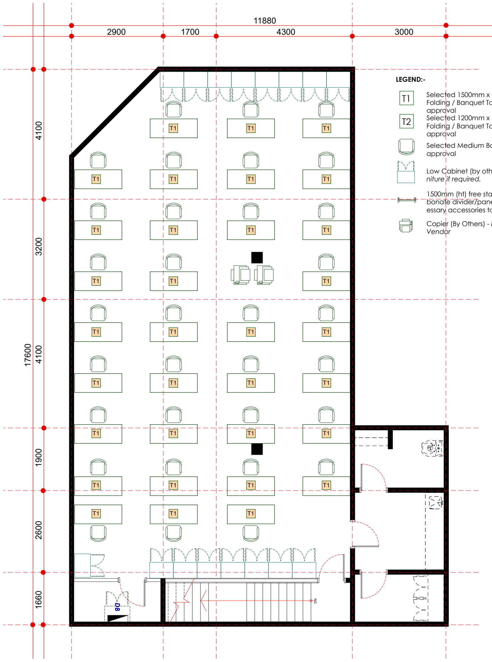
furniture layout plan - first floor scale 1: 75
