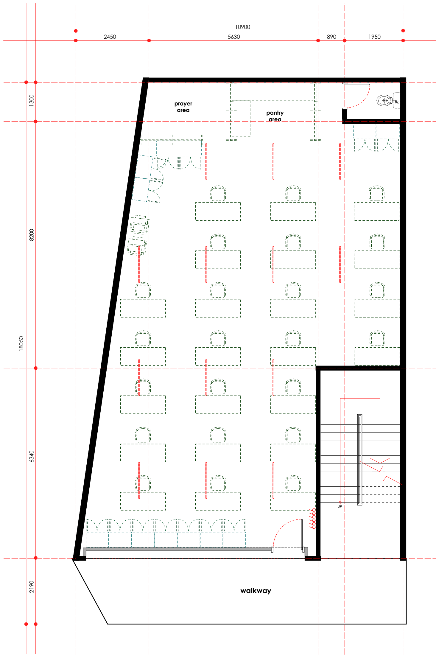
electrical point layout plan - first floor scale 1: 75
