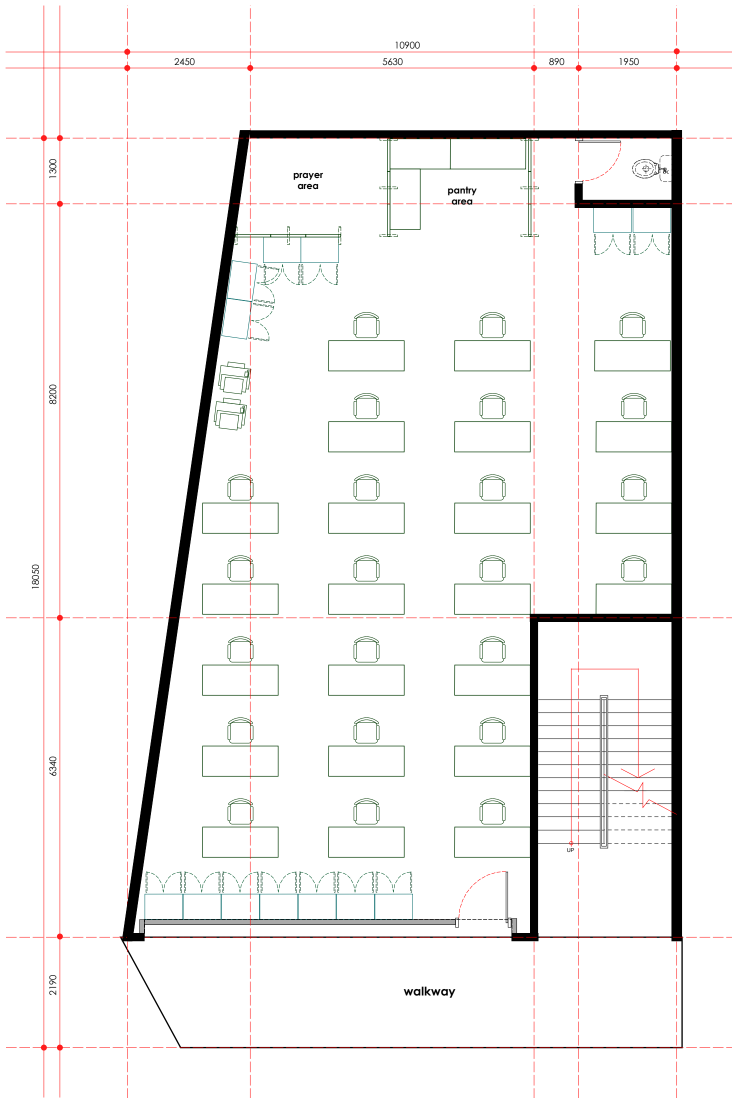
proposed layout plan - first floor scale 1: 75
