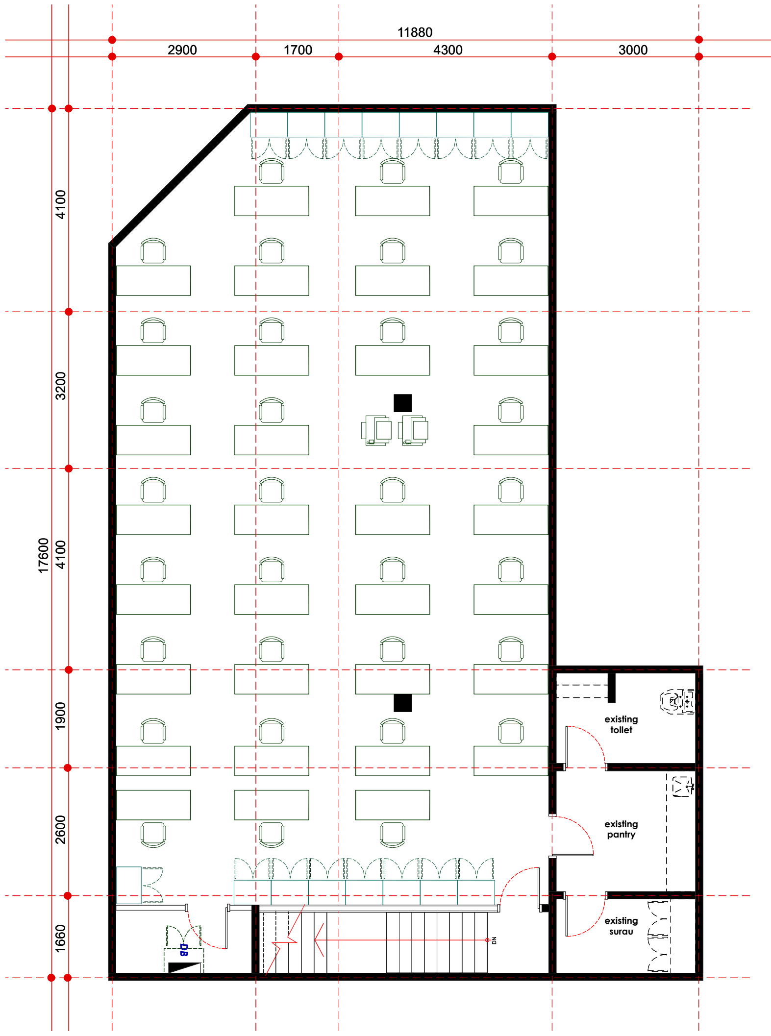
proposed layout plan - first floor scale 1:75
