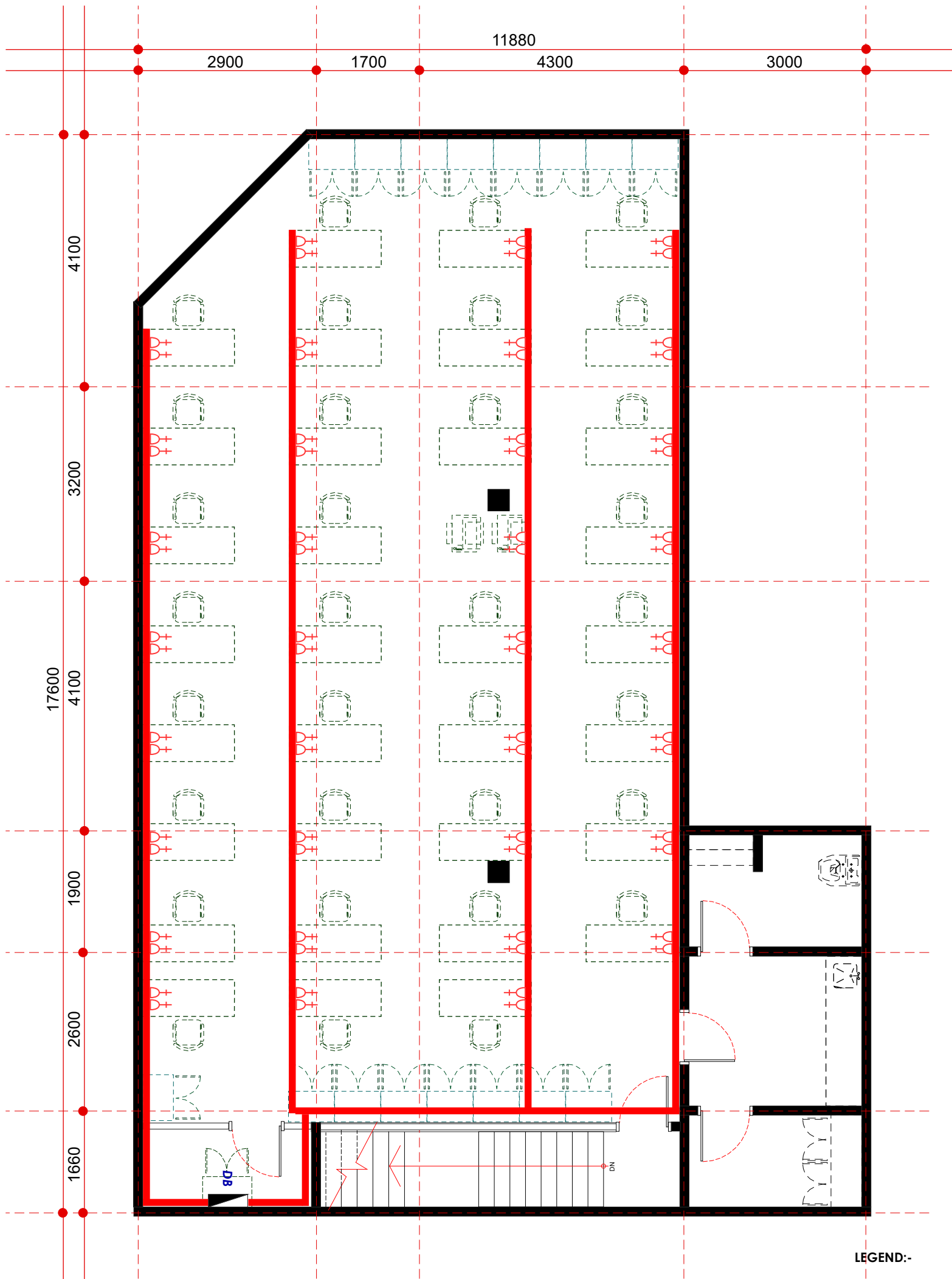
cabling route & SSO point layout plan - first floor scale 1: 75
