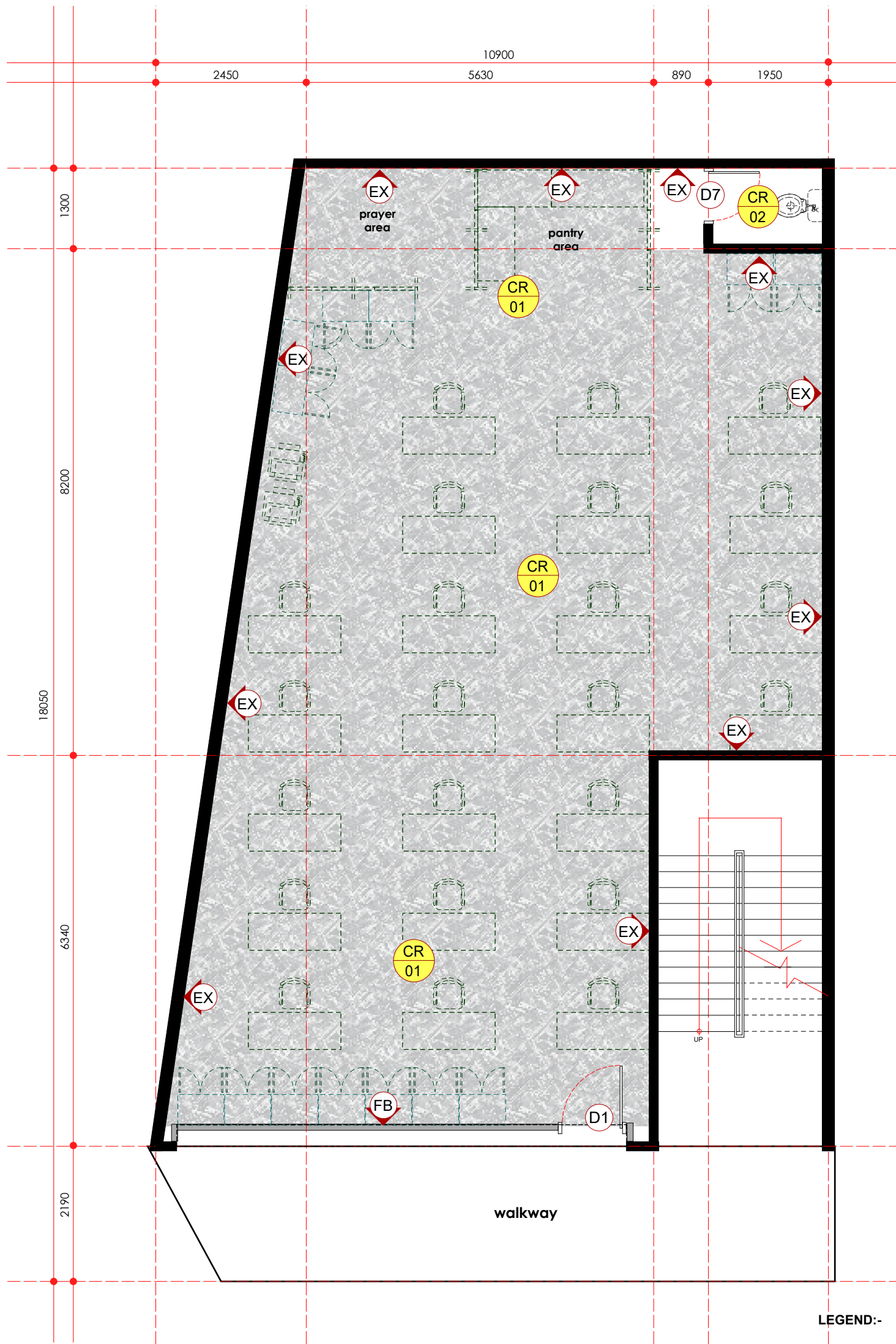
finishing layout plan - first floor scale 1: 75
