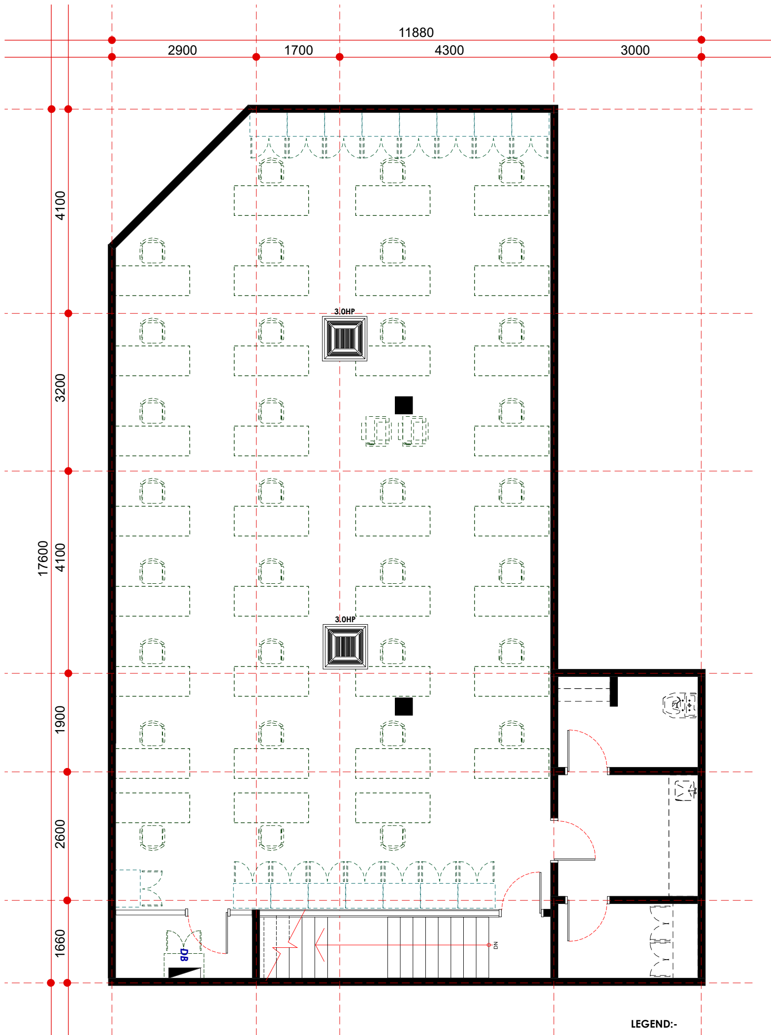
mechanical point layout plan - first floor scale 1: 75
