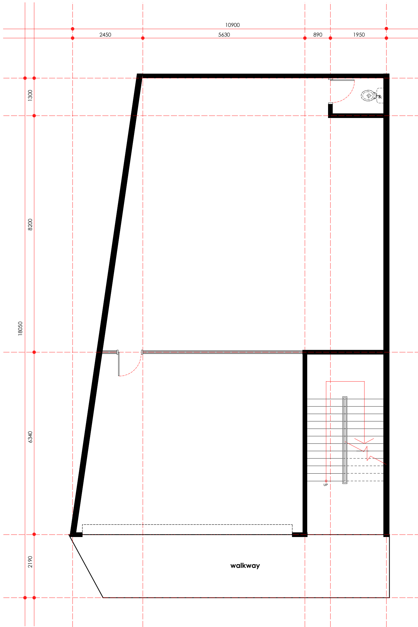
existing layout plan - first floor scale 1:75
