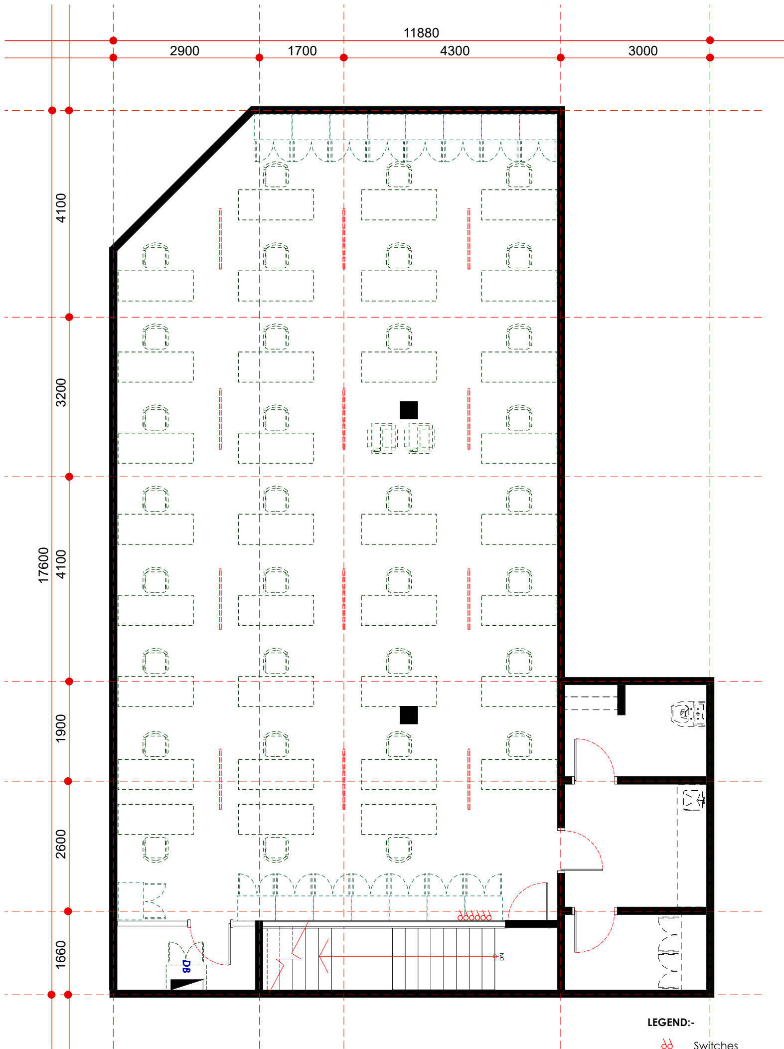
electrical point layout plan - first floor scale 1: 75
