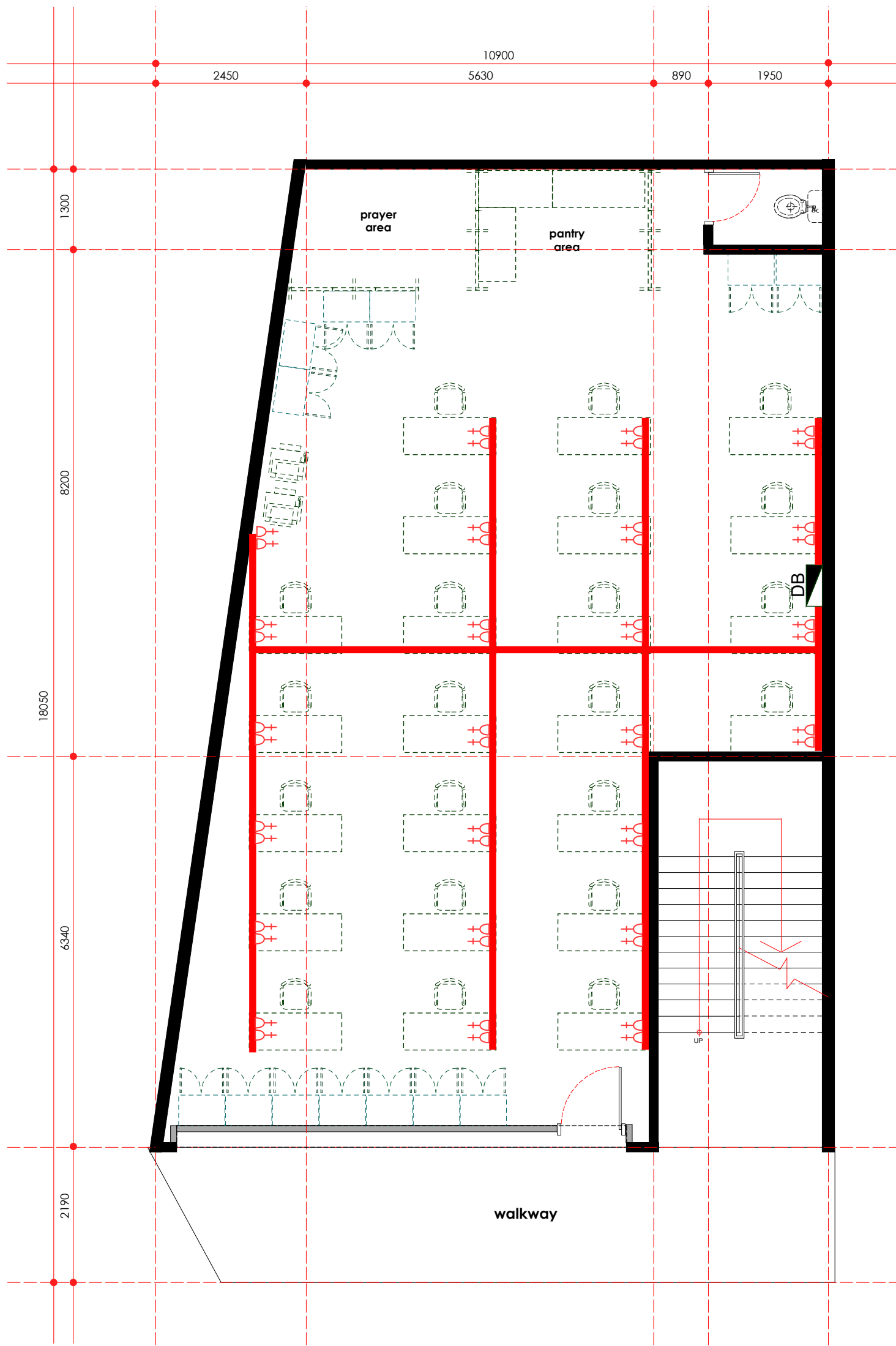
cabling route & SSO point layout plan - first floor scale 1: 75
