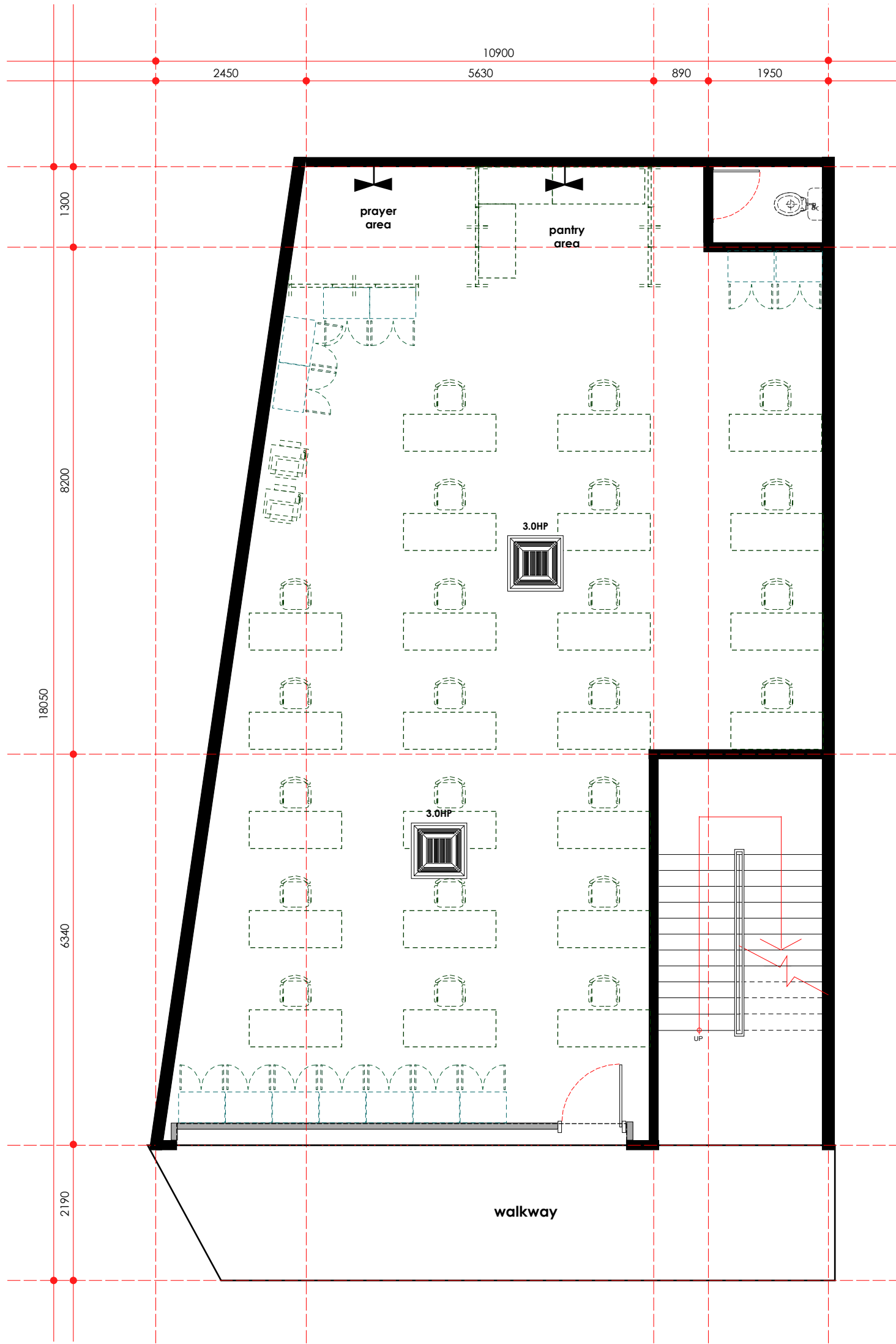
mechanical point layout plan - first floor scale 1: 75
