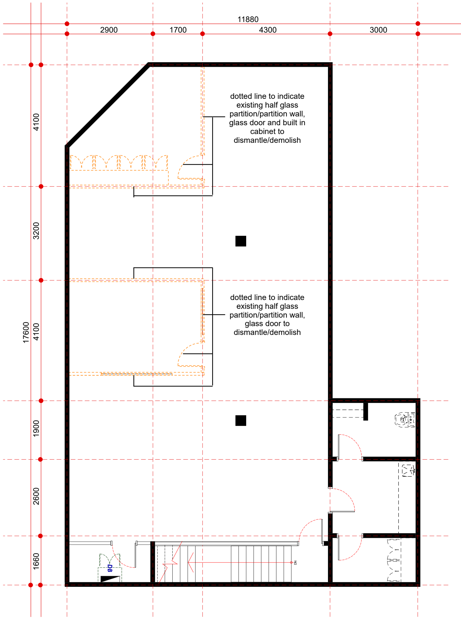
existing layout plan - first floor scale 1:75
