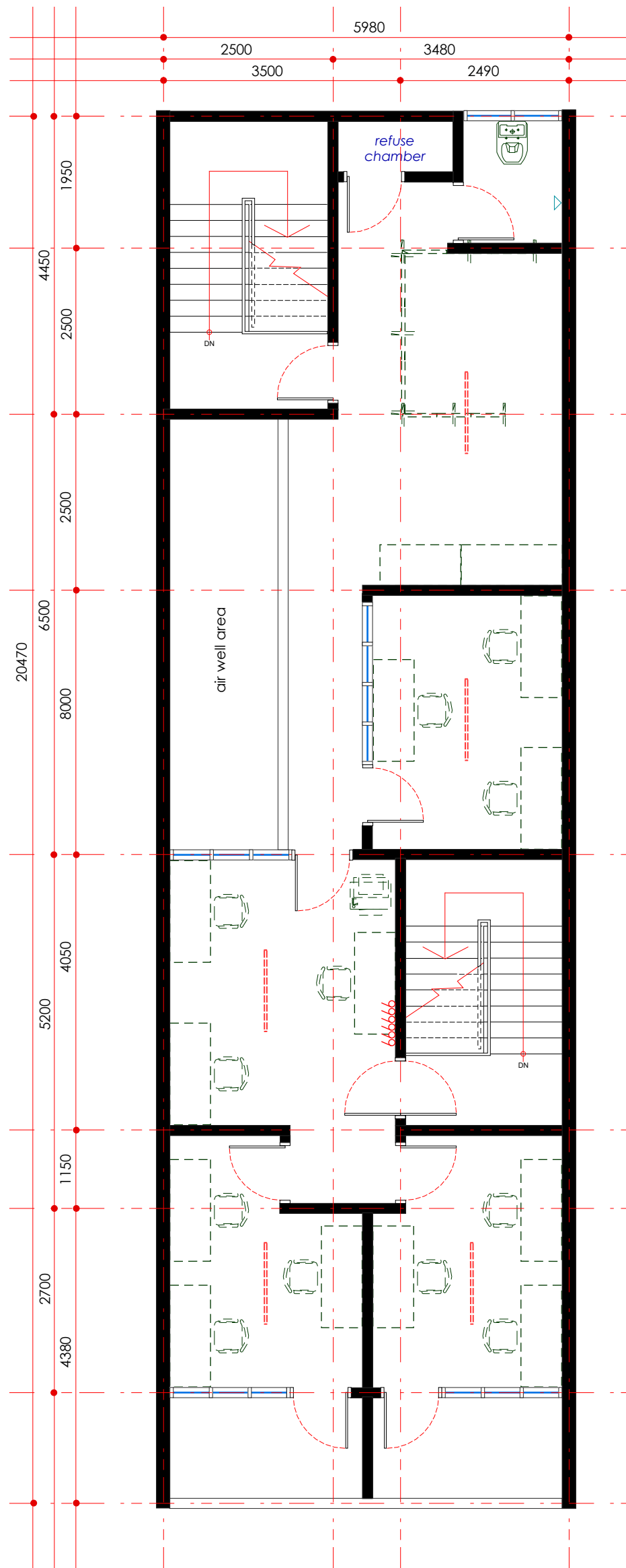
electrical layout plan - second floor scale 1: 75
