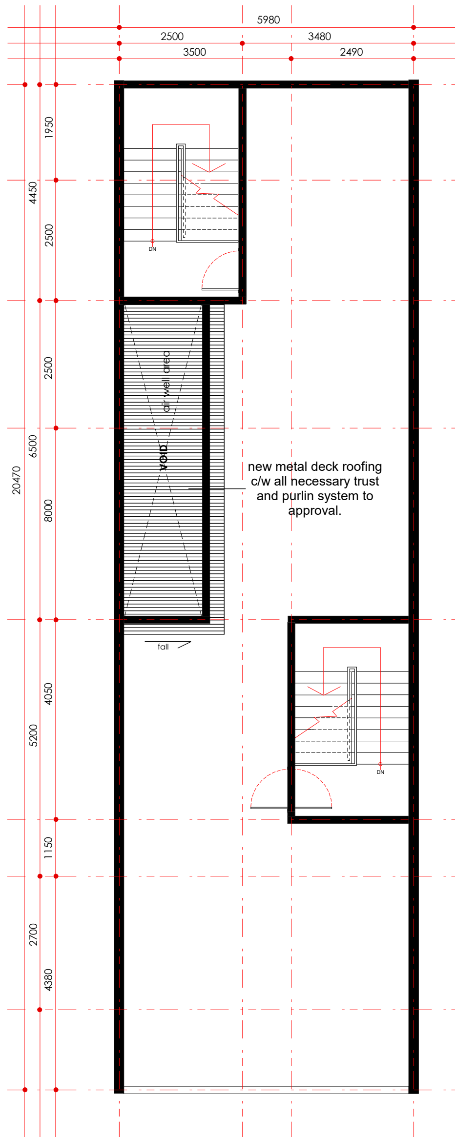
roof layout plan - second floor scale 1: 75
