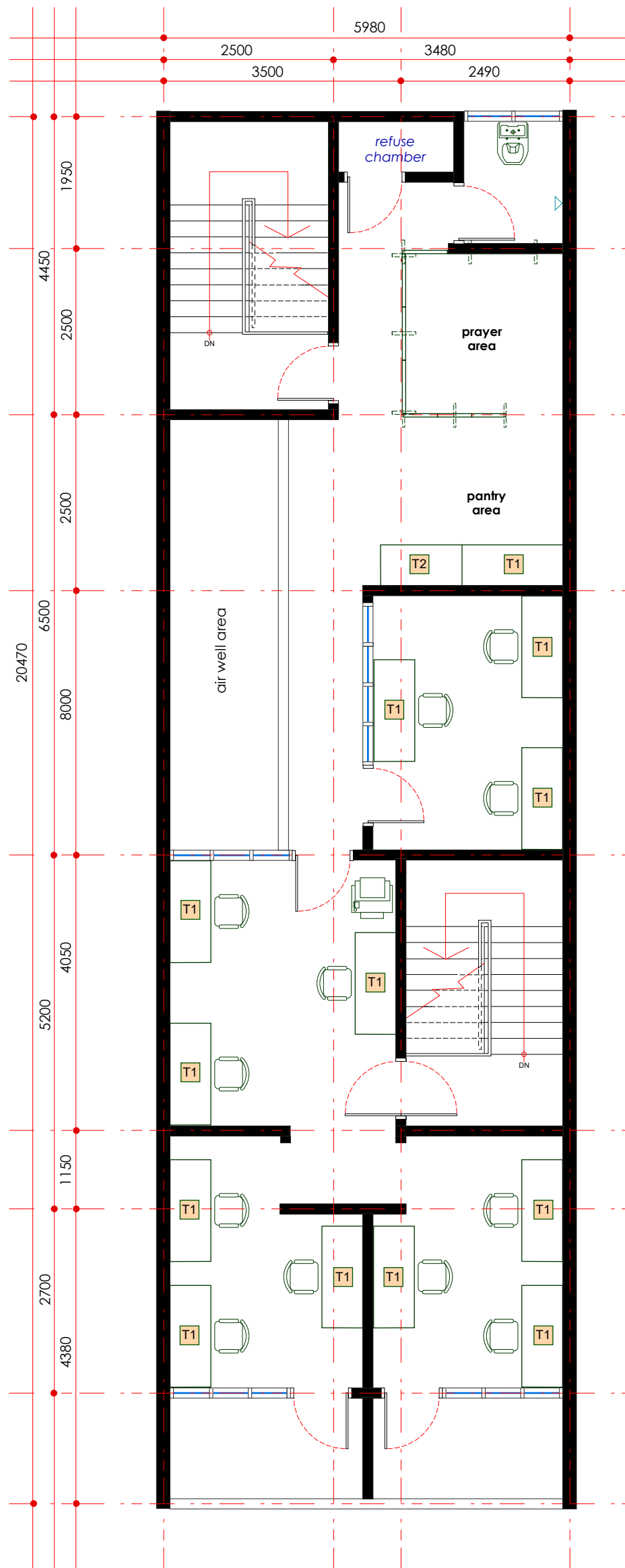
furniture layout plan - second floor scale 1: 75
