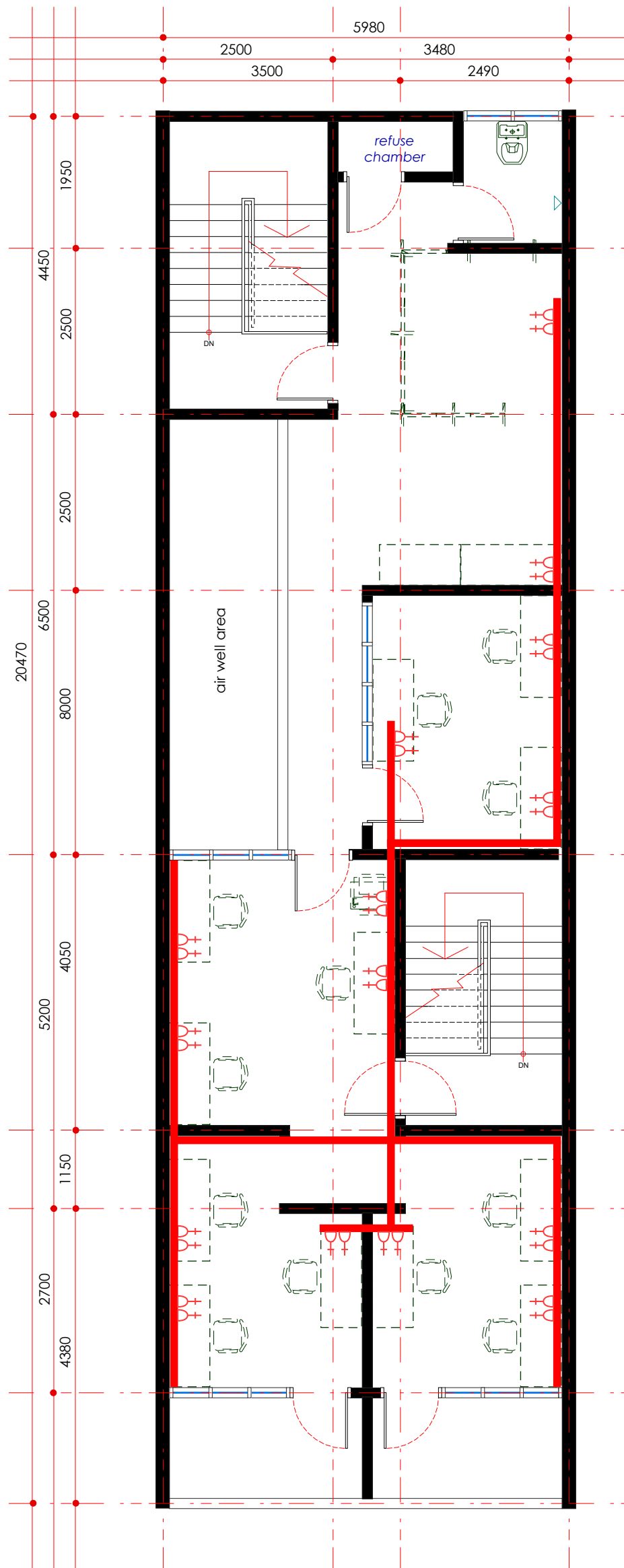
cabling route & SSO point layout plan - second floor scale 1: 75
