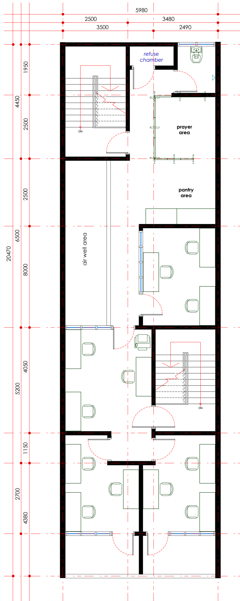
proposed layout plan - second floor scale 1: 75
