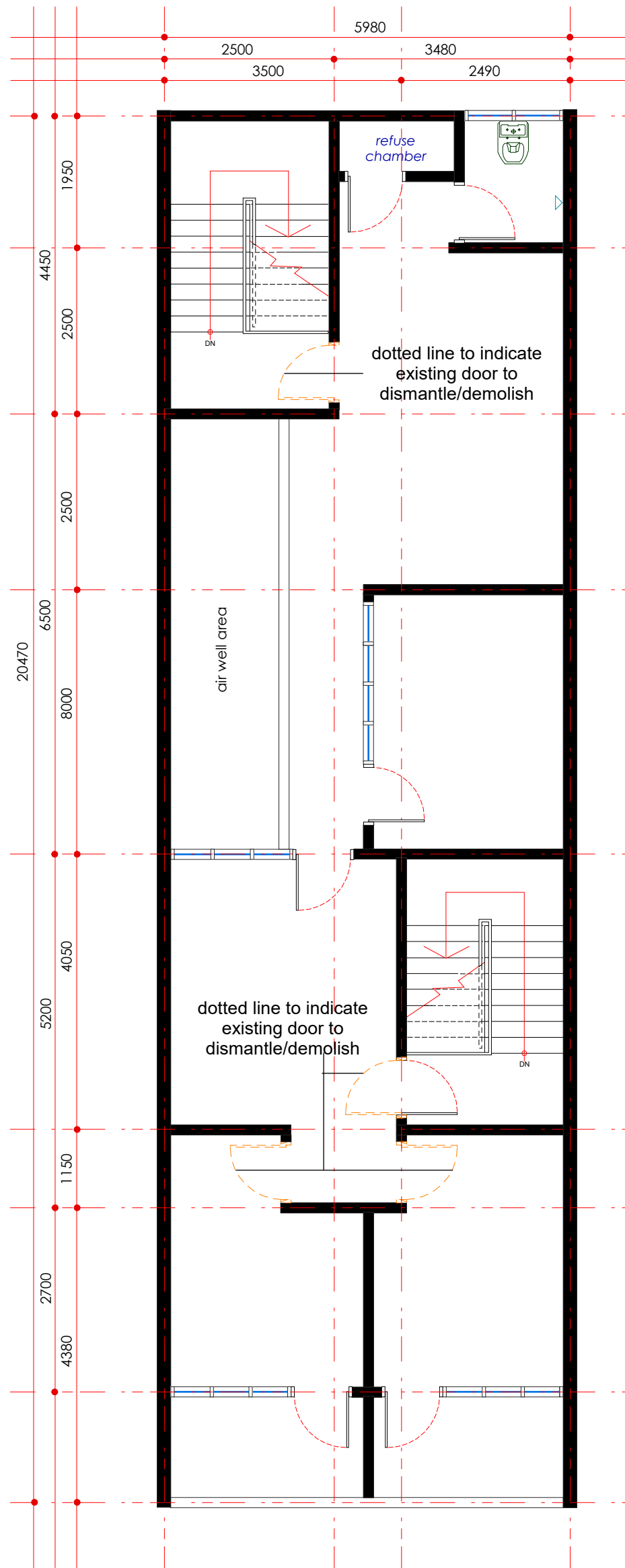
existing layout plan - second floor scale 1: 75
