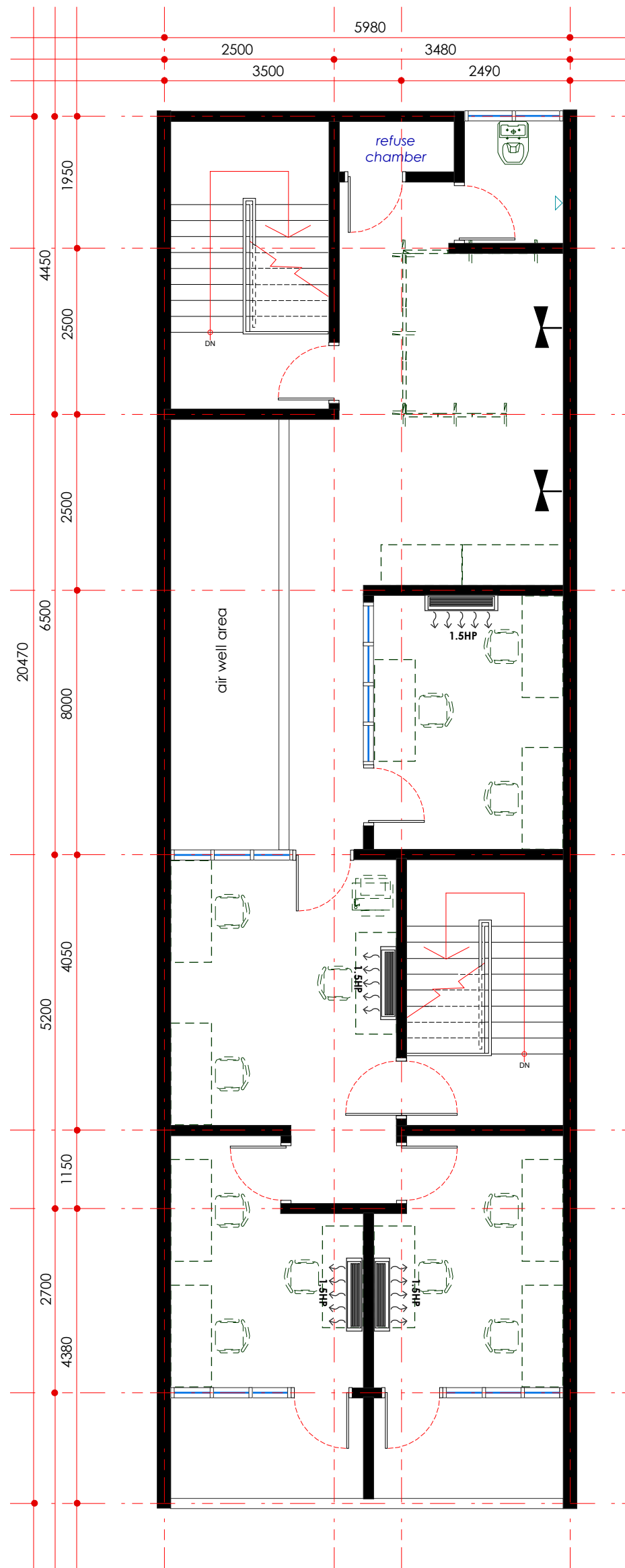
mechanical layout plan - second floor scale 1: 75
