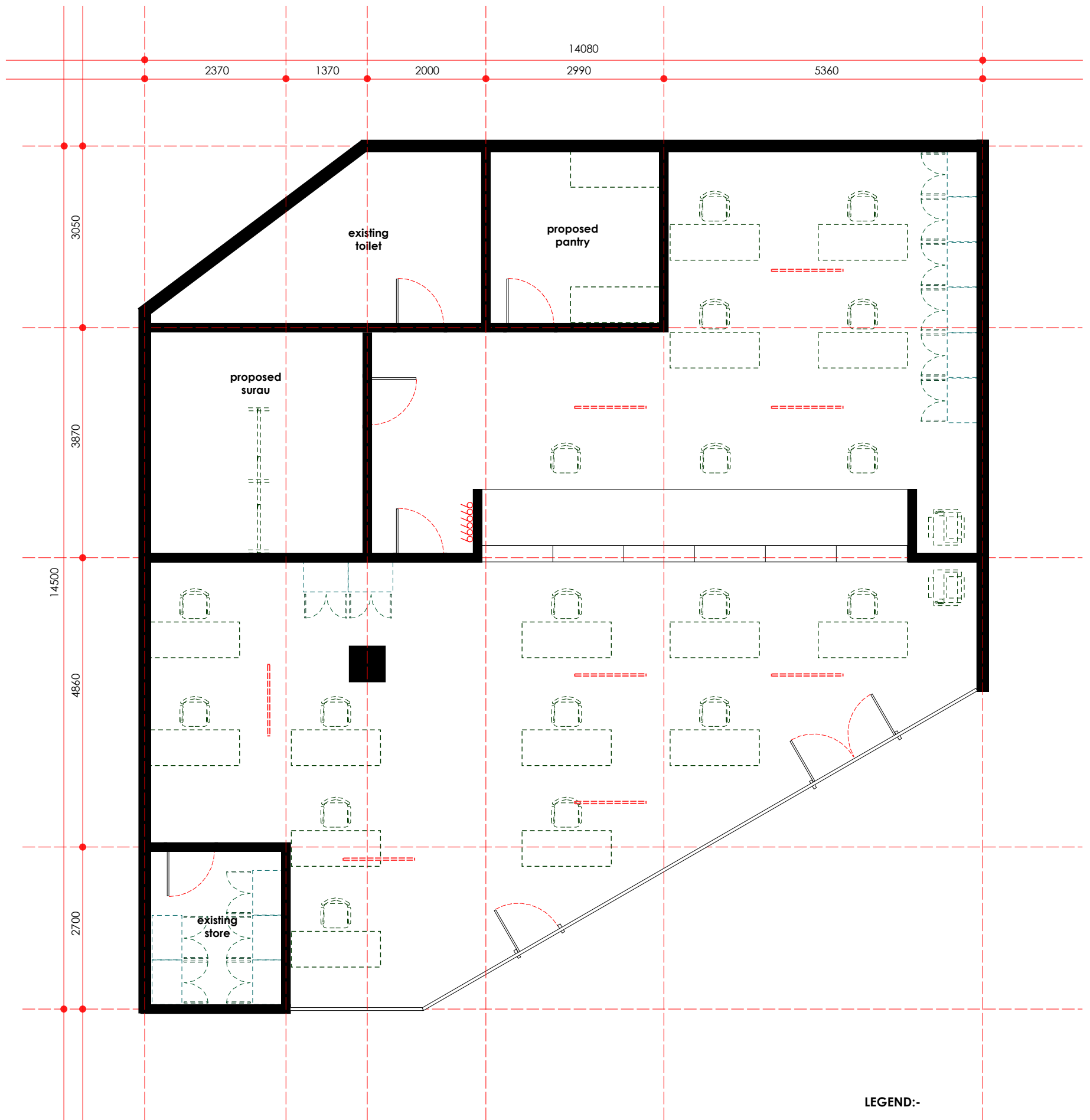
electrical point layout plan - ground floor scale 1: 75
