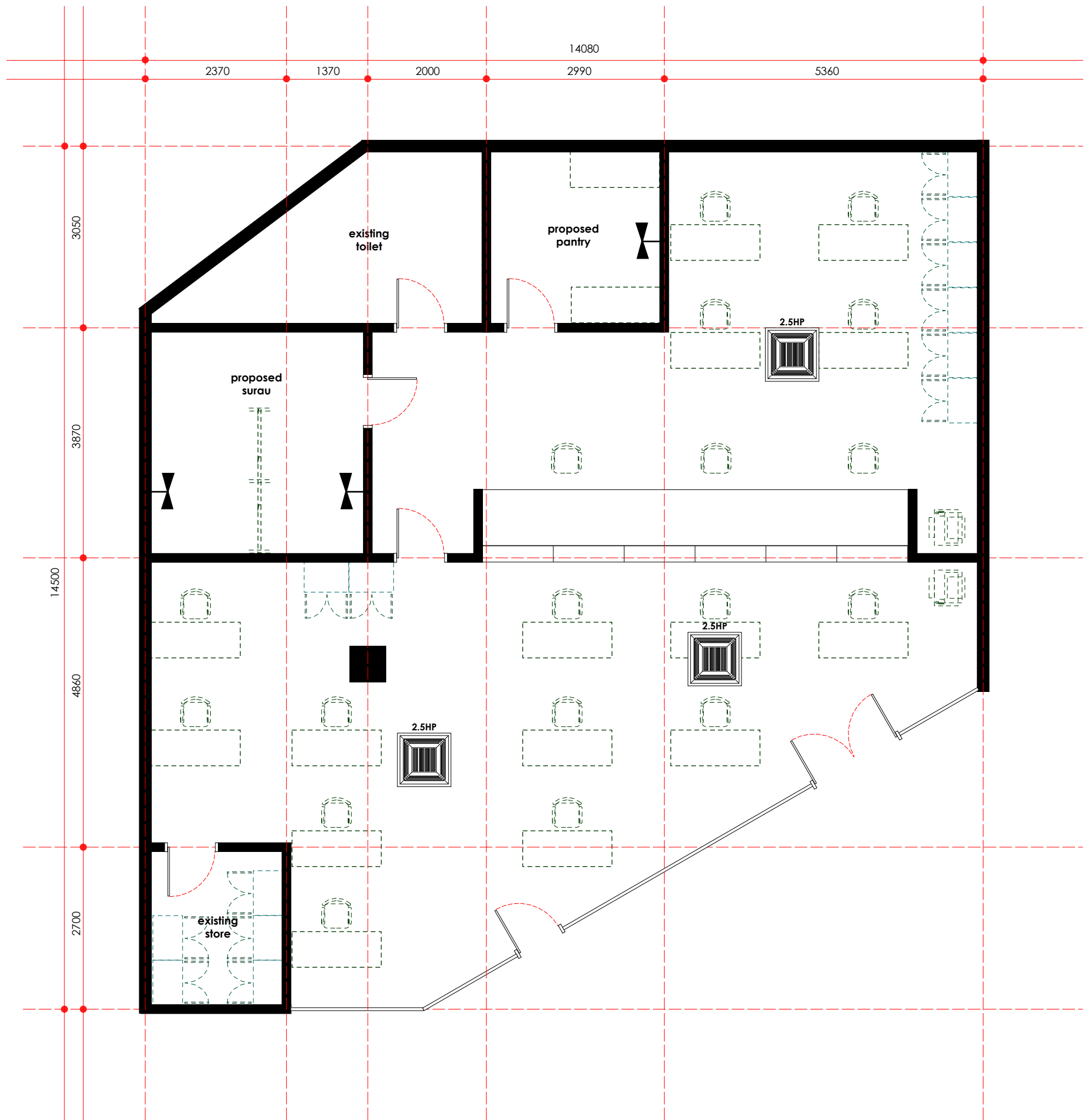
mechanical point layout plan - ground floor scale 1: 75
