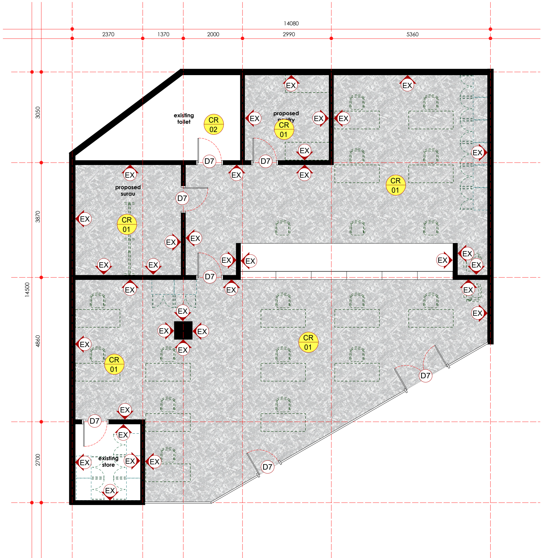
finishing layout plan - ground floor scale 1: 75
