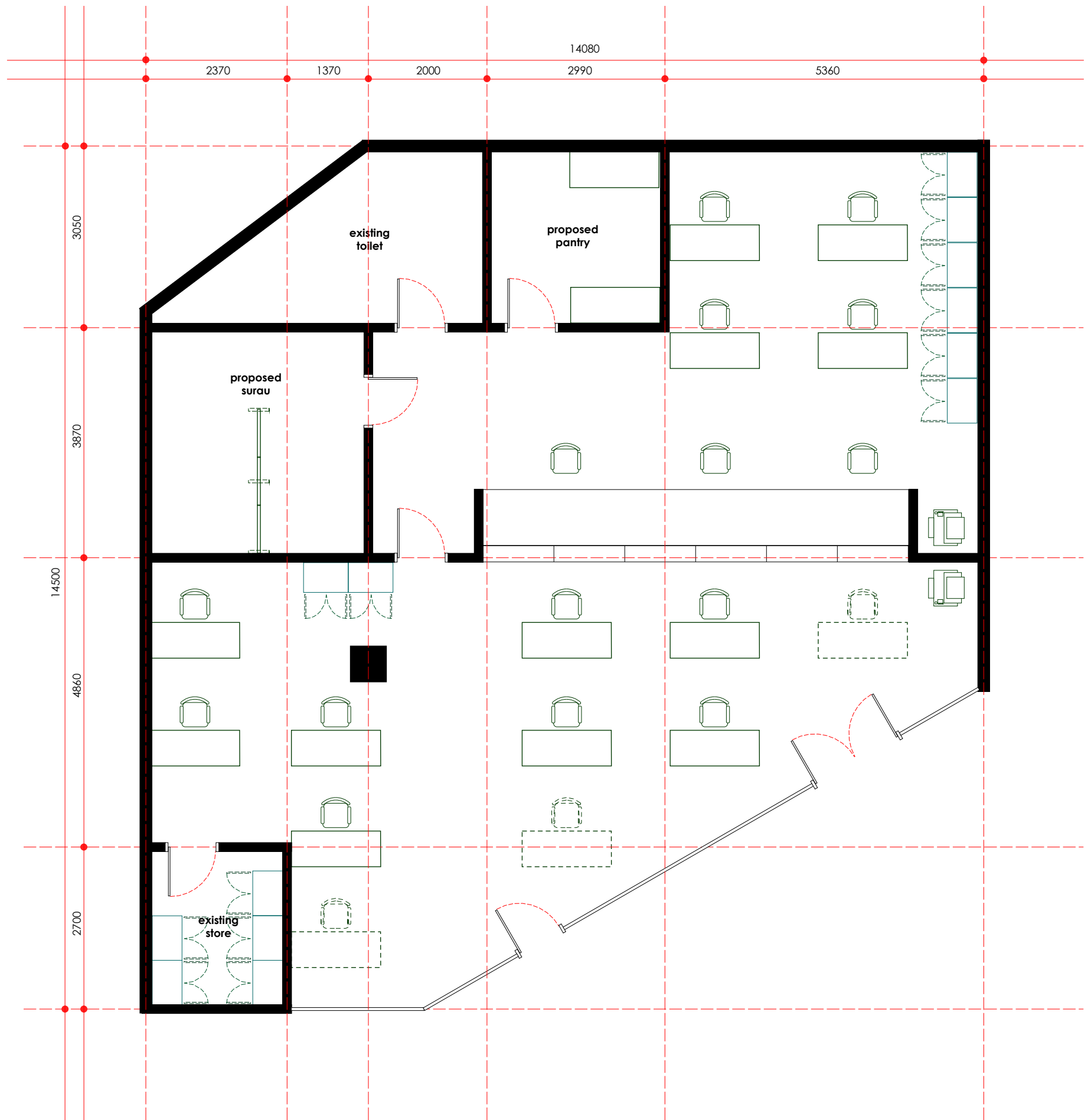
proposed layout plan - ground floor scale 1: 75
