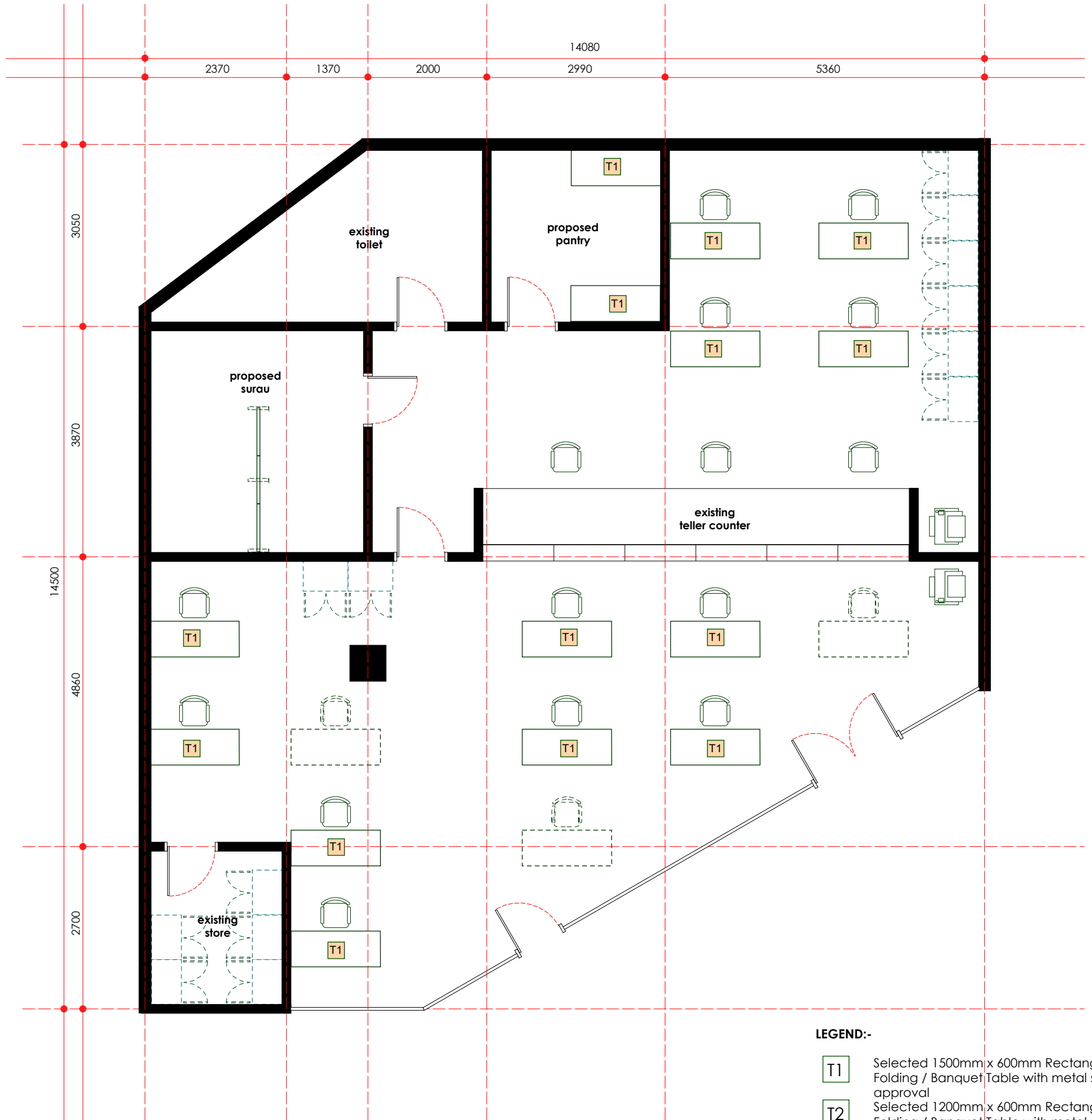
furniture layout plan - ground floor scale 1: 75
