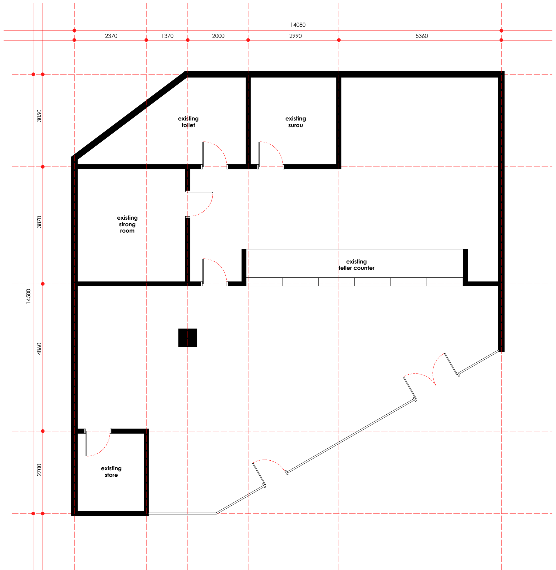
existing layout plan - ground floor scale 1: 75
