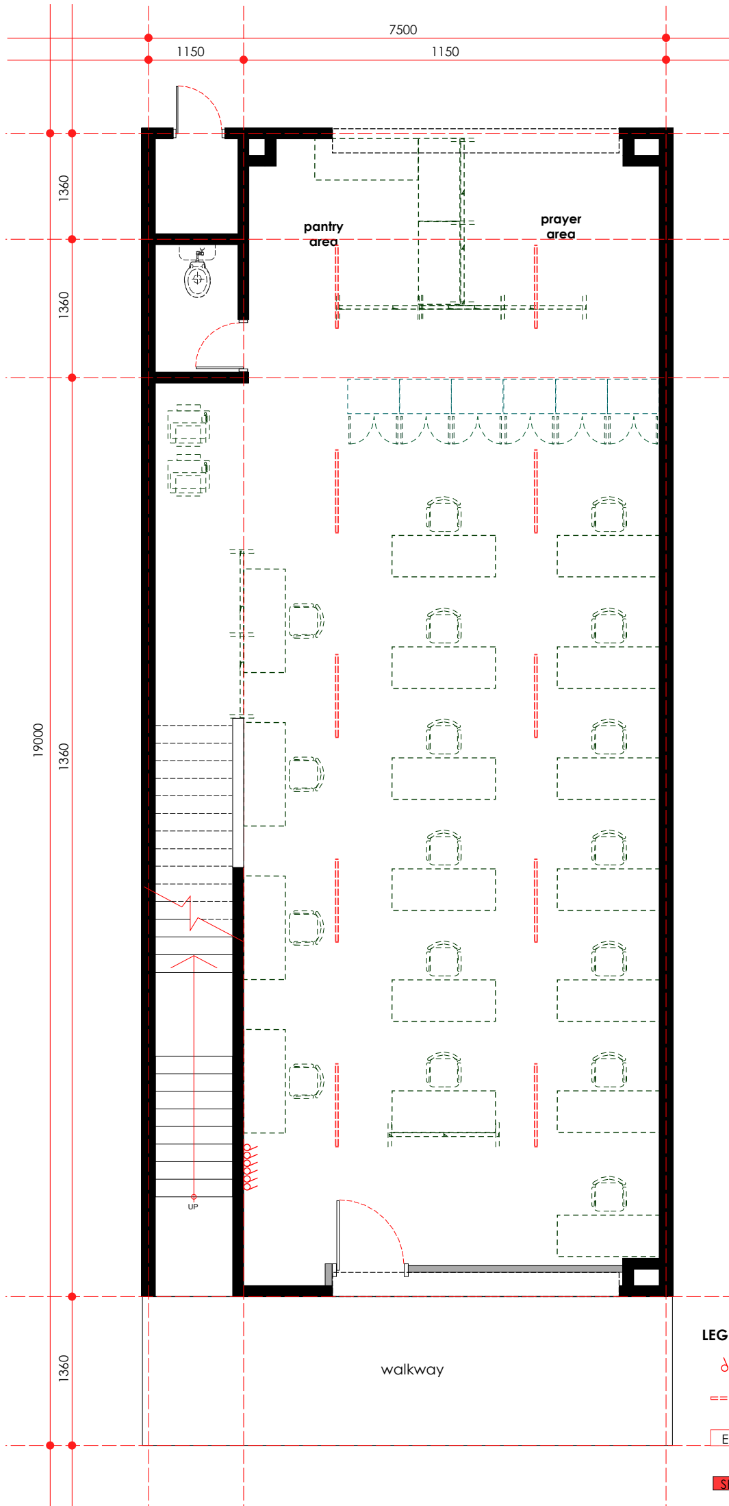
electrical point layout plan - ground floor scale 1: 75
