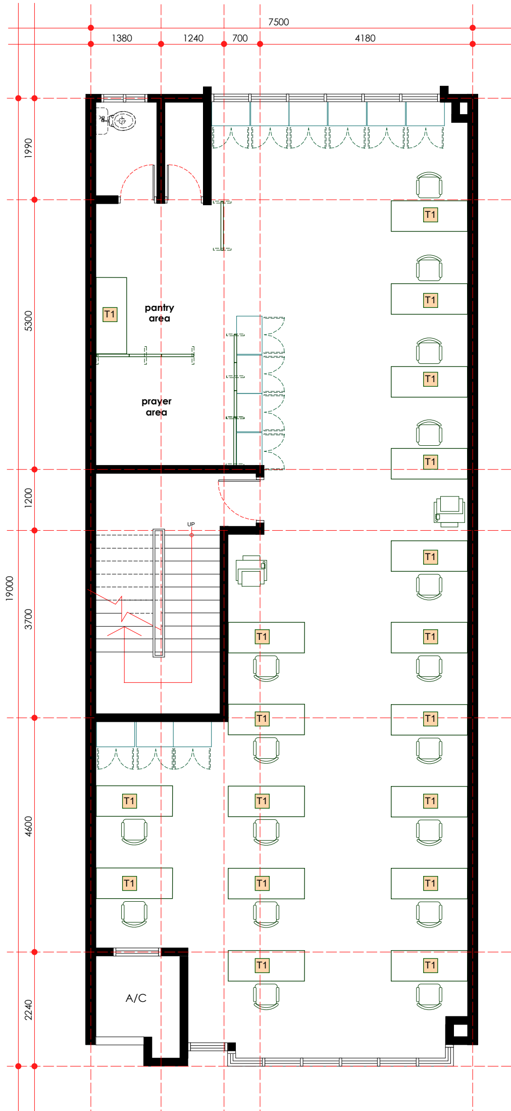
furniture layout plan - first floor scale 1: 75
