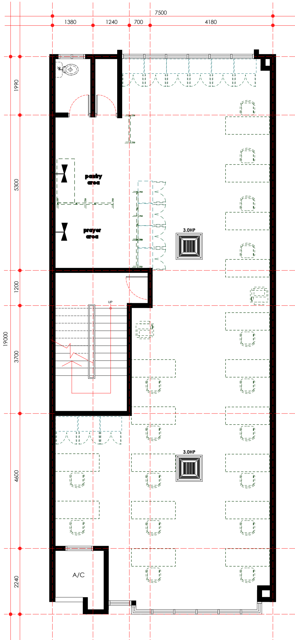
mechanical point layout plan - first floor scale 1: 75
