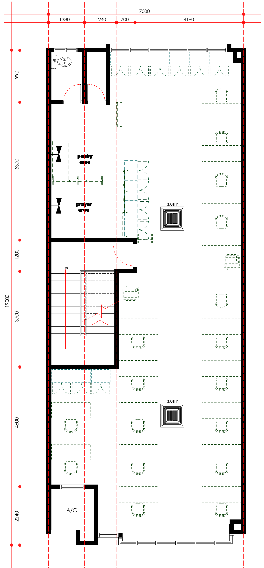
mechanical point layout plan - second floor scale 1: 75
