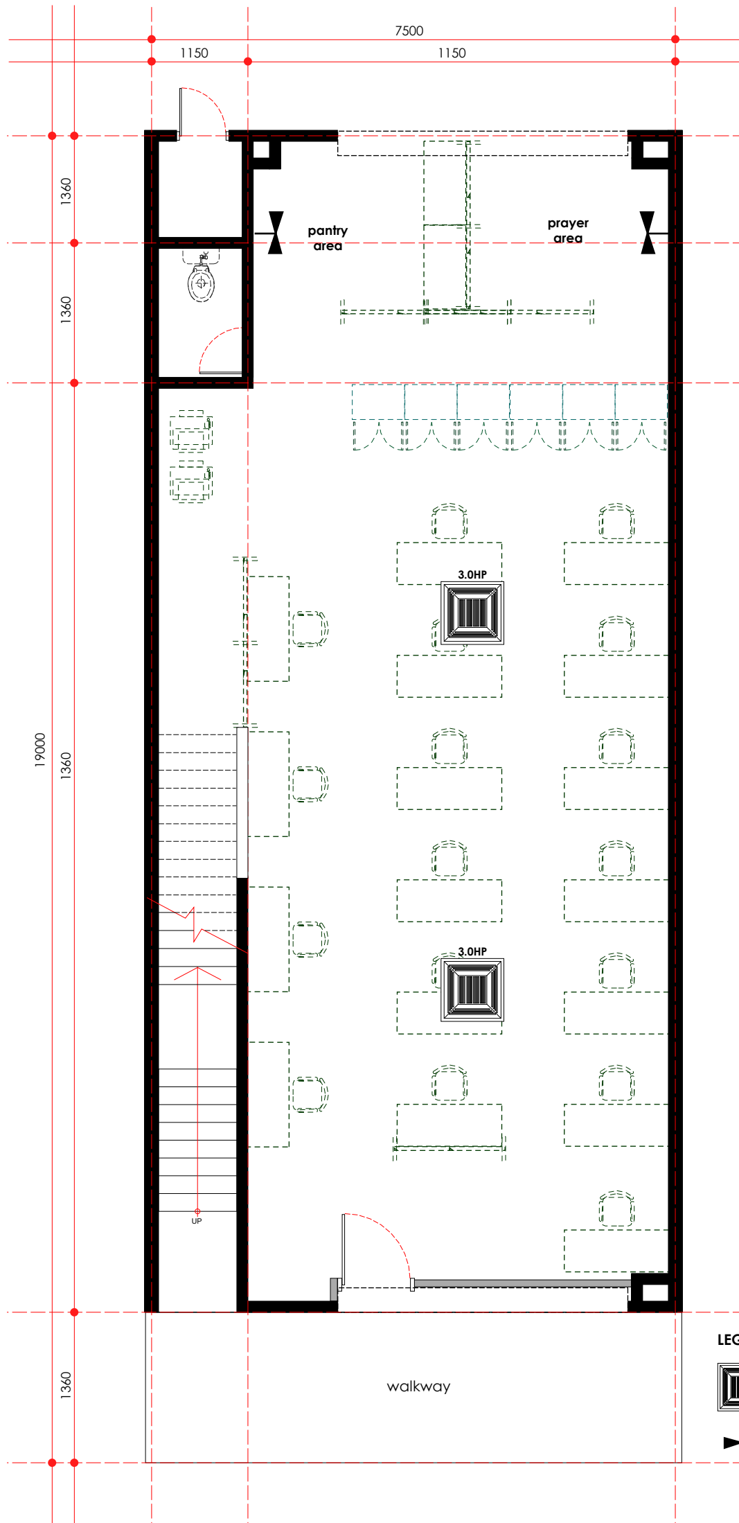
mechanical point layout plan - ground floor scale 1: 75
