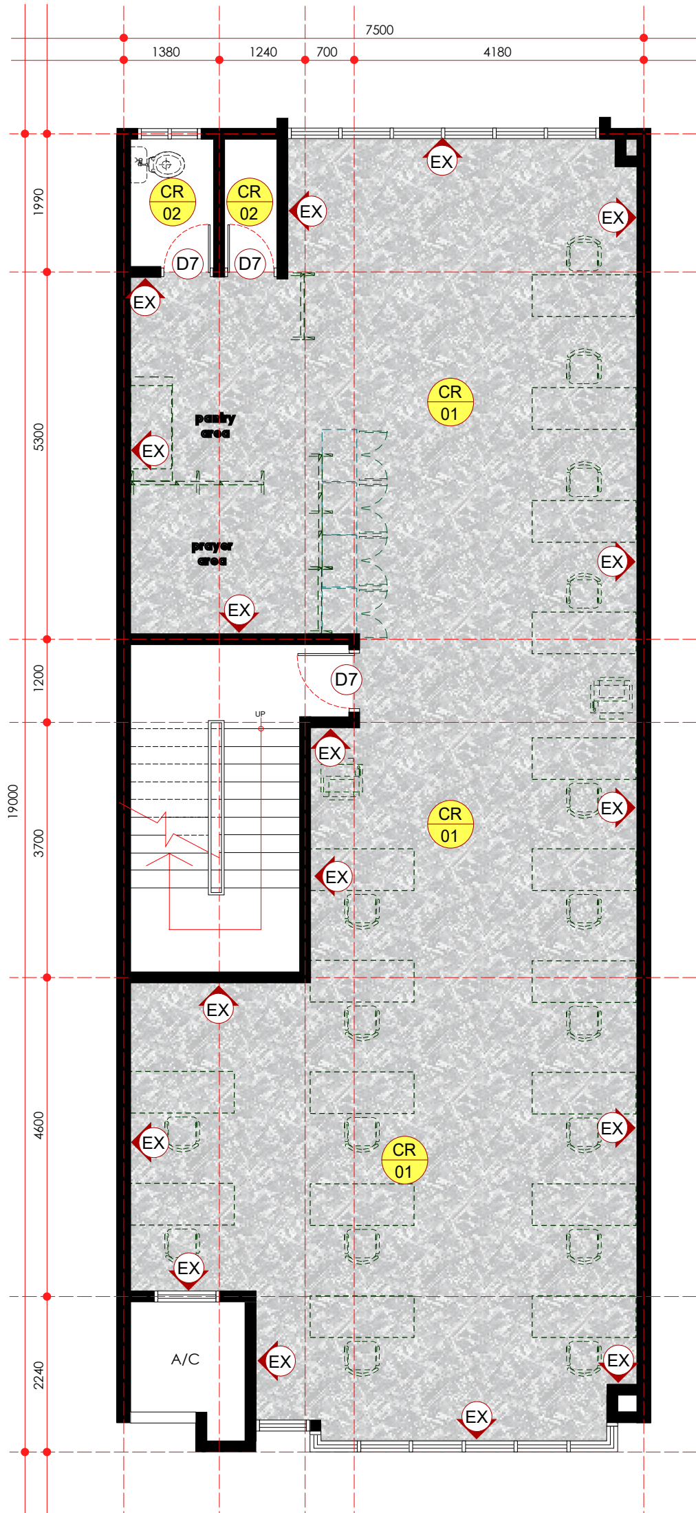
finishing layout plan - first floor scale 1: 75
