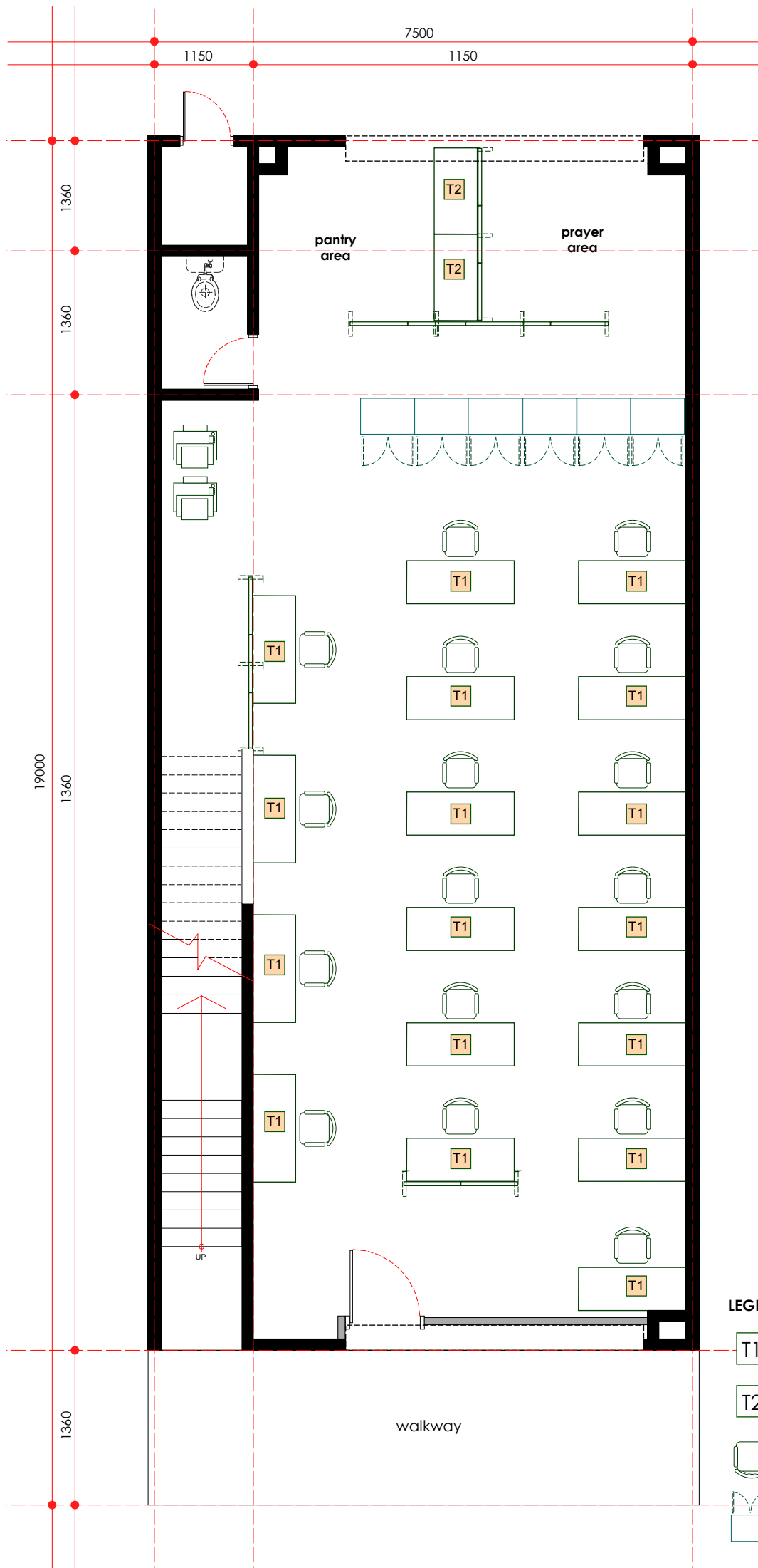
furniture layout plan - ground floor scale 1: 75
