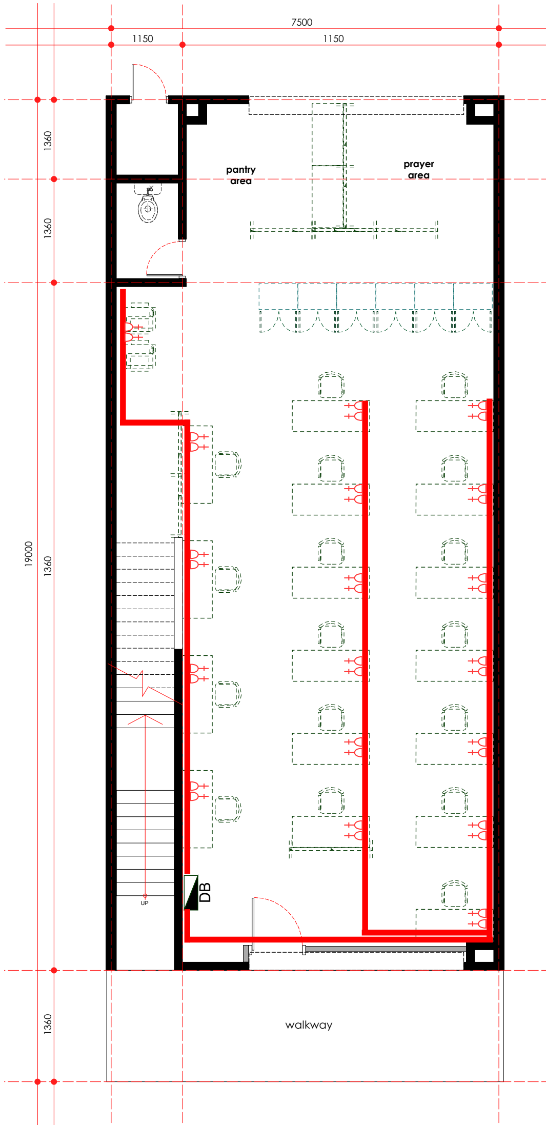
cabling route & SSO point layout plan - ground floor scale 1: 75
