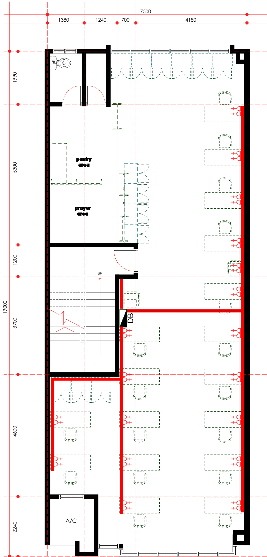
cabling route & SSO point layout plan - first floor scale 1: 75
