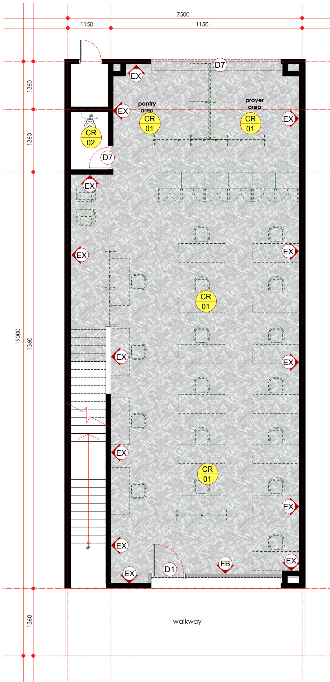
finishing layout plan - ground floor scale 1: 75
