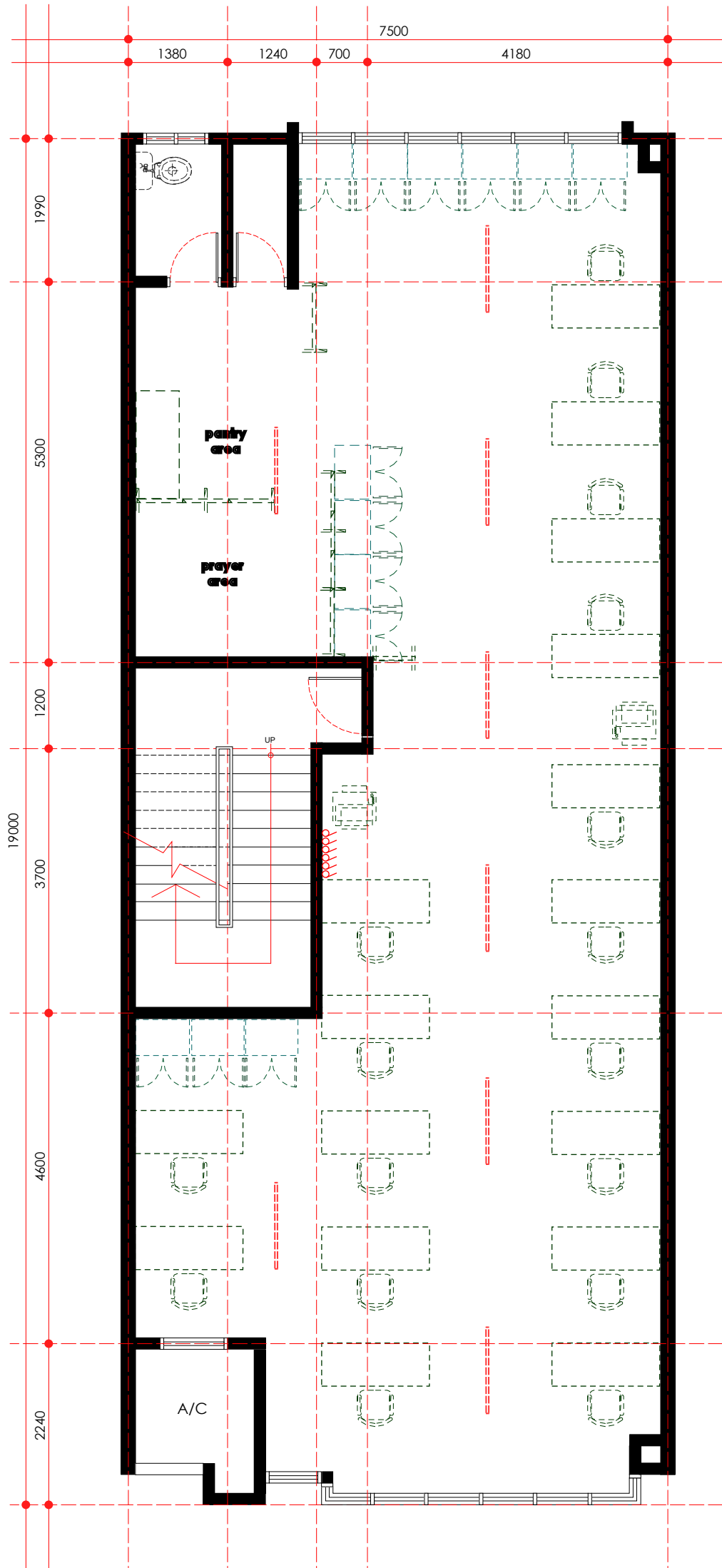
electrical point layout plan - first floor scale 1: 75
