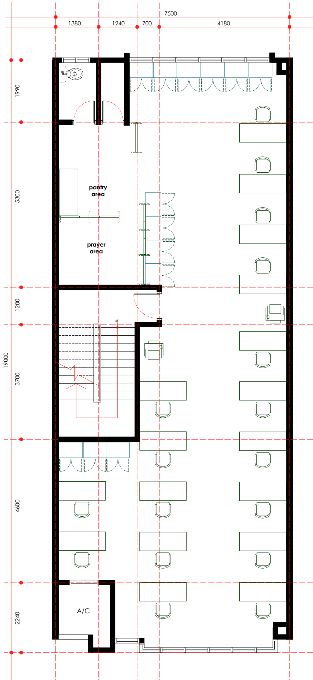
proposed layout plan - first floor scale 1: 75
