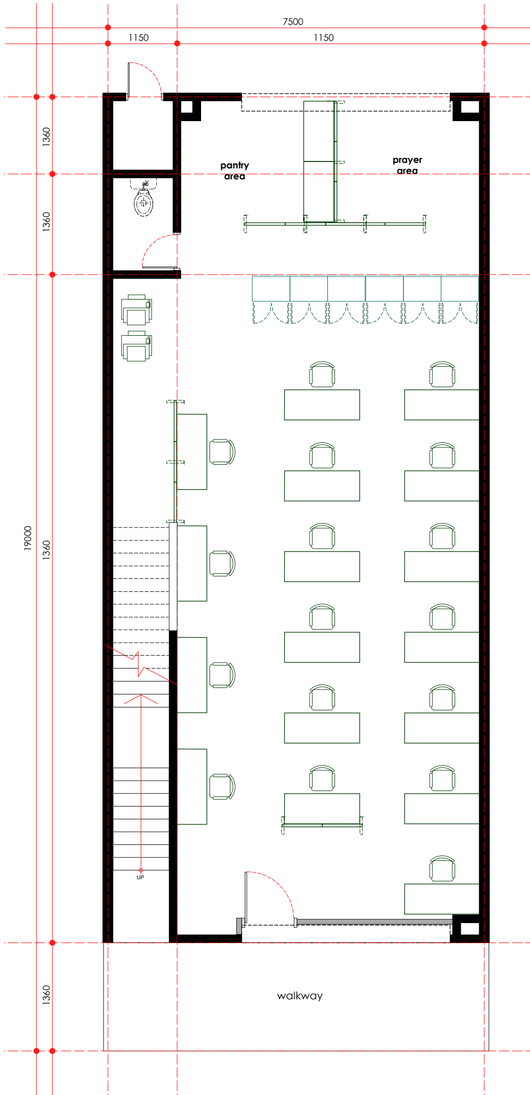
proposed layout plan - ground floor scale 1: 75
