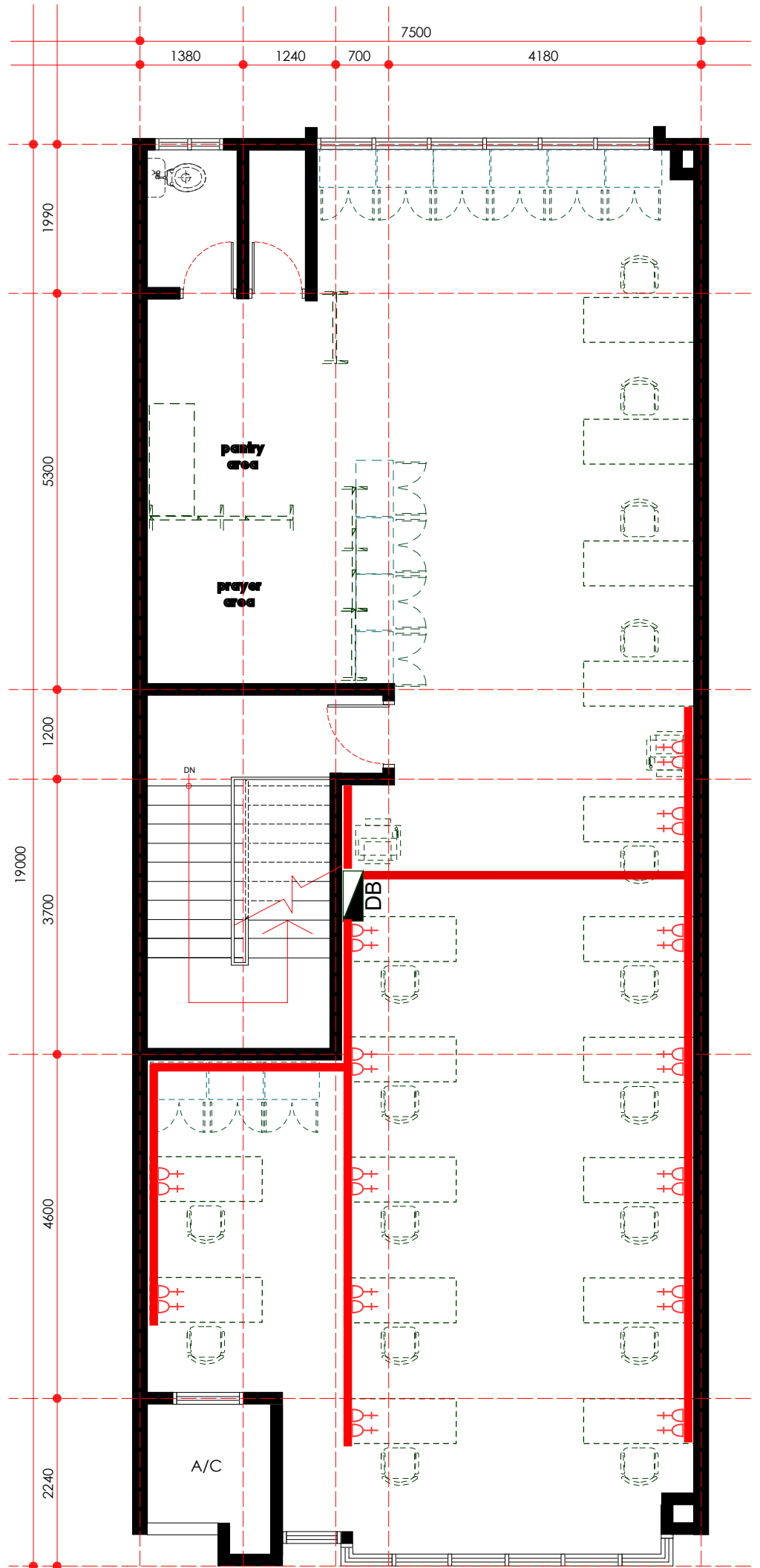
cabling route & SSO point layout plan - second floor scale 1: 75
