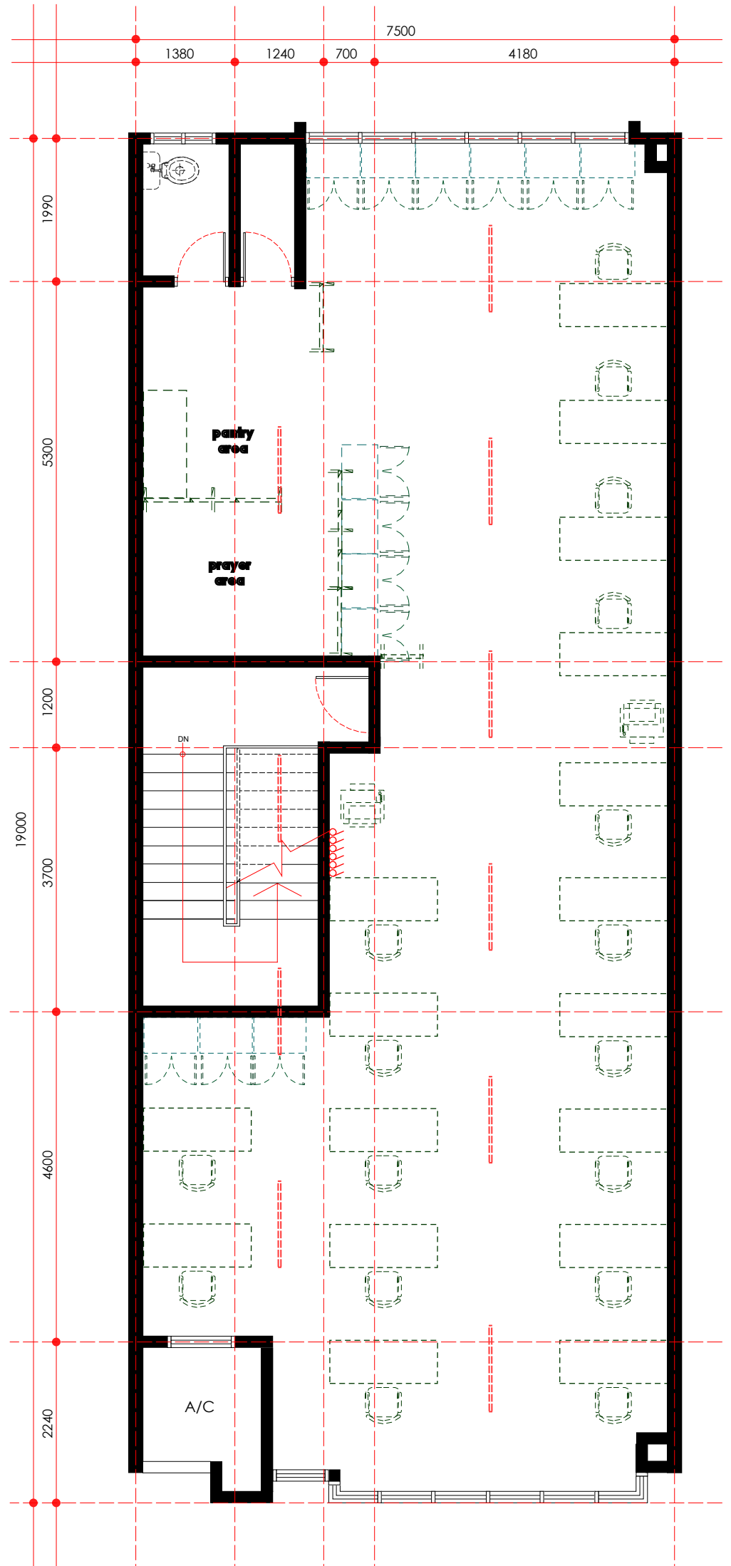
electrical point layout plan - second floor scale 1: 75
