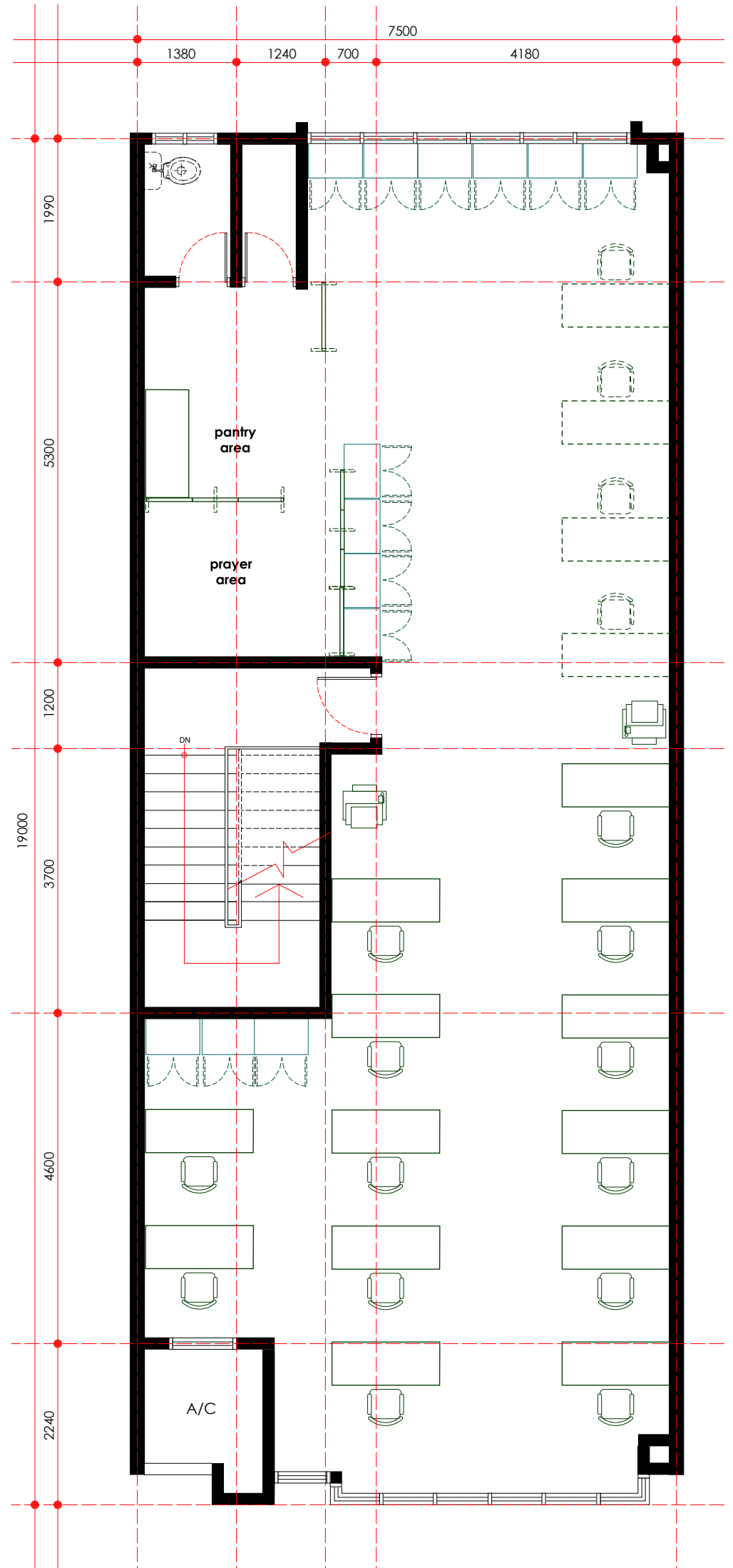
proposed layout plan - second floor scale 1: 75
