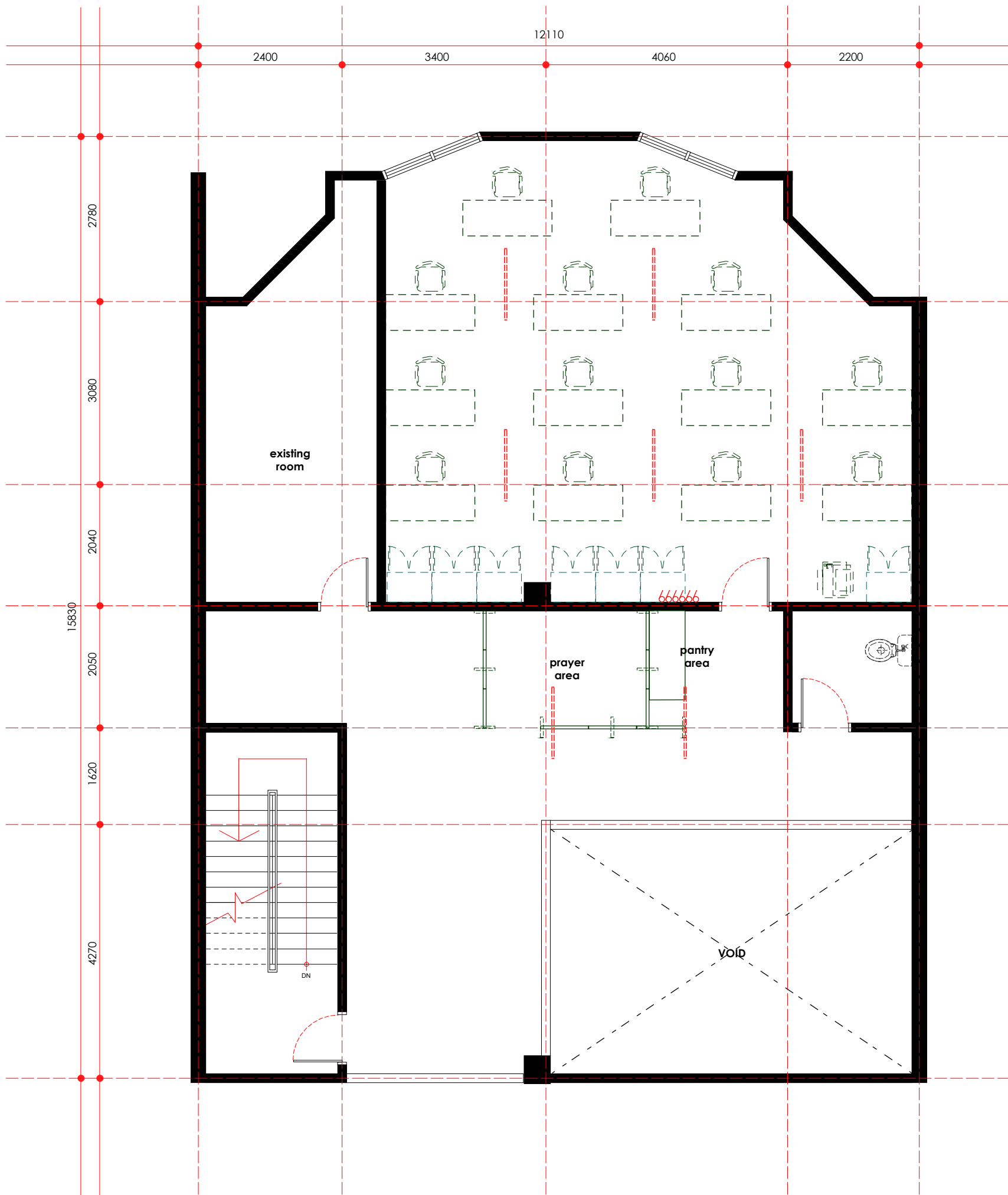
electrical point layout plan - first floor scale 1: 75
