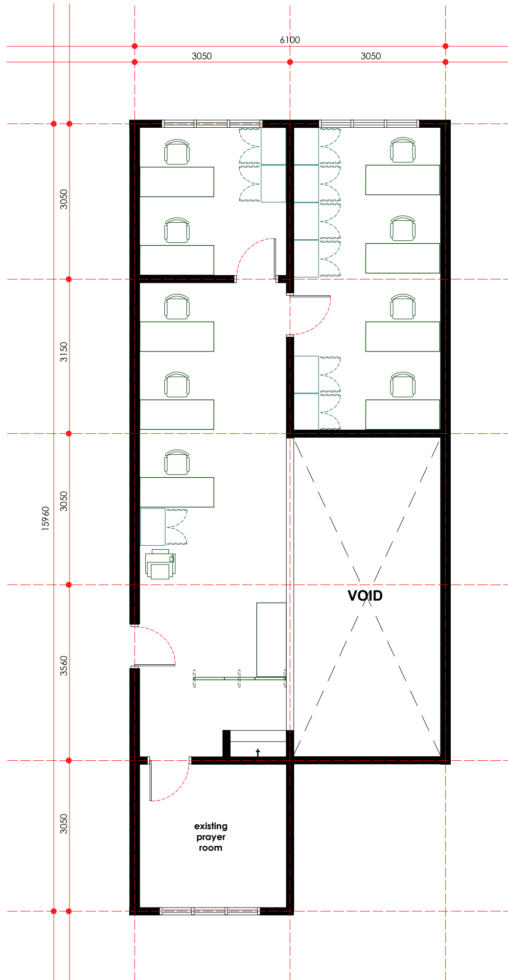
proposed layout plan - first floor scale 1: 75
