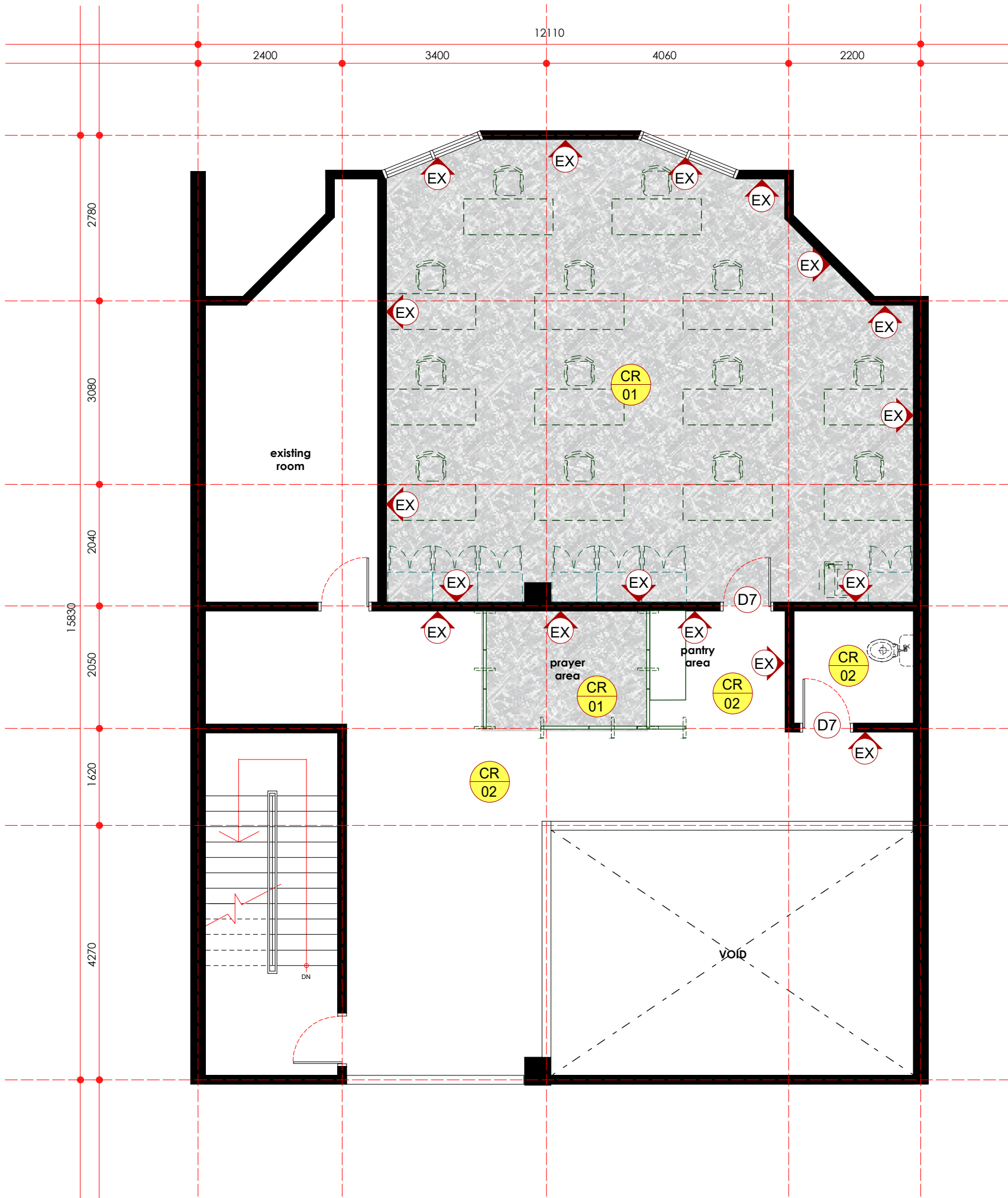
finishing layout plan - first floor scale 1: 75
