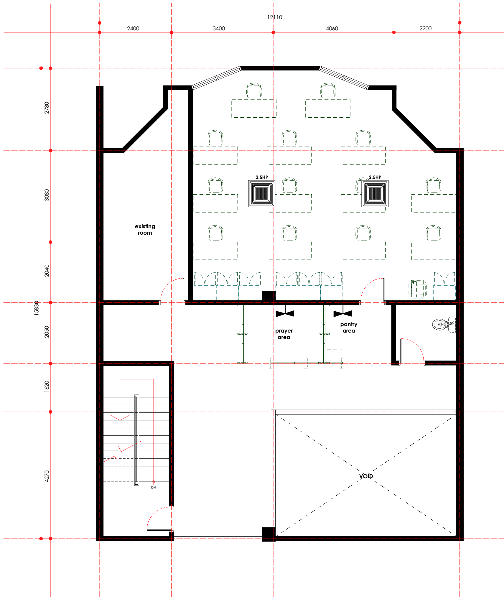
mechanical point layout plan - first floor scale 1: 75
