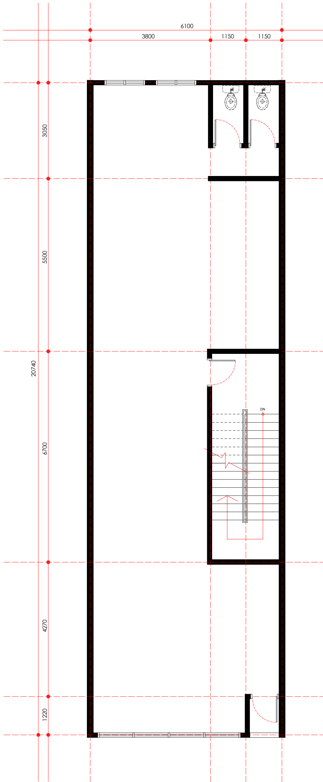
existing layout plan - first floor scale 1: 75
