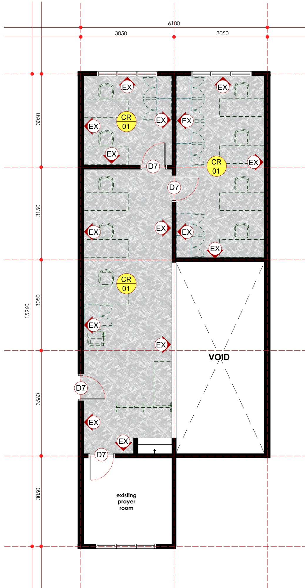
finishing layout plan - first floor scale 1: 75
