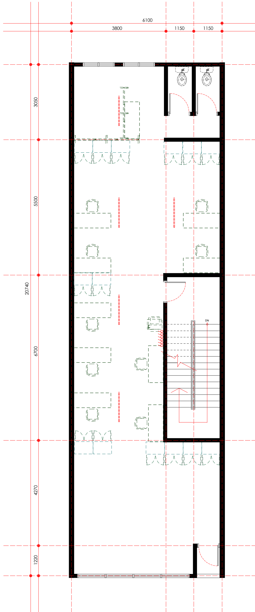
electrical point layout plan - first floor scale 1: 75
