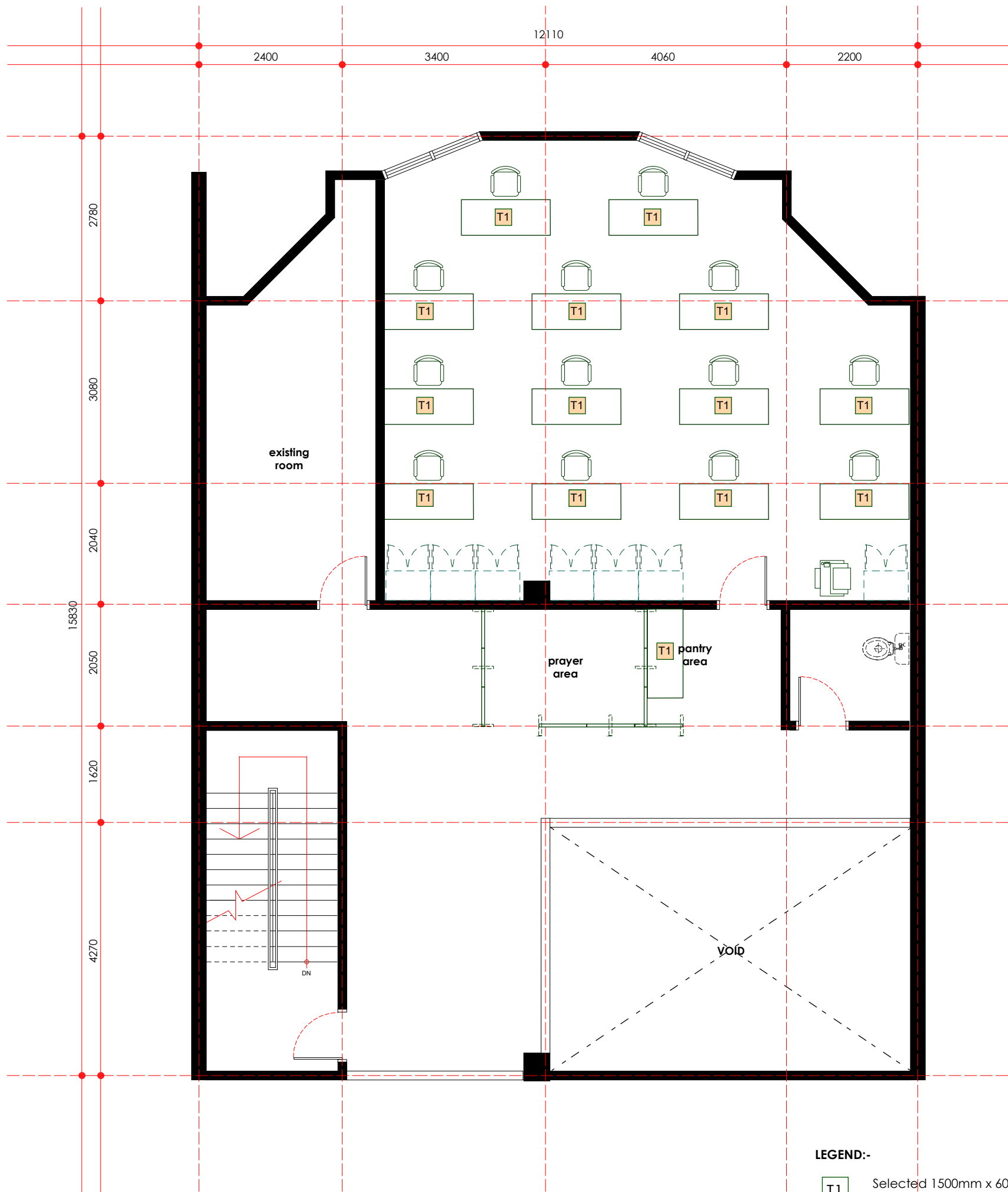
furniture layout plan - first floor scale 1:75
