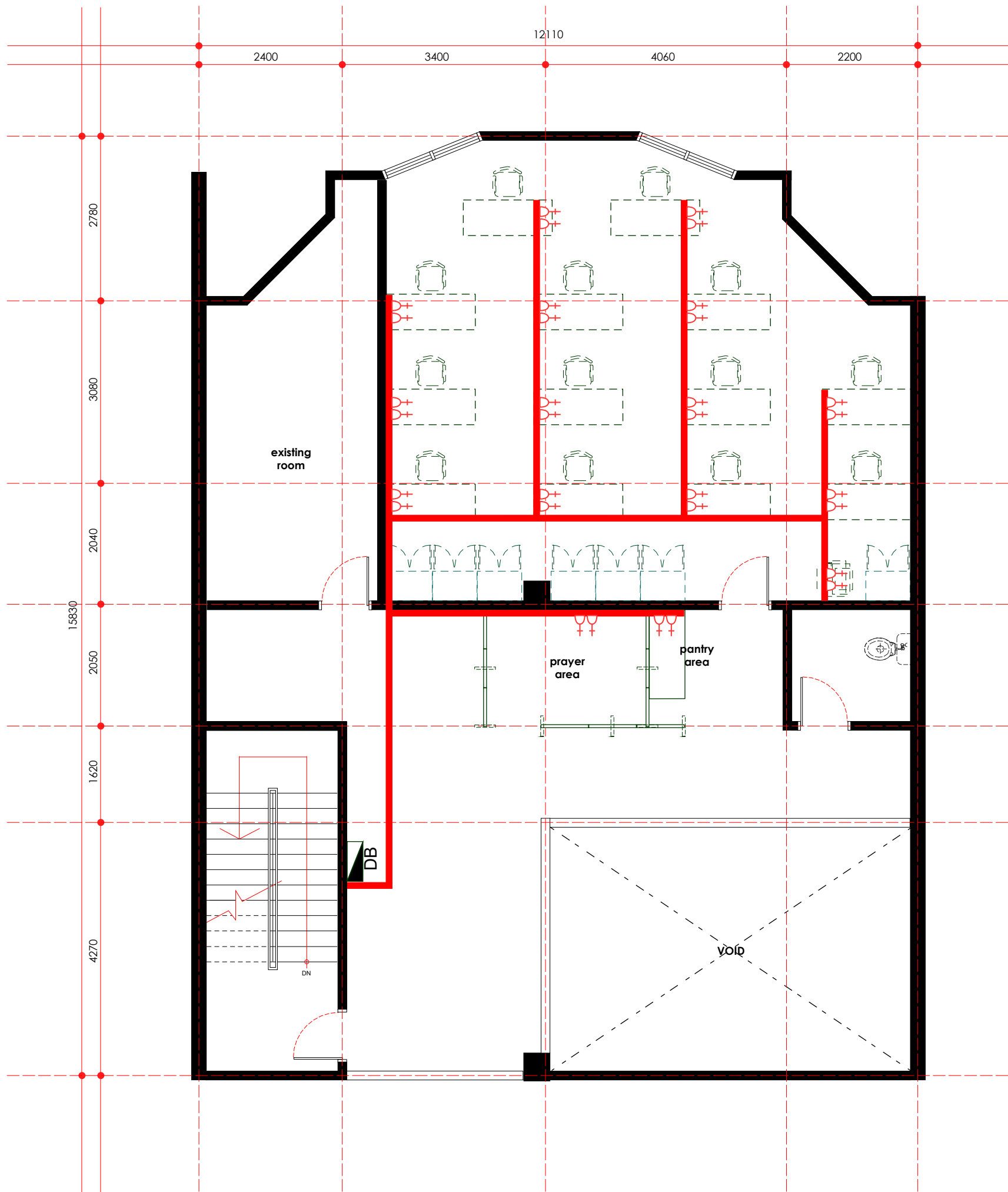
cabling route & SSO point layout plan - first floor scale 1: 75
