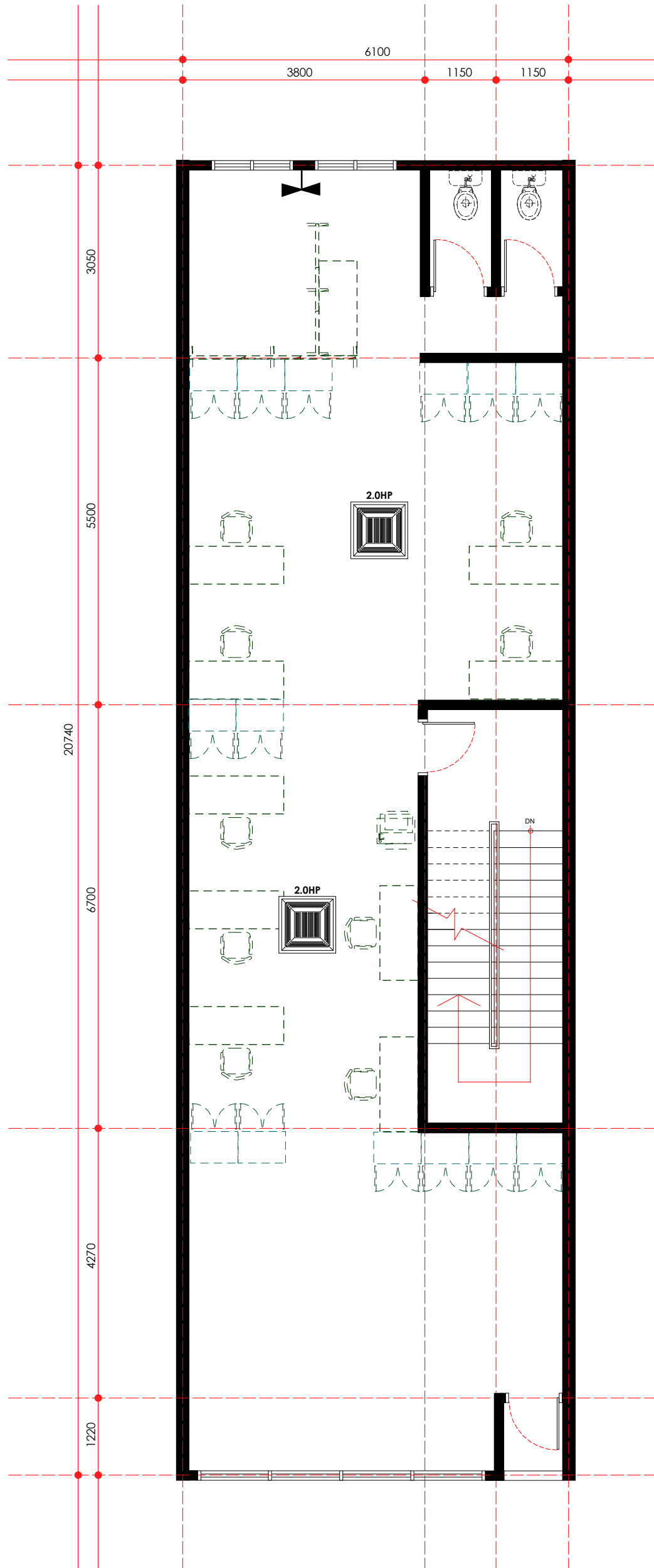
mechanical point layout plan - first floor scale 1: 75
