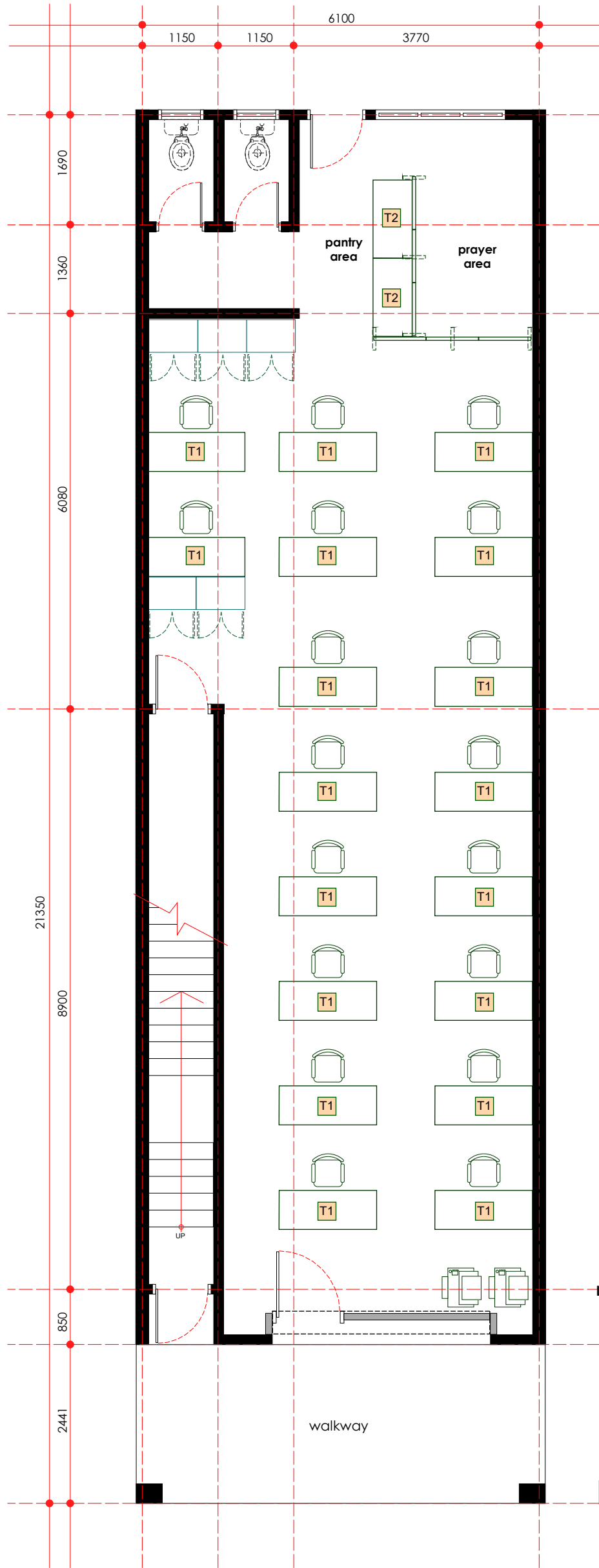
furniture layout plan - ground floor scale 1: 75
