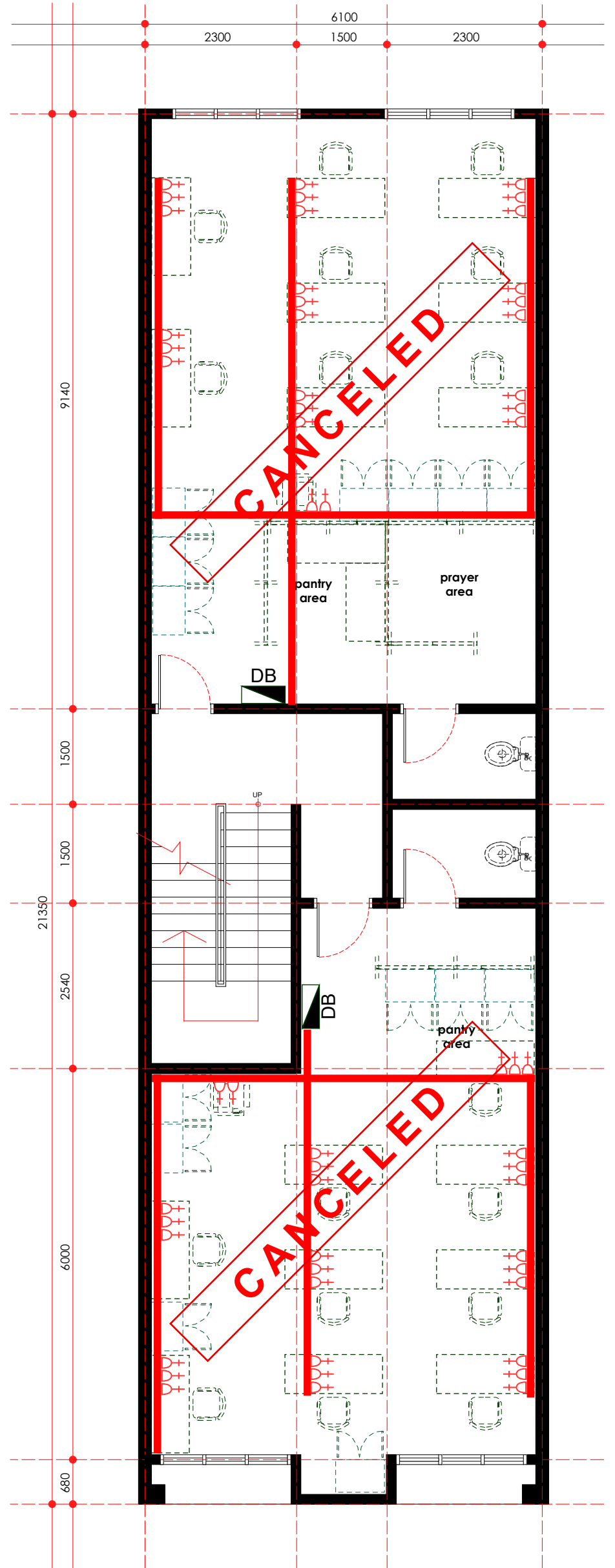
cabling route & point layout plan - second floor scale 1: 75
