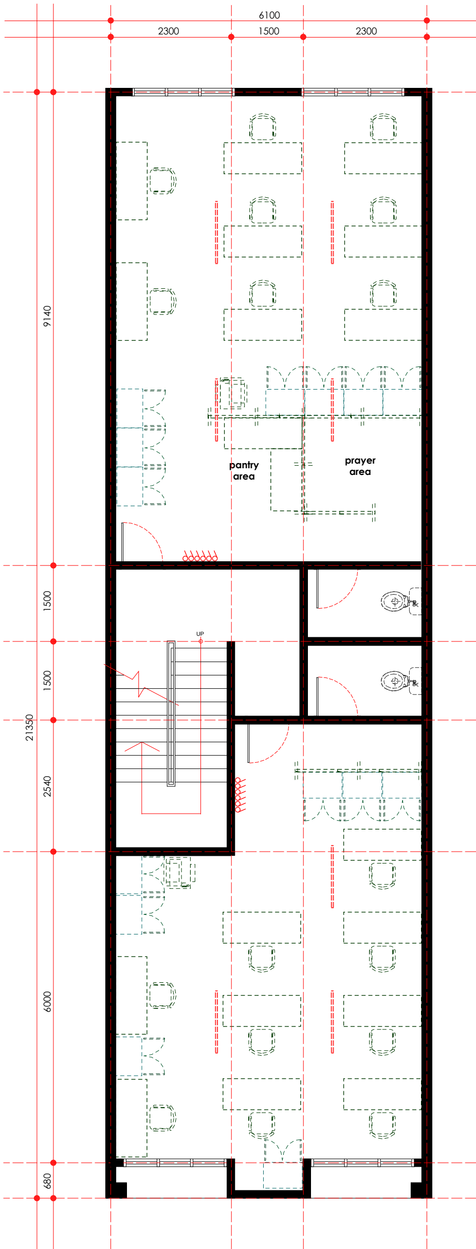
electrical point layout plan - first floor scale 1: 75
