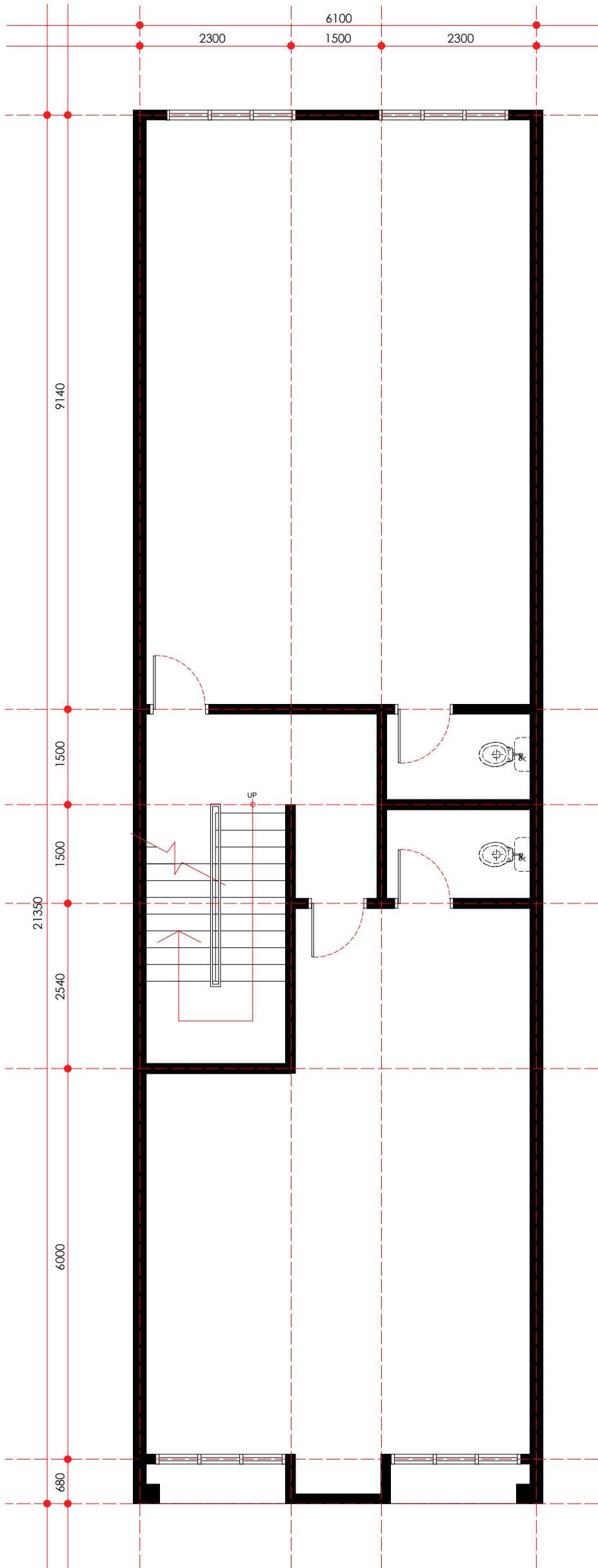
existing layout plan - first floor scale 1: 75
