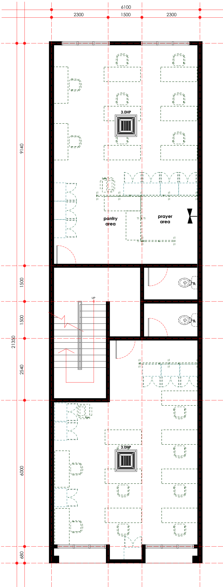
mechanical point layout plan - first floor scale 1: 75
