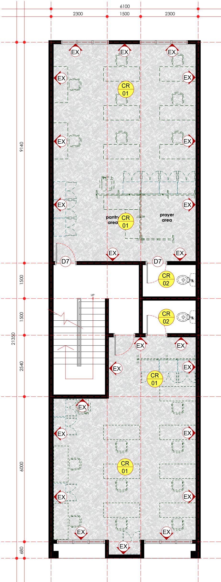
finishing layout plan - first floor scale 1: 75
