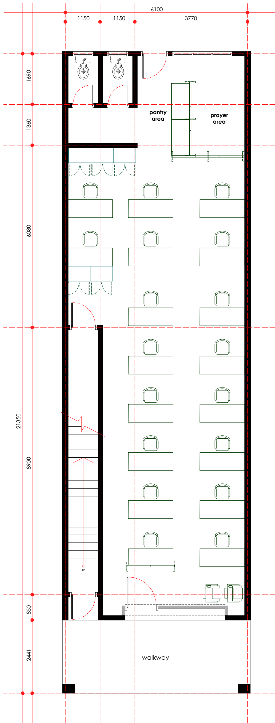
proposed layout plan - ground floor scale 1: 75
