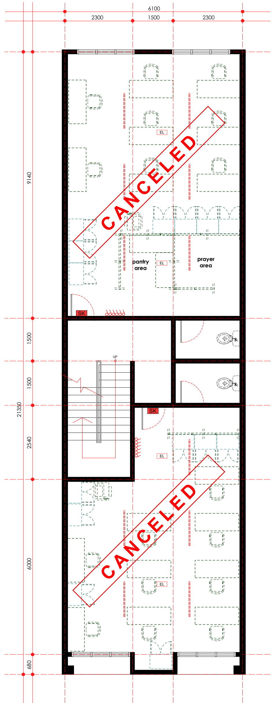
electrical point layout plan - second floor scale 1: 75
