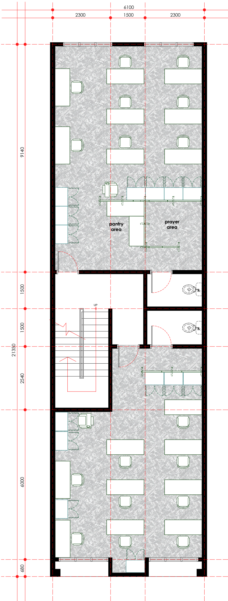
proposed layout plan - first floor scale 1: 75
