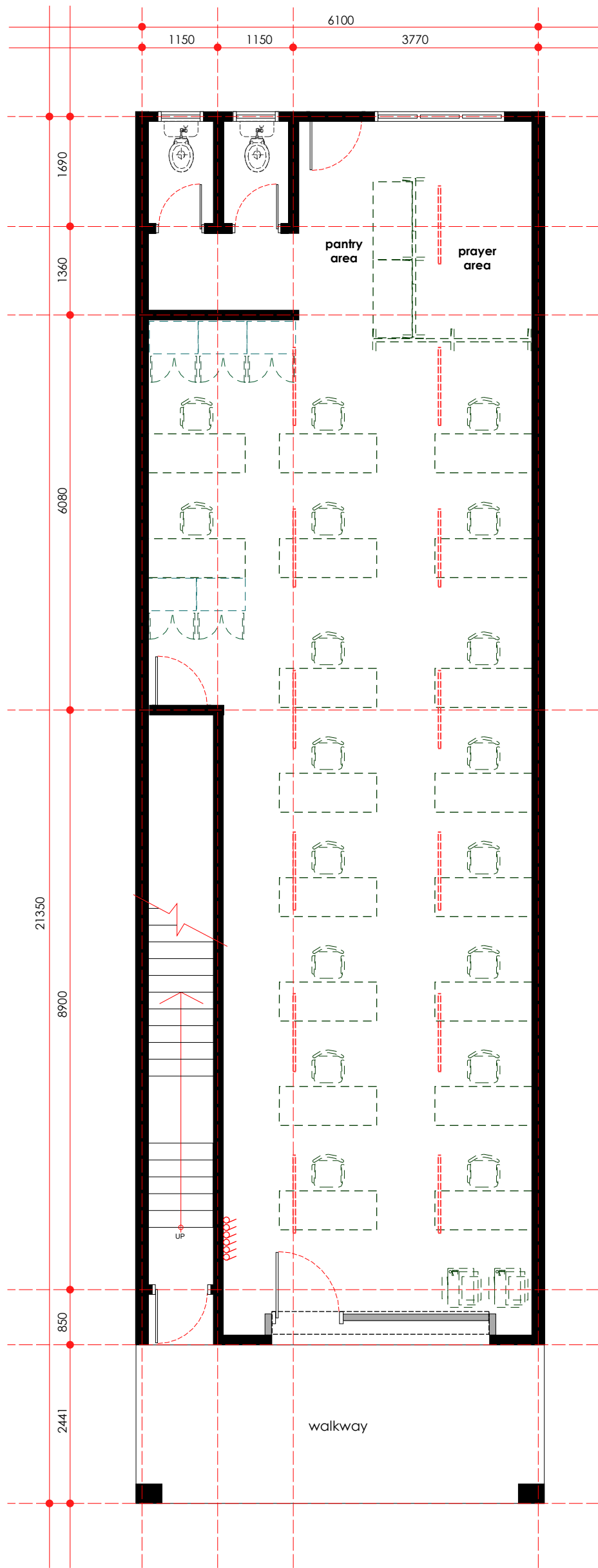
electrical point layout plan - ground floor scale 1: 75
