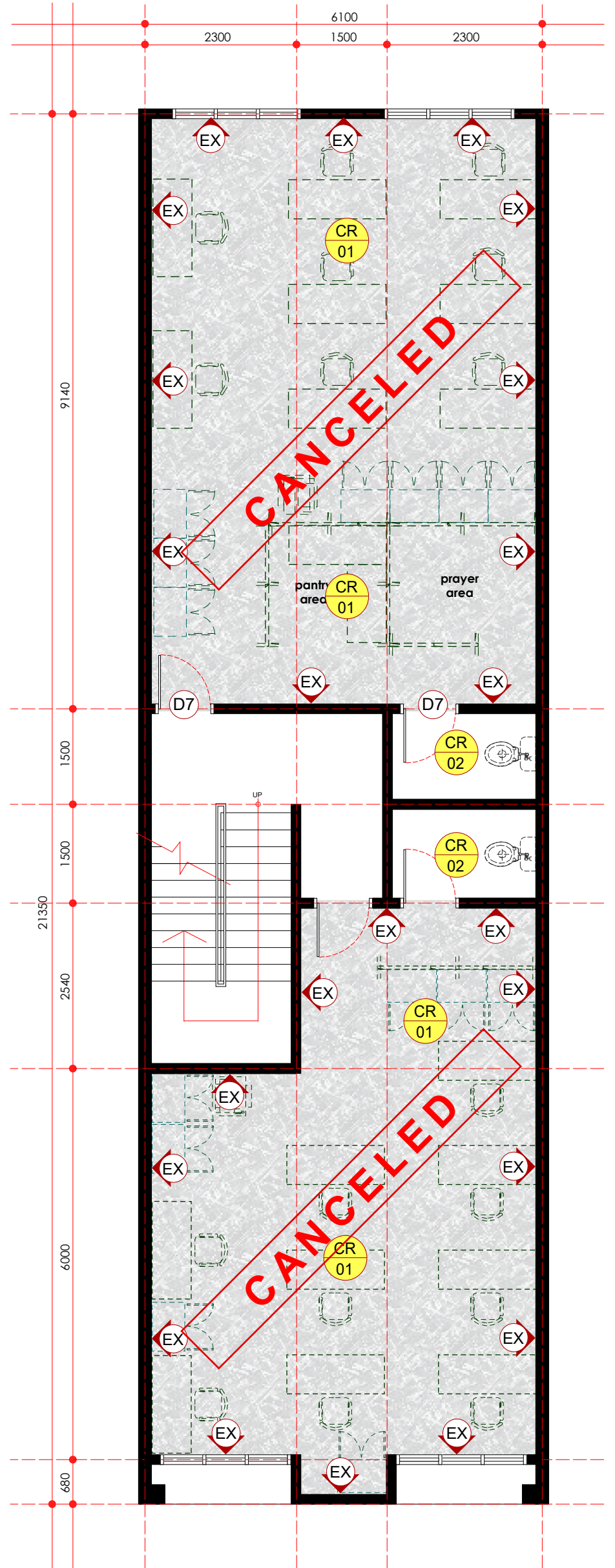
finishing layout plan - second floor scale 1: 75
