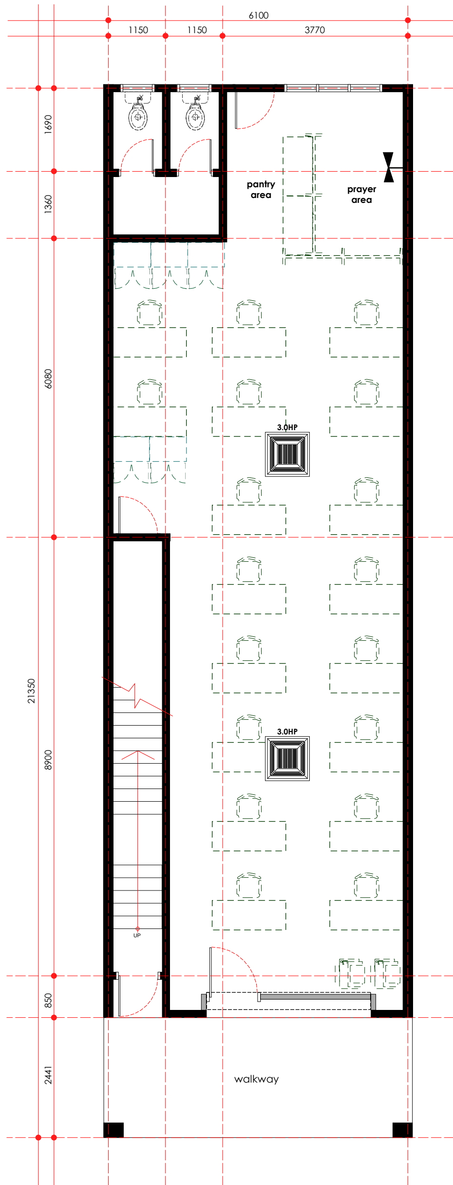
mechanical point layout plan - ground floor scale 1: 75
