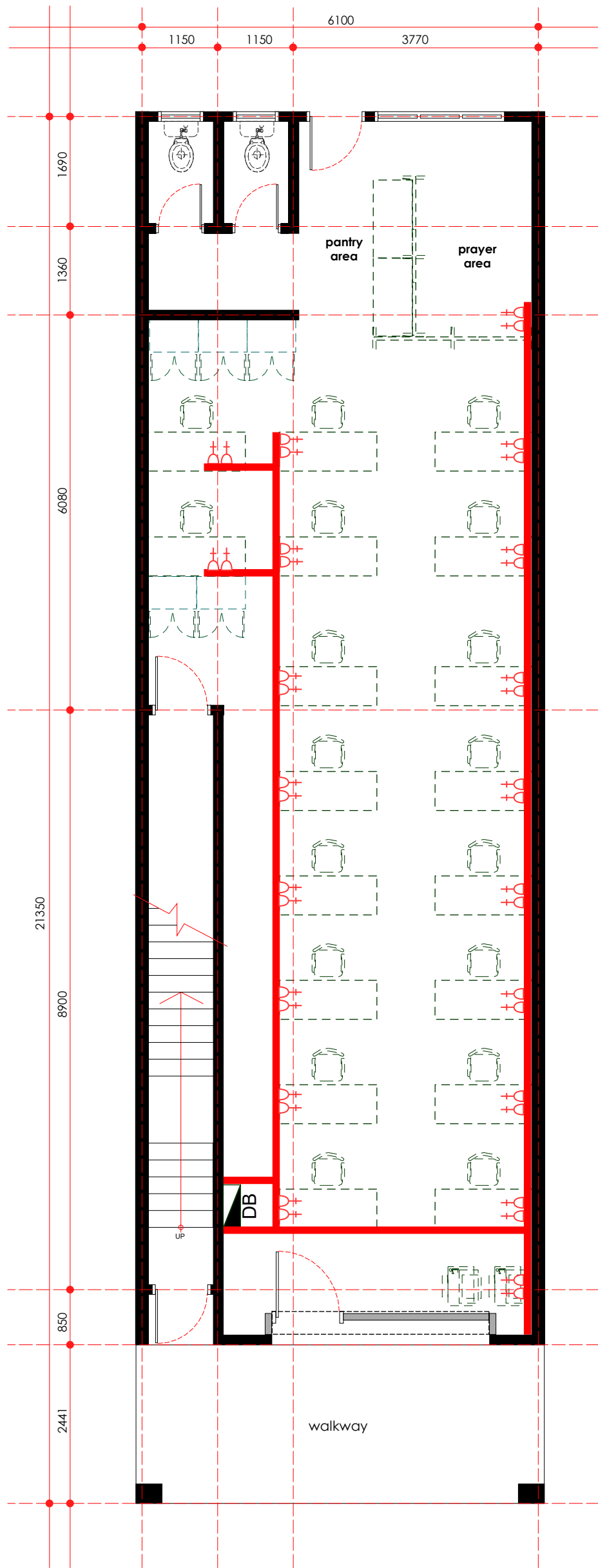
cabling route & point layout plan - ground floor scale 1: 75
