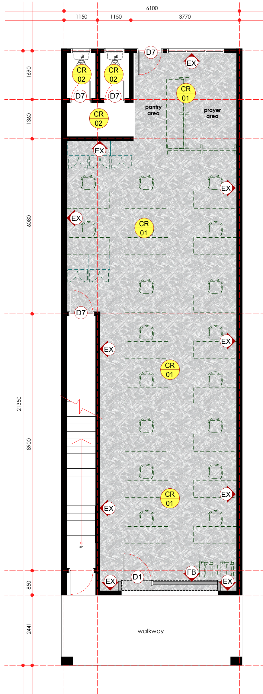
finishing layout plan - ground floor scale 1: 75
