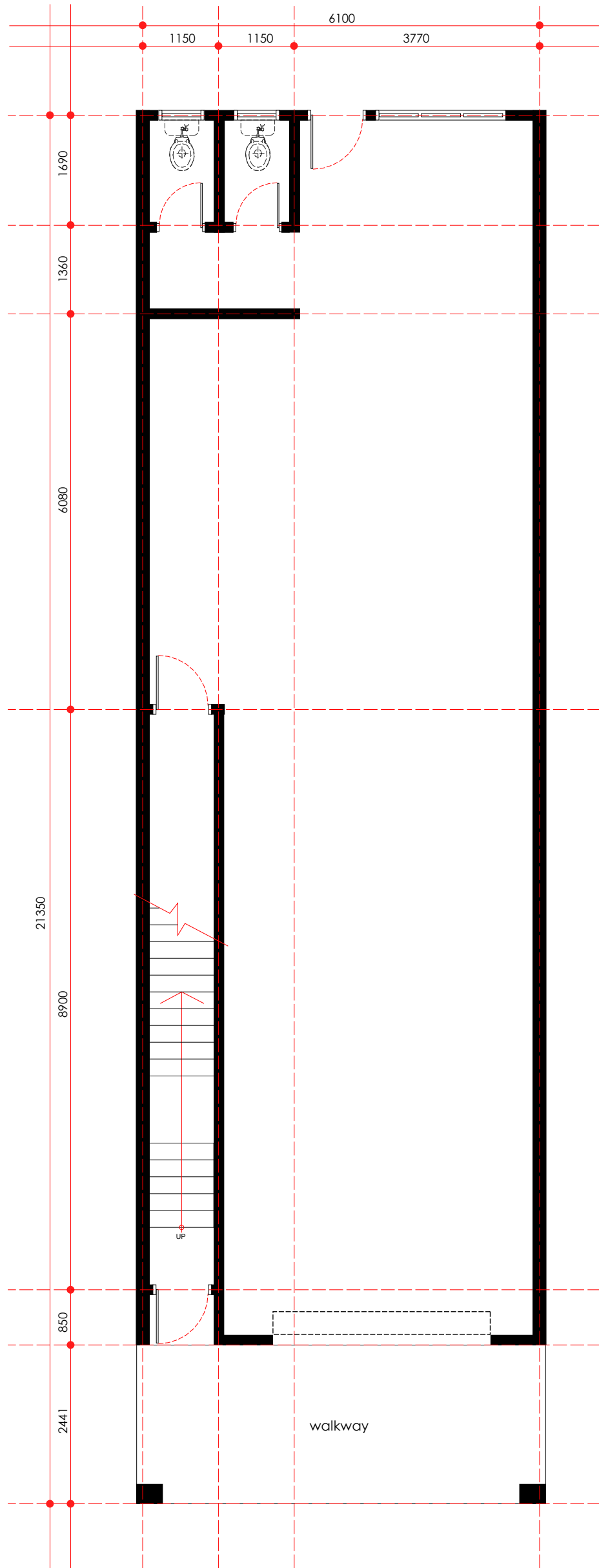
existing layout plan - ground floor scale 1: 75
