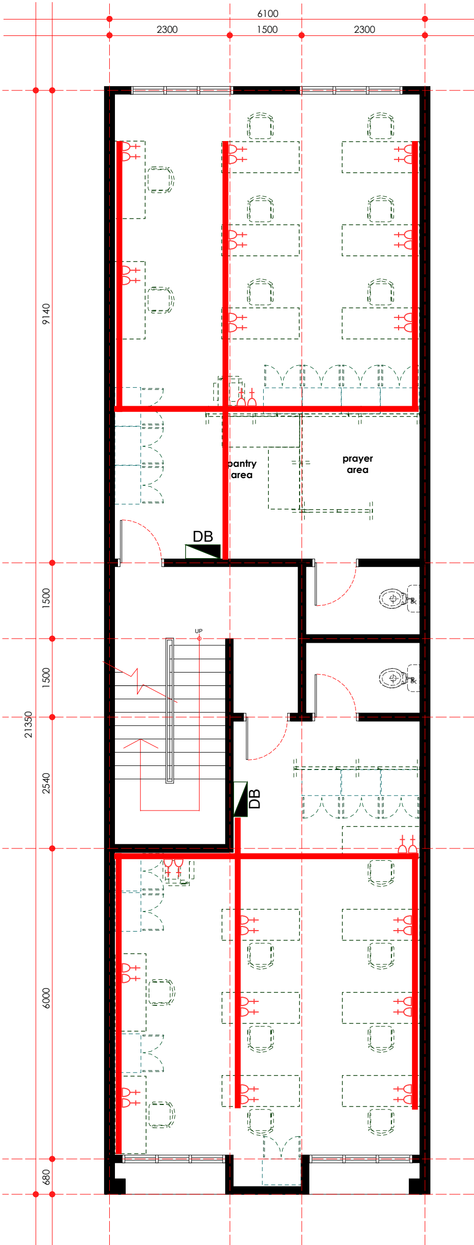
cabling route & point layout plan - first floor scale 1: 75
