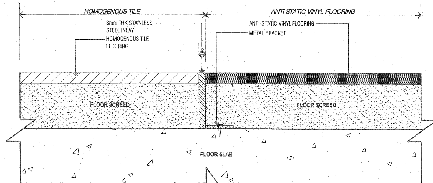
TYPICAL FLOOR DETAIL FD 03
