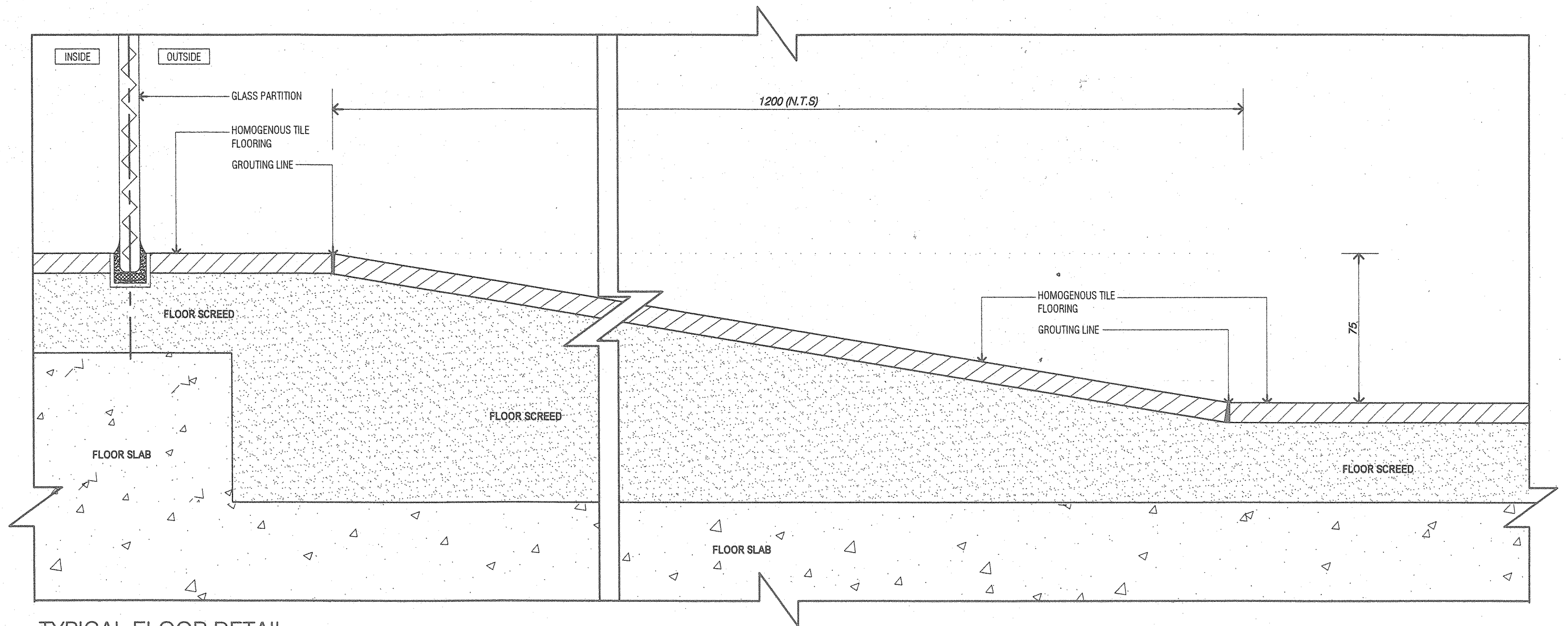
TYPICAL FLOOR DETAIL FD 05
