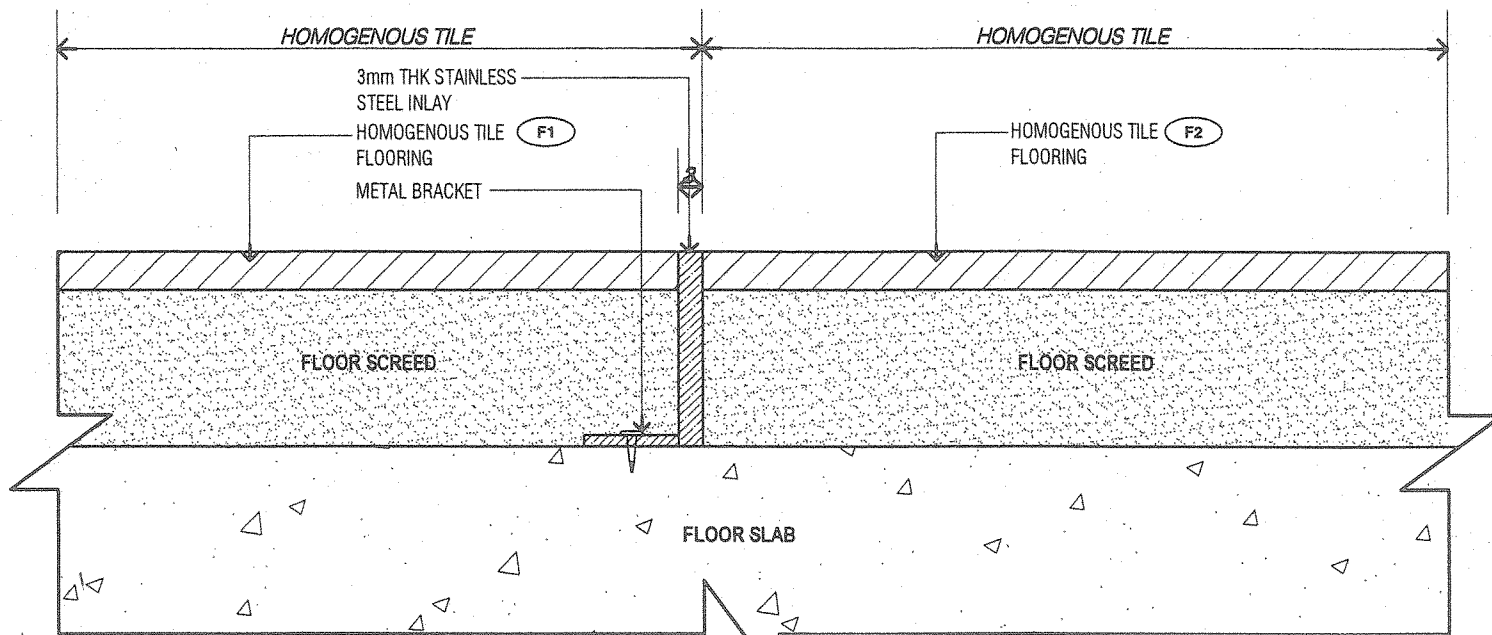
TYPICAL FLOOR DETAIL FD 02
