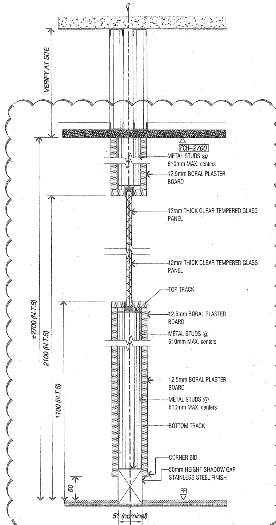
1F - NORMAL PARTITION + GLASS PARTITION SCALE 1/5
