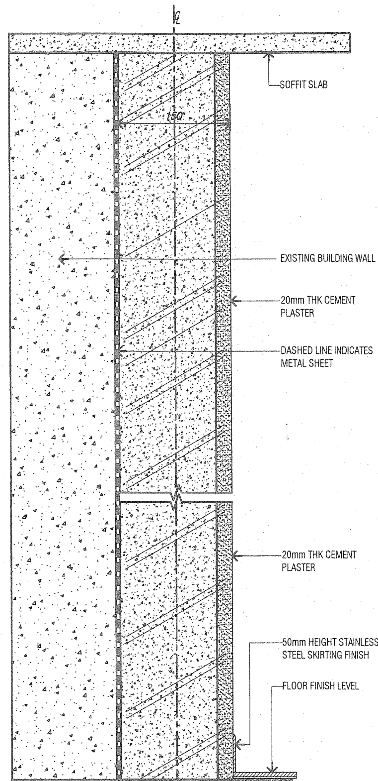
3A- BRICK WALL W/ METAL SHEET CLAD SCALE 1/5
