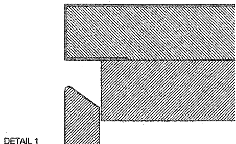
DETAIL 1 TYPICAL WORKTOP DETAIL FOR JOINERY IN STAINLESS STEEL OR LAMINATE EDGING OR VENEER FINISH
