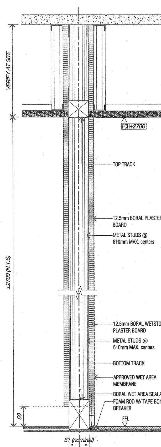
1C - WET RESISTANT PARTITION SCALE 1/5
