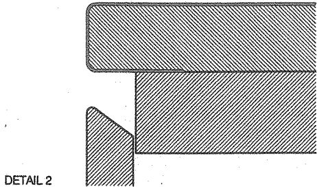
DETAIL 2 TYPICAL BENCHTOP DETAIL FOR JOINERY IN POSTFORMED LAMINATE FINISH
