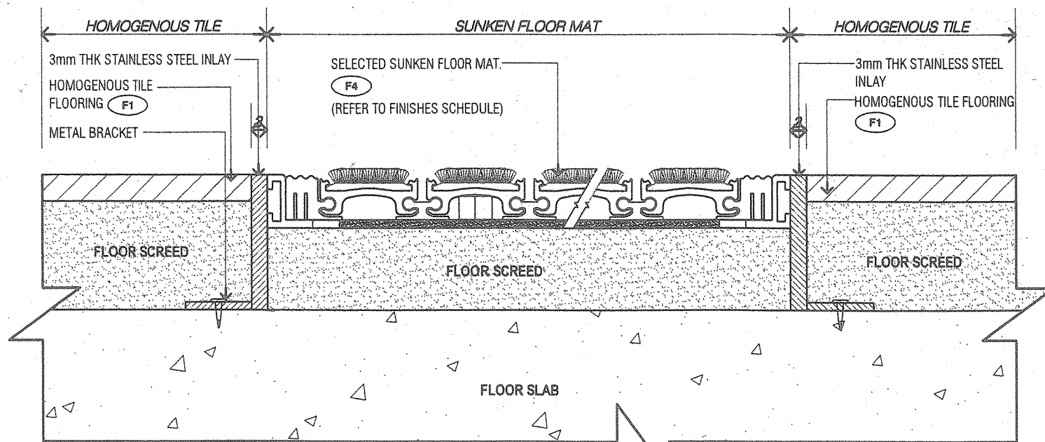
TYPICAL FLOOR DETAIL FD 01
