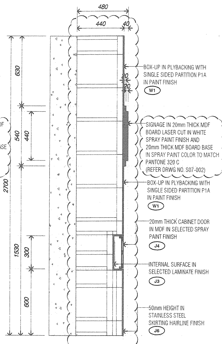
BF3 SECTION B SCALE 1/20
