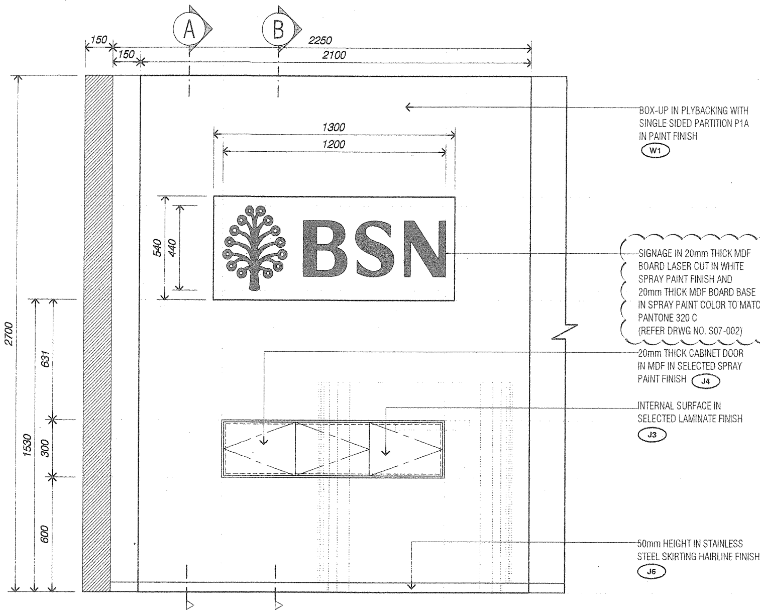
BF3 ELEVATION 1 SCALE 1/20
