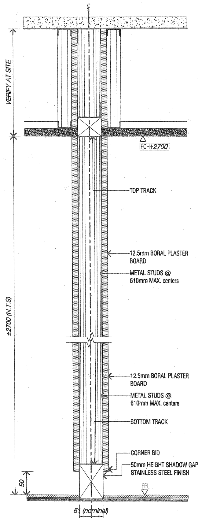
1 - NORMAL PARTITION SCALE 1/5
