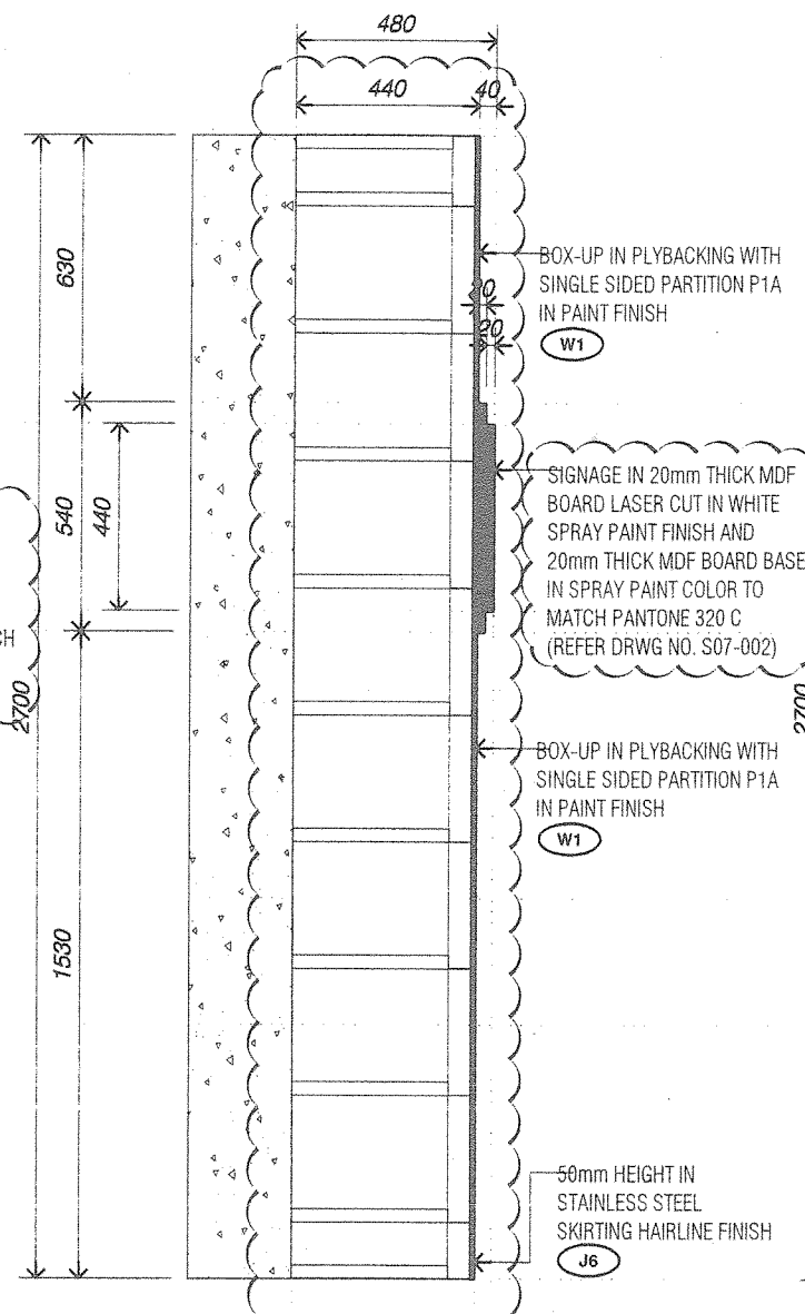
BF3 SECTION A SCALE 1/20
