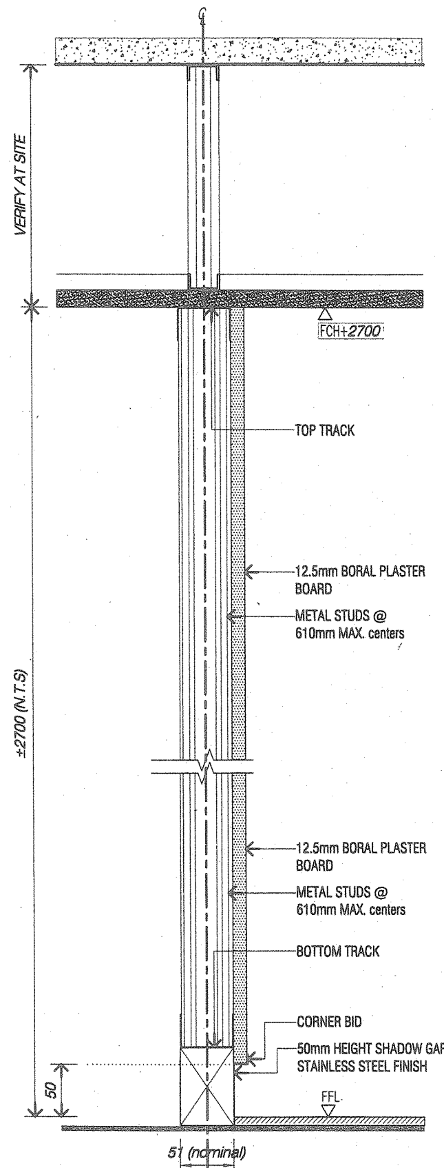
1A - SINGLE SIDED PARTITION SCALE 1/5
