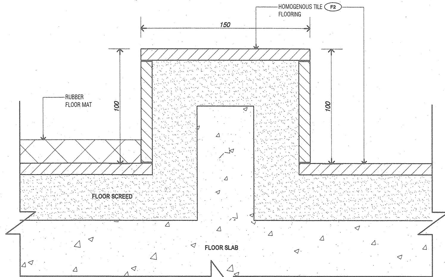
TYPICAL FLOOR DETAIL FD 04
