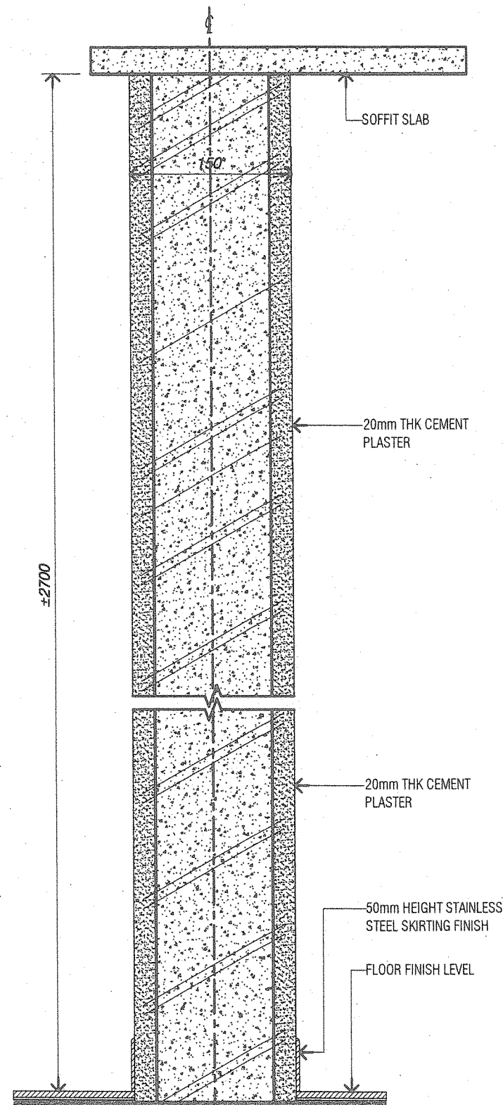
3- BRICK WALL SCALE 1/5
